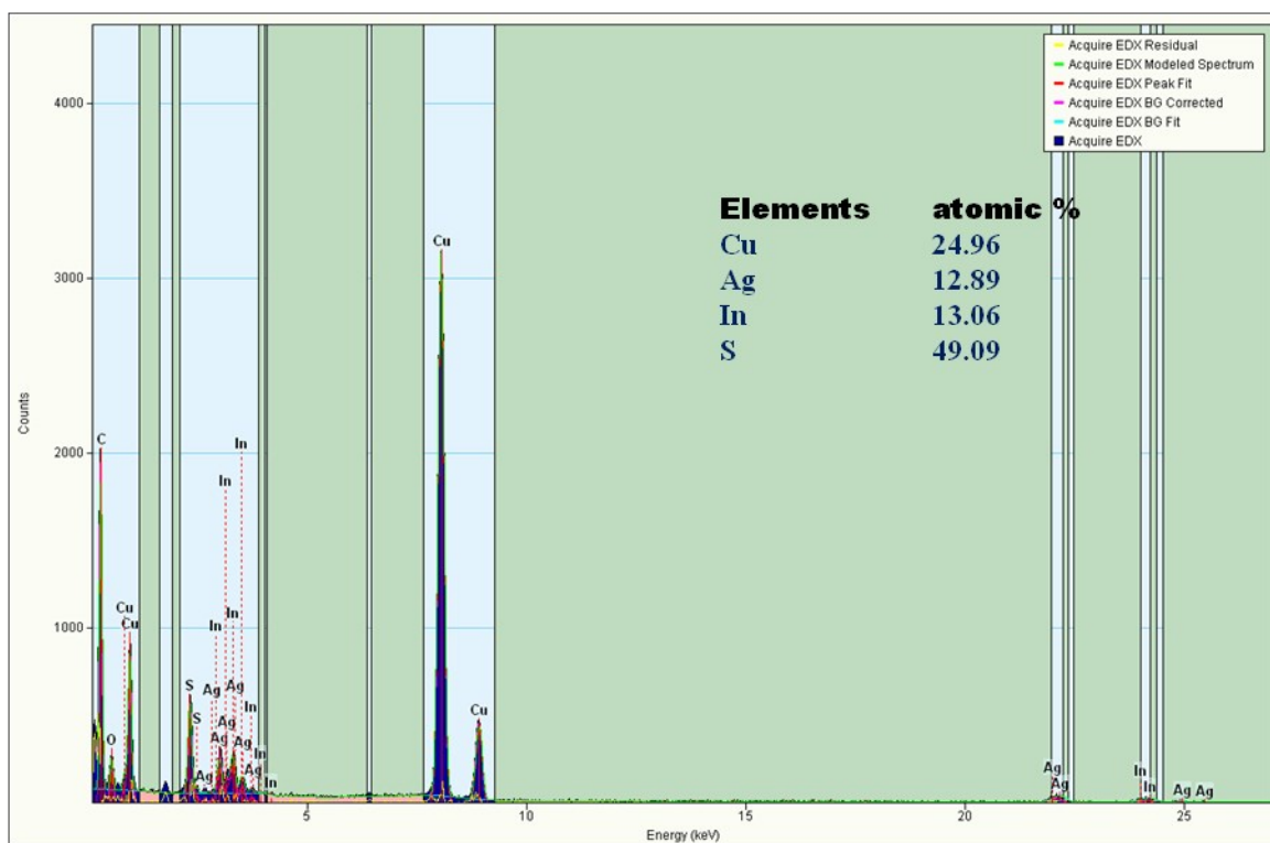
Fig. S1 EDX spectrum of CAIS QDs
