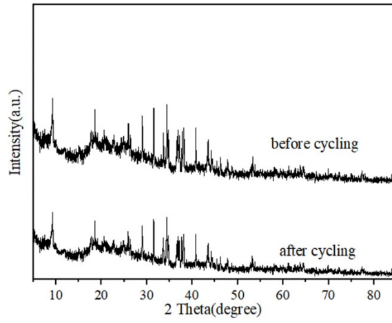
Figure S2. XRD pattern of the ASM-3 after the cycling tests for photocatalytic degradation of RhB.
