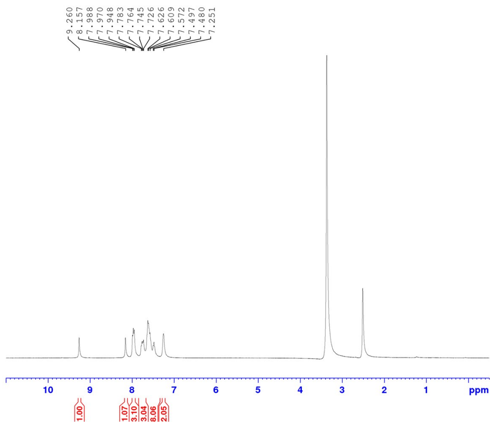
Fig. S5. 1 H NMR Spectrum of 2-(3-(4-fluorophenyl)-1-phenyl-1H-pyrazol-4-yl)-1H-phenanthro[9,10-d] imidazole (6c)
