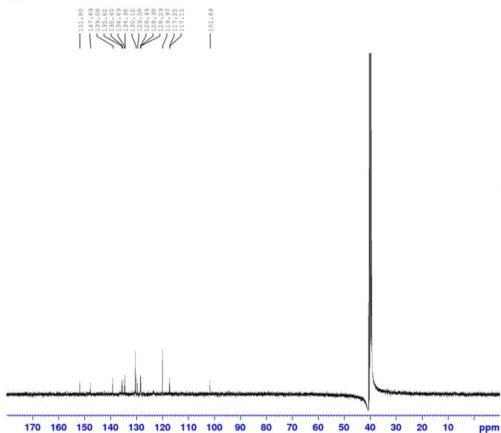
Fig. S4. 13 C NMR Spectrum of 2-(3-(4-chlorophenyl)-1-phenyl-1H-pyrazol-4-yl)-1H-phenanthro[9,10-d] imidazole (6b)
