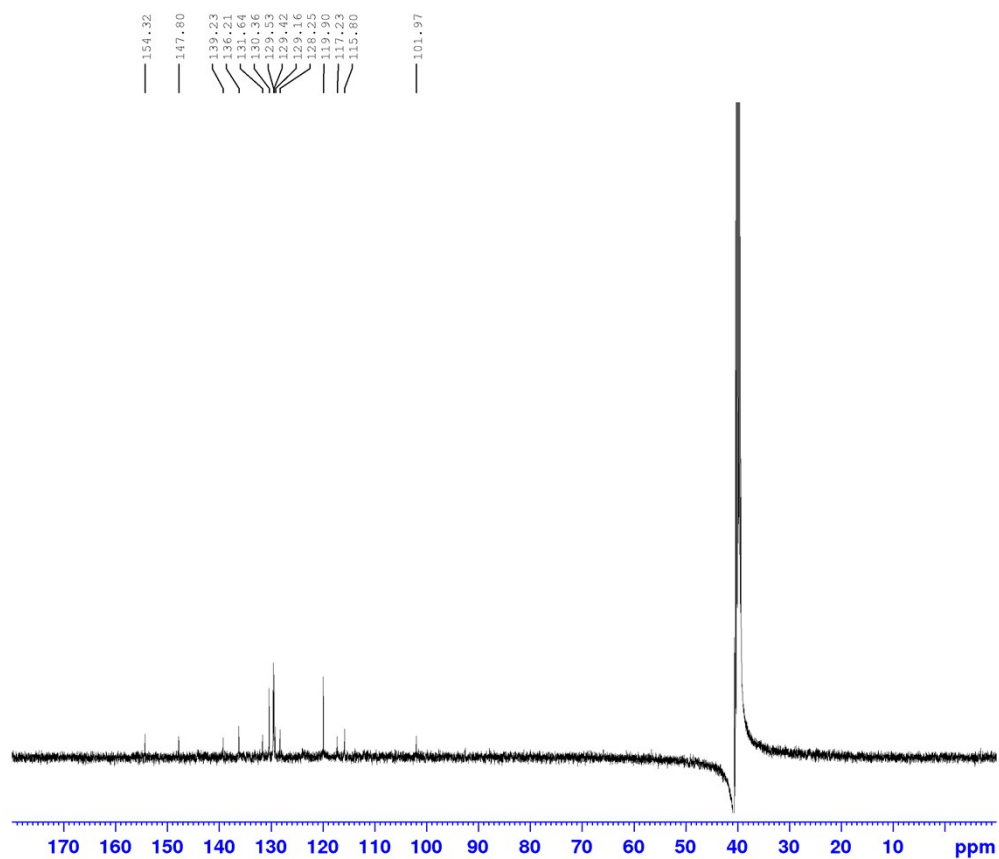
Fig. S20. ^{13}\text{C} NMR Spectrum of 2-(3-(4-nitrophenyl)-1-phenyl-1H-pyrazol-4-yl)-1H-phenanthro[9,10-d]imidazole (6j)
