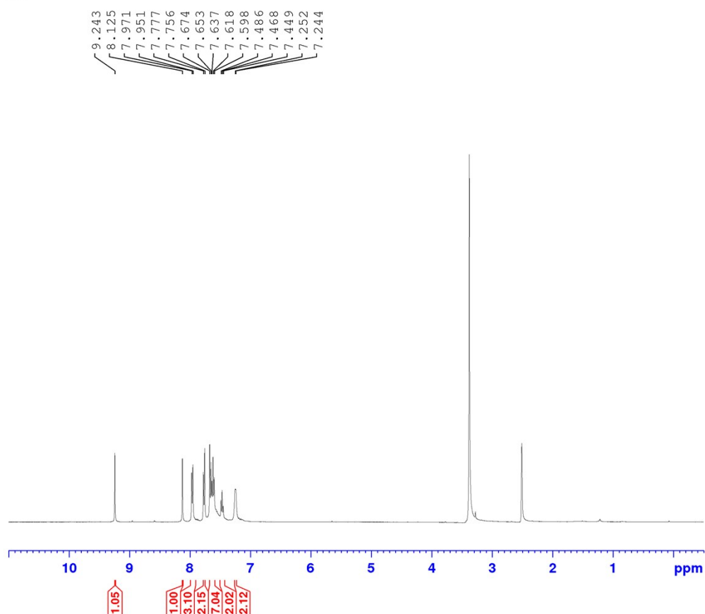
Fig. S9. ^1\text{H} NMR Spectrum of 2-(3-(3-fluorophenyl)-1-phenyl-1H-pyrazol-4-yl)-1H-phenanthro[9,10-d]imidazole (6e)
