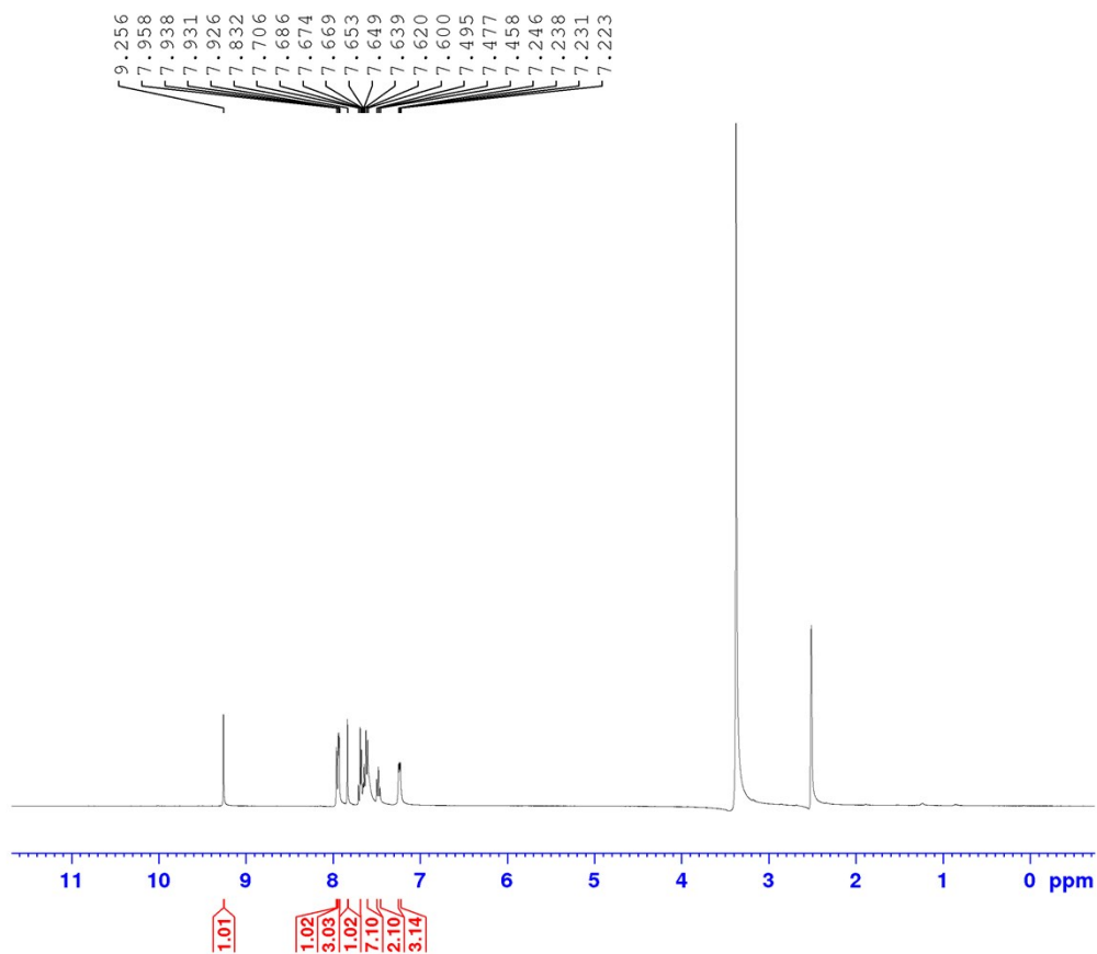
Fig. S3. 1 H NMR Spectrum of 2-(3-(4-chlorophenyl)-1-phenyl-1H-pyrazol-4-yl)-1H-phenanthro[9,10-d] imidazole (6b)
