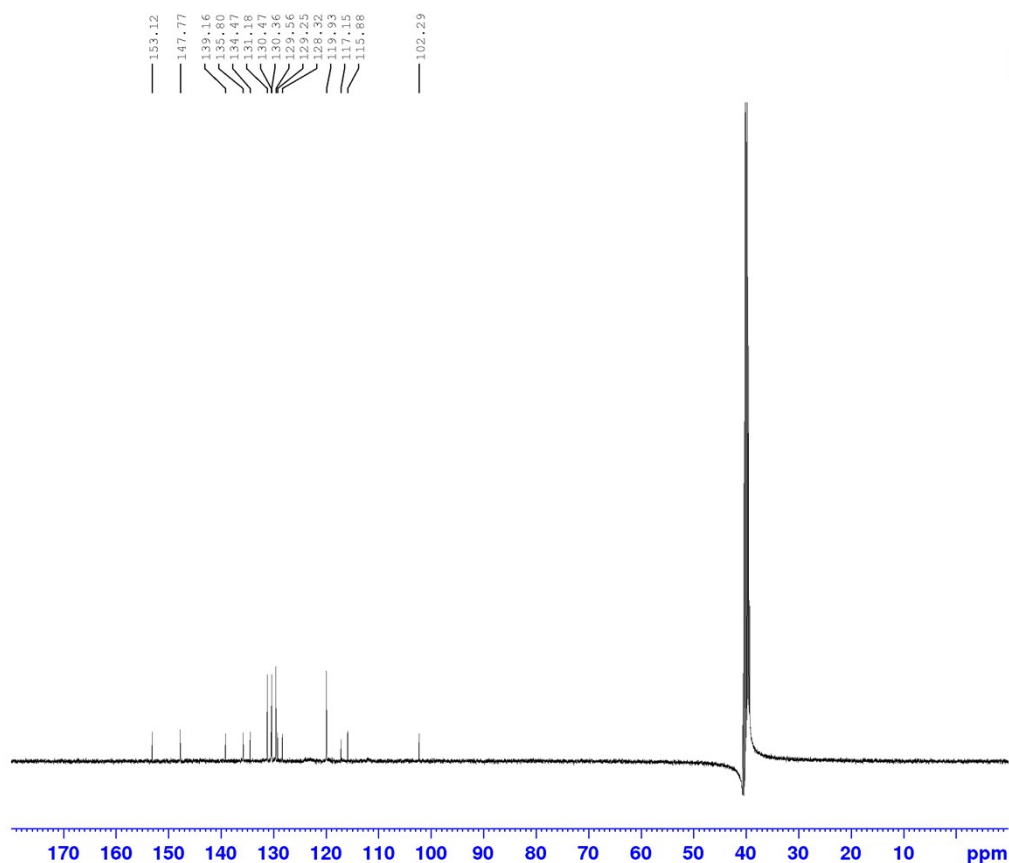
Fig. S10. 13 C NMR Spectrum of 2-(3-(3-fluorophenyl)-1-phenyl-1H-pyrazol-4-yl)-1H-phenanthro[9,10-d]imidazole (6e)
