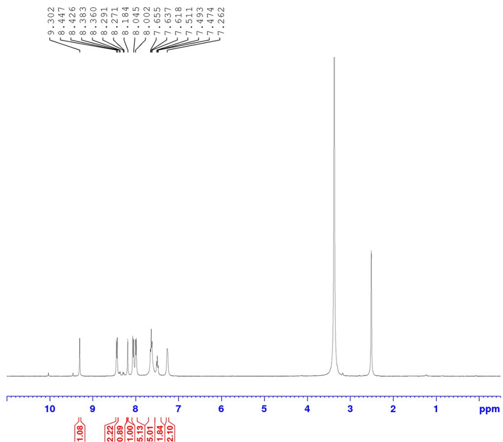
Fig. S1. 1 H NMR Spectrum of 2-(1,3-diphenyl-1H-pyrazol-4-yl)-1H-phenanthro[9,10-d]imidazole (6a)
