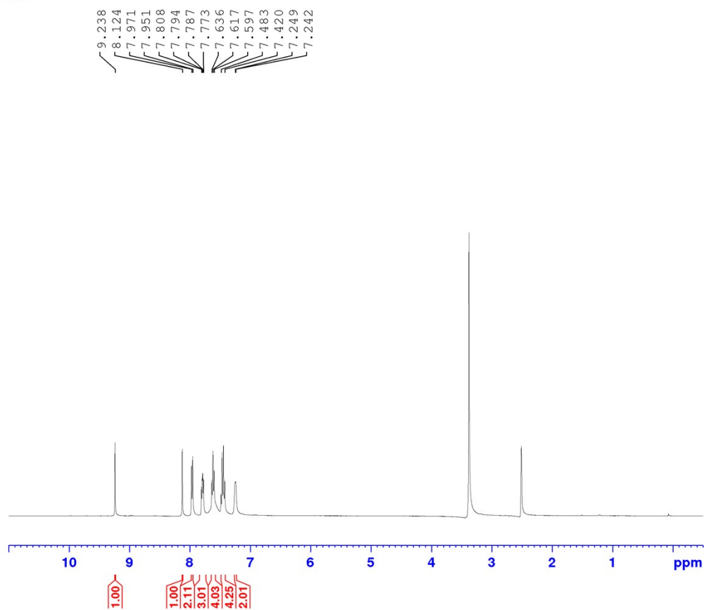
Fig. S15. 1 H NMR Spectrum of 2-(3-(2,4-dichlorophenyl)-1-phenyl-1H-pyrazol-4-yl)-1H-phenanthro[9,10-d]imidazole (6h)
