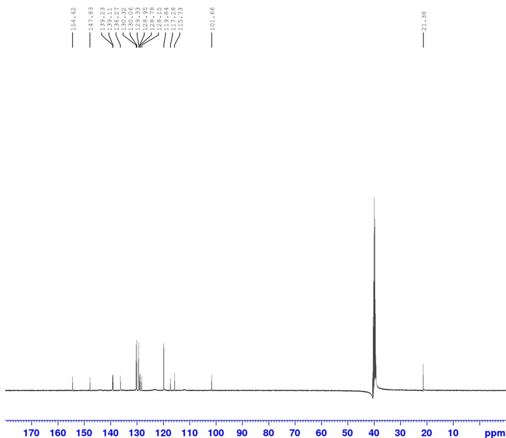
Fig. S12. ^{13}\text{C} NMR Spectrum of 2-(1-phenyl-3-(p-tolyl)-1H-pyrazol-4-yl)-1H-phenanthro[9,10-d]imidazole (6f)
