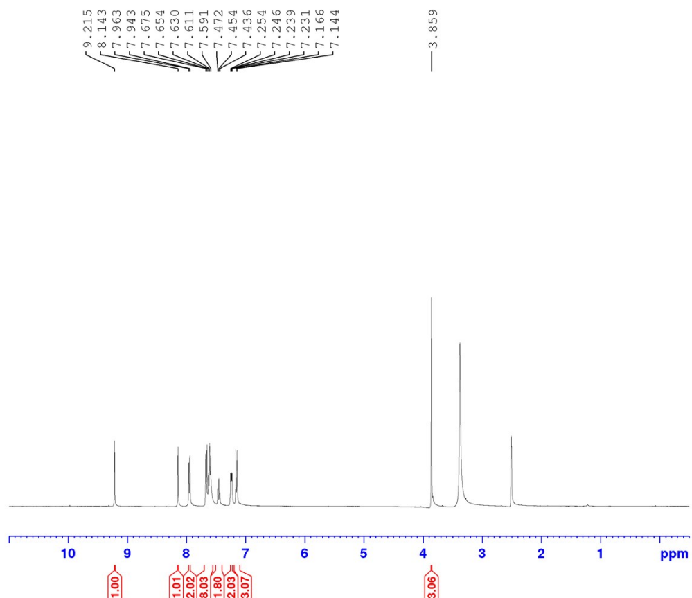
Fig. S17. ^1\text{H} NMR Spectrum of 2-(3-(4-methoxyphenyl)-1-phenyl-1H-pyrazol-4-yl)-1H-phenanthro[9,10-d]imidazole (6i)
