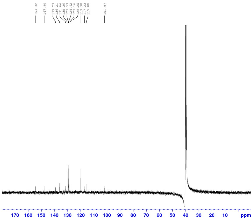
Fig. S2. 13 C NMR Spectrum of 2-(1,3-diphenyl-1H-pyrazol-4-yl)-1H-phenanthro[9,10-d]imidazole (6a)
