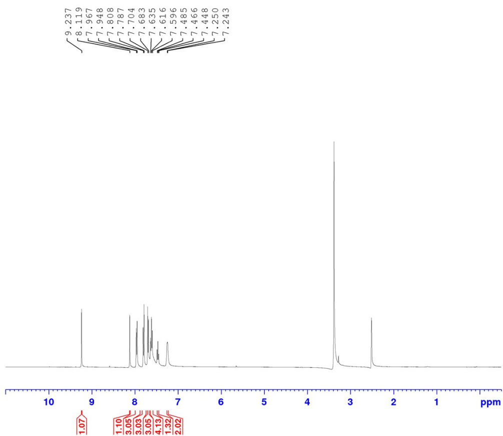
Fig. S7. ^1\text{H} NMR Spectrum of 2-(3-(4-bromophenyl)-1-phenyl-1H-pyrazol-4-yl)-1H-phenanthro[9,10-d] imidazole (6d)
