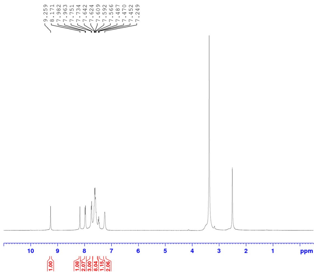
Fig. S19. ^1\text{H} NMR Spectrum of 2-(3-(4-nitrophenyl)-1-phenyl-1H-pyrazol-4-yl)-1H-phenanthro[9,10-d]imidazole (6j)
