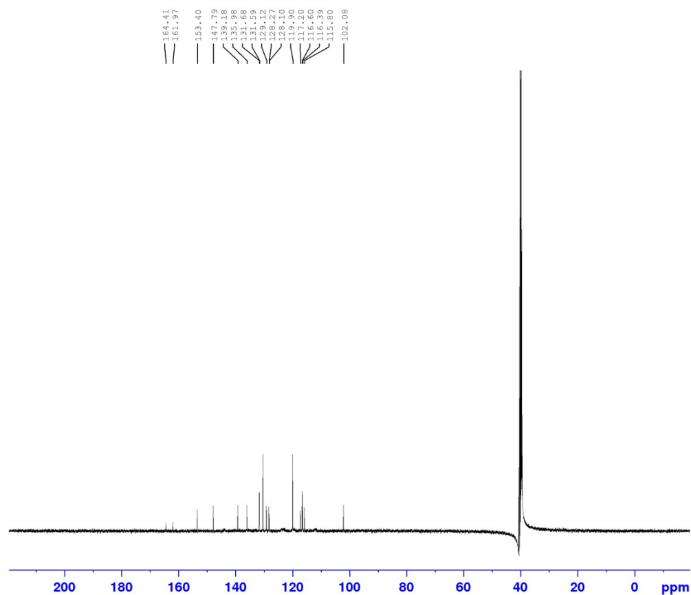
Fig. S16. 13 C NMR Spectrum of 2-(3-(2,4-dichlorophenyl)-1-phenyl-1H-pyrazol-4-yl)-1H-phenanthro[9,10-d]imidazole (6h)
