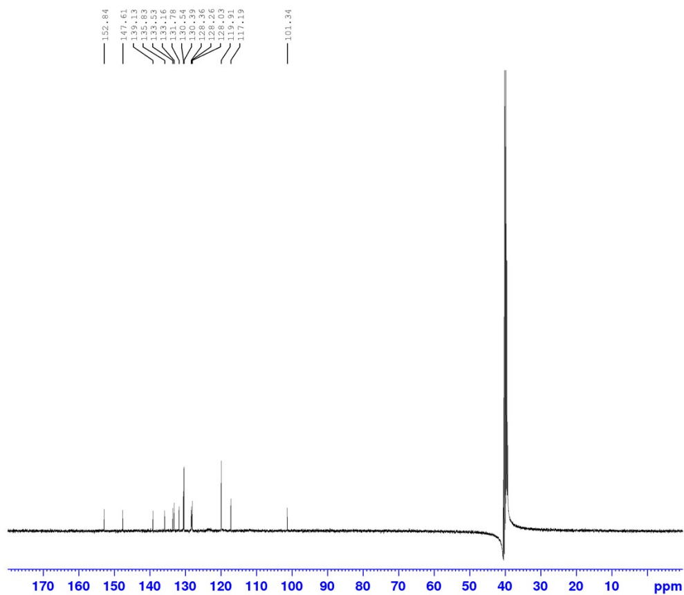
Fig. S14. ^{13}\text{C} NMR Spectrum of 2-(3-(2-chlorophenyl)-1-phenyl-1H-pyrazol-4-yl)-1H-phenanthro[9,10-d]imidazole (6g)
