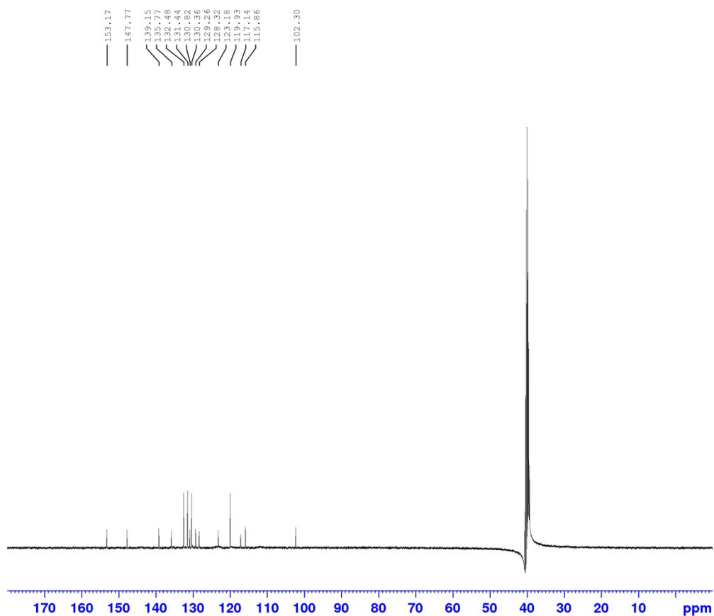
Fig. S8. ^{13}\text{C} NMR Spectrum of 2-(3-(4-bromophenyl)-1-phenyl-1H-pyrazol-4-yl)-1H-phenanthro[9,10-d]imidazole (6d)
