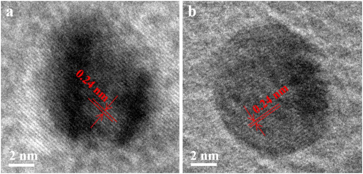
Fig. S1 HRTEM of Au/HT and 0.5Cu-Au/HT
