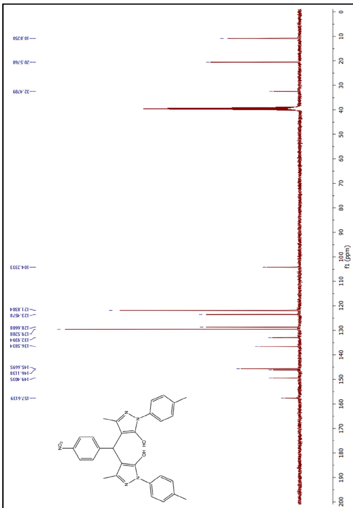
Figure 80. ^{13}\text{C} -NMR spectrum of compound (6be)
