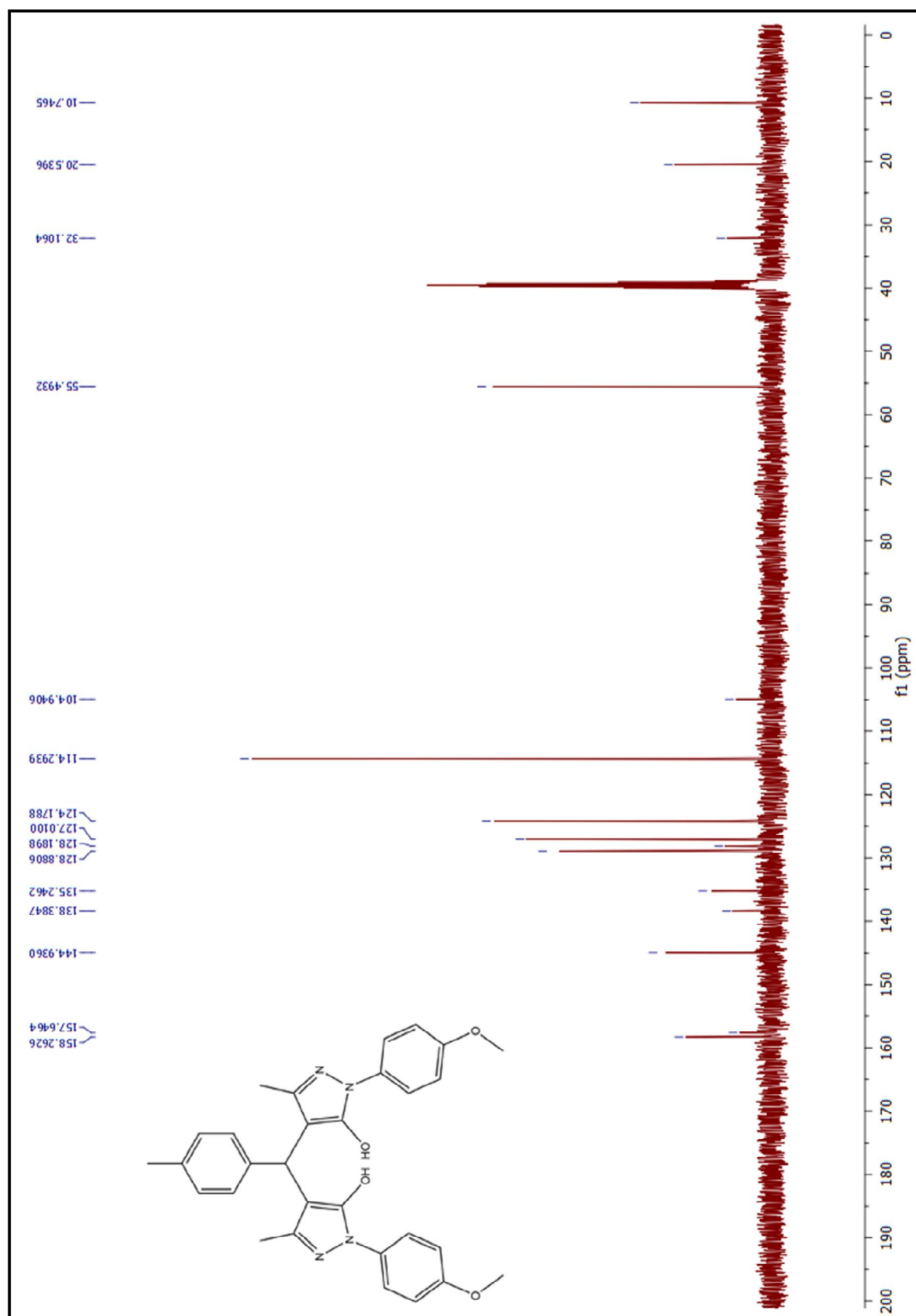
Figure 92. ^{13}\text{C} -NMR spectrum of compound (6bi)
