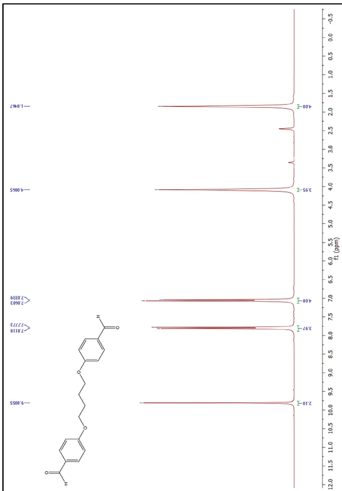
Figure 5. ^1\text{H} -NMR spectrum of compound (4b)
