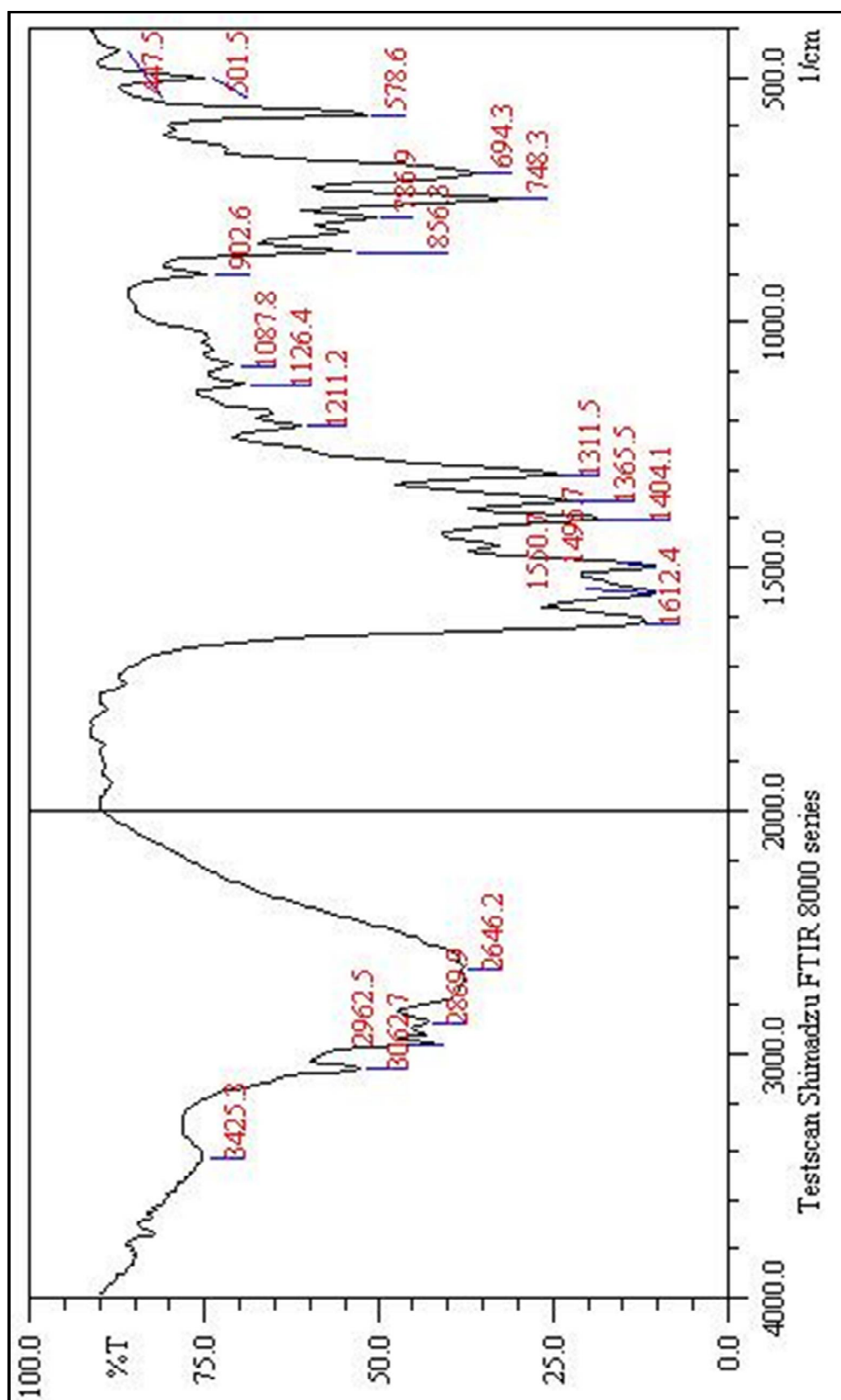
Figure 31. FT-IR spectrum of compound (6ak)
