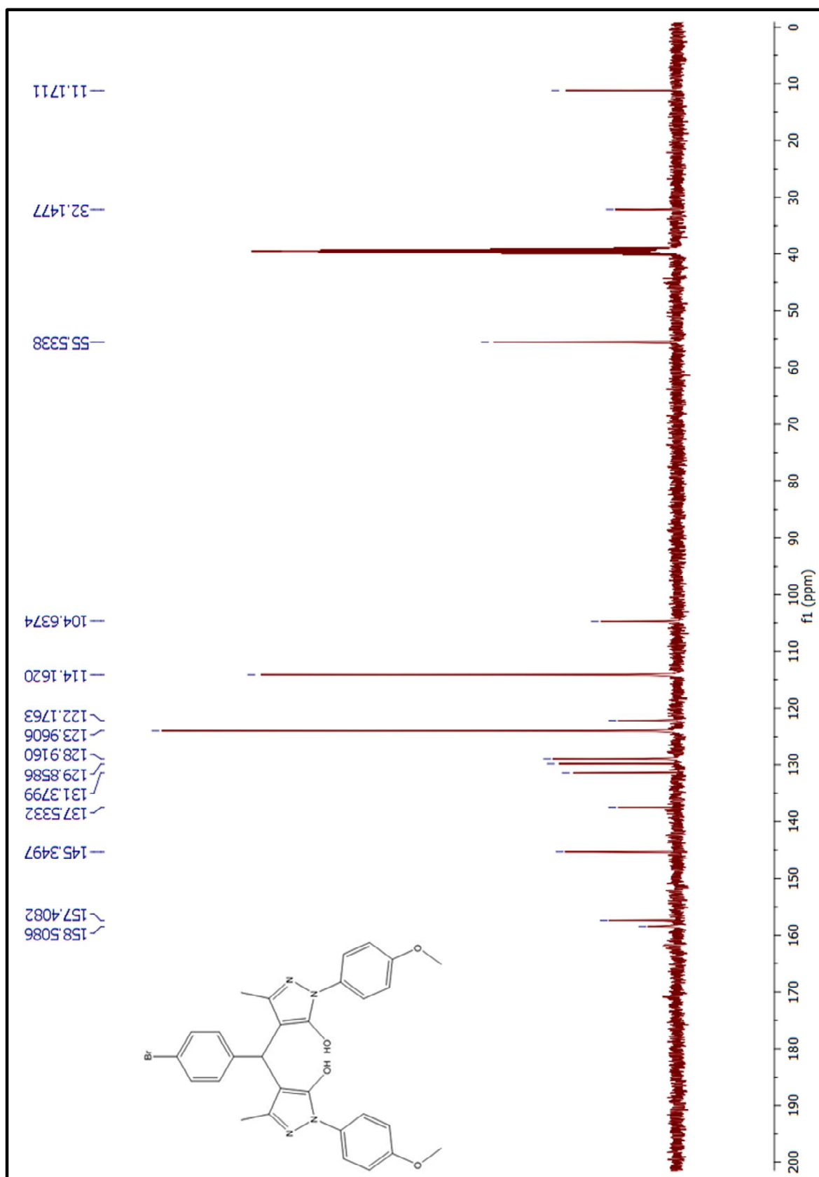
Figure 89. ^{13}\text{C} -NMR spectrum of compound (6bh)
