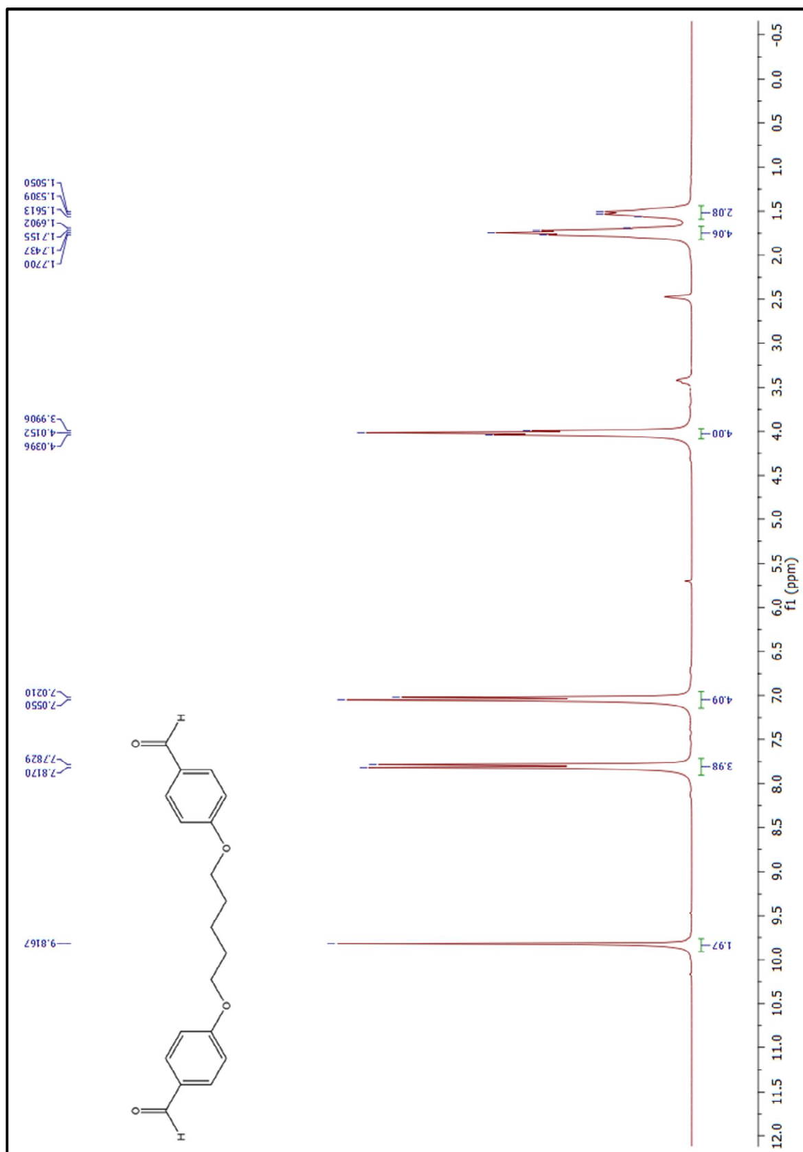
Figure 8. 1 H-NMR spectrum of compound (4c)
