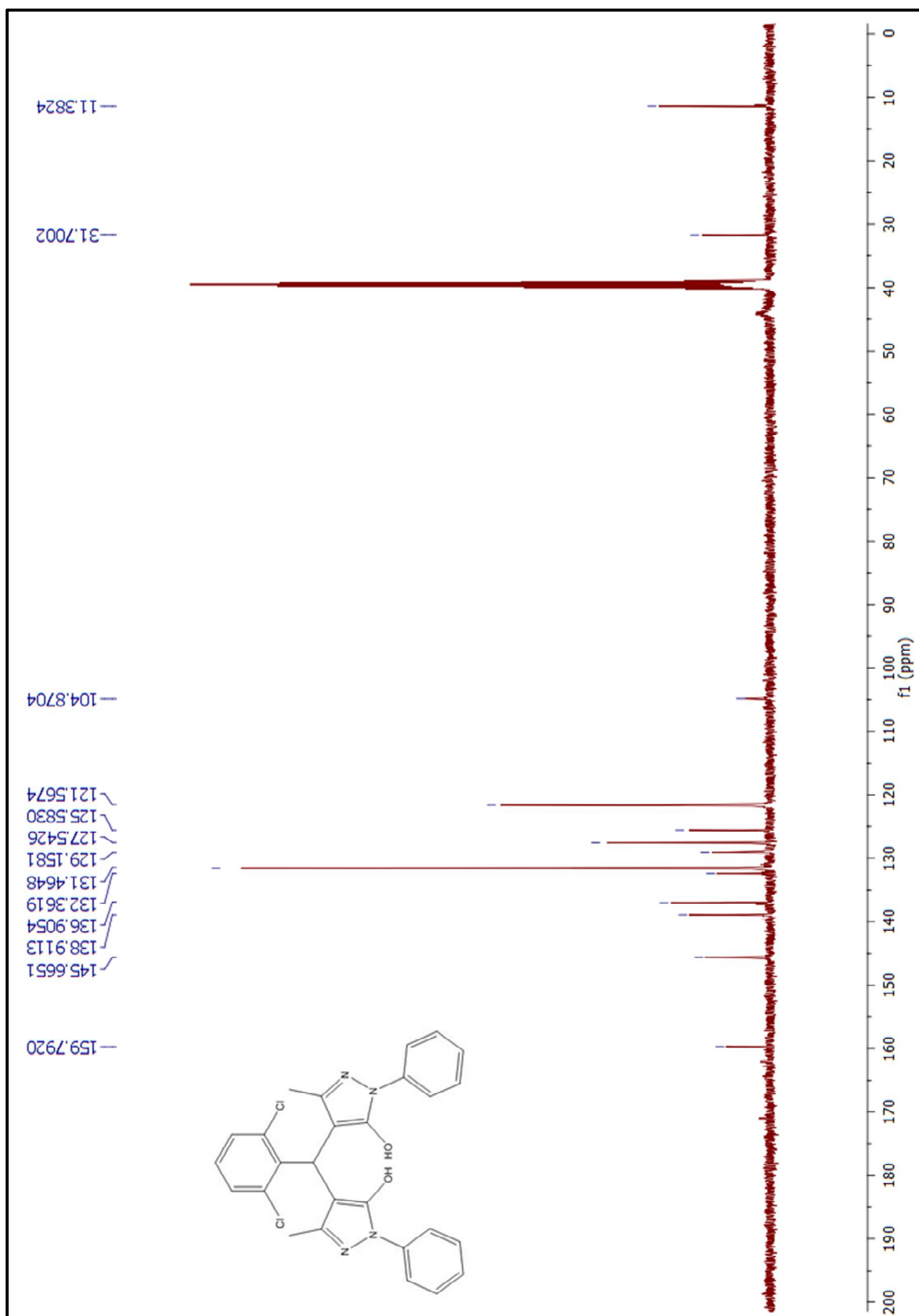
Figure 22. ^{13}\text{C} -NMR spectrum of compound (6af)
