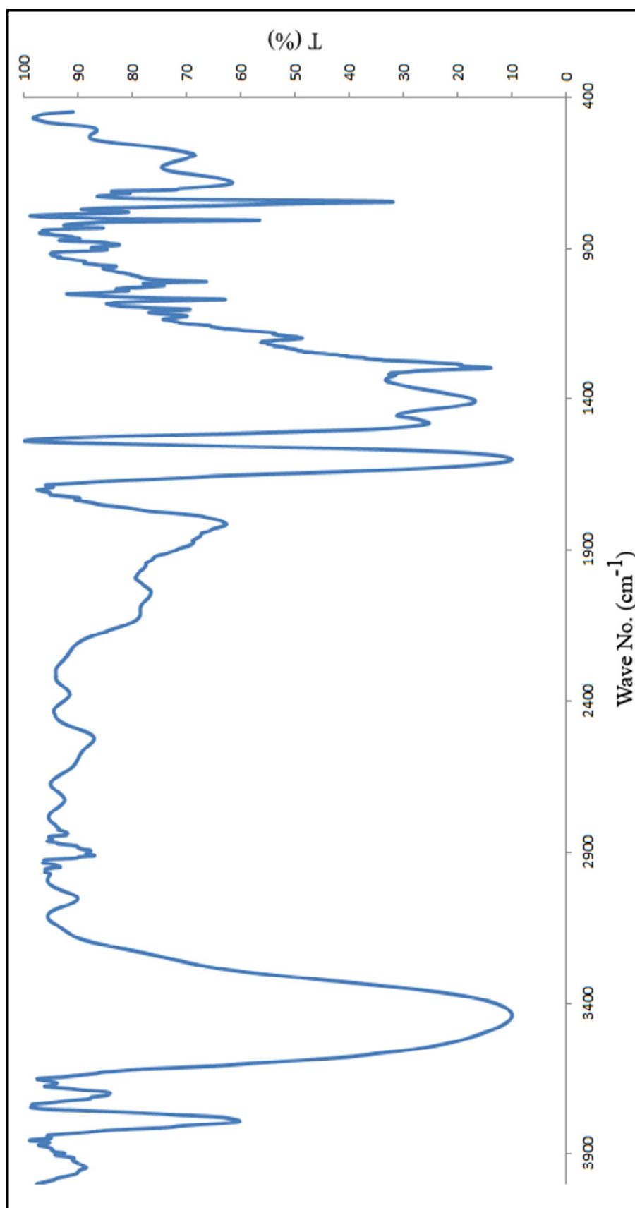
Figure 23. FT-IR spectrum of compound (6ag)
