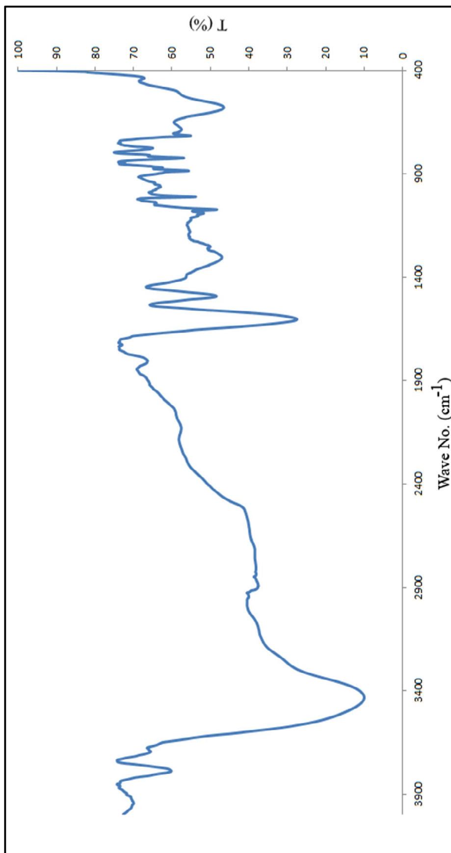
Figure 61. FT-IR spectrum of compound (6ay)
