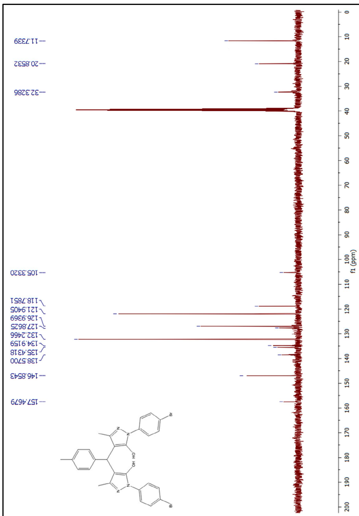
Figure 65. ^{13}\text{C} -NMR spectrum of compound (6az)
