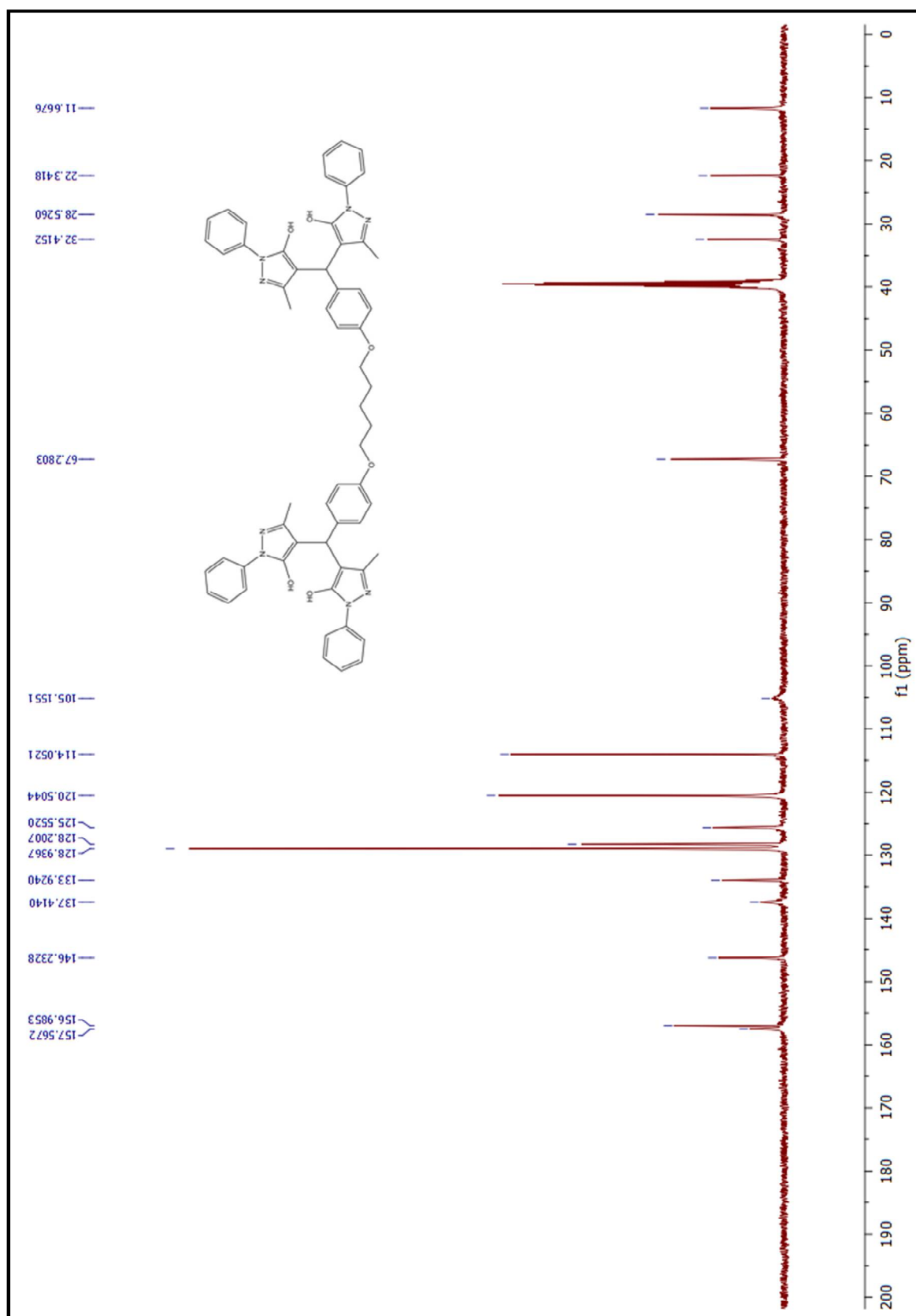
Figure 107. ^{13}\text{C} -NMR spectrum of compound (6bn)
