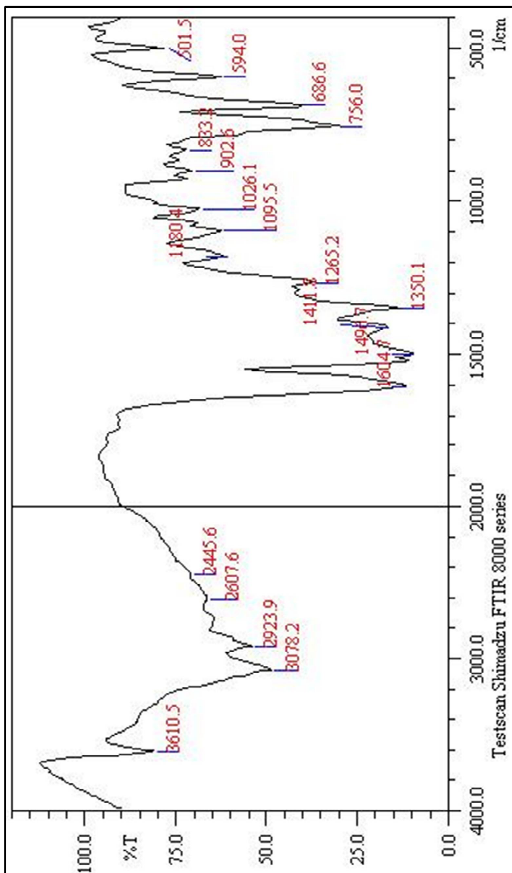
Figure 48. FT-IR spectrum of compound (6as)
