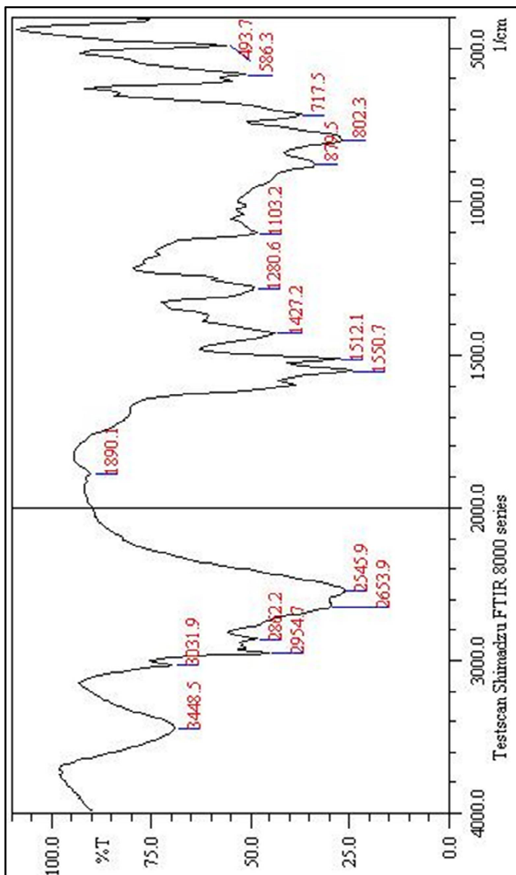
Figure 75. FT-IR spectrum of compound (6bd)
