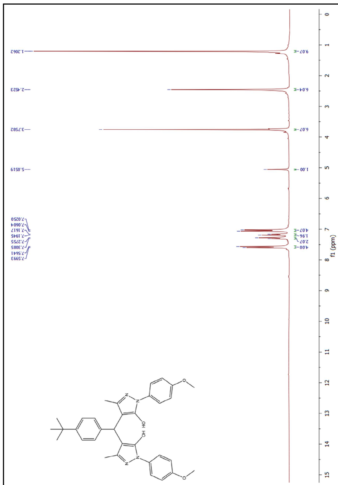
Figure 94. 1 H-NMR spectrum of compound (6bj)
