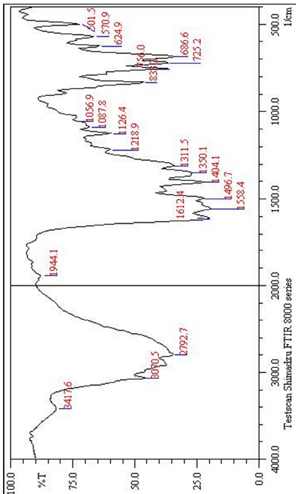
Figure 50. FT-IR spectrum of compound (6at)
