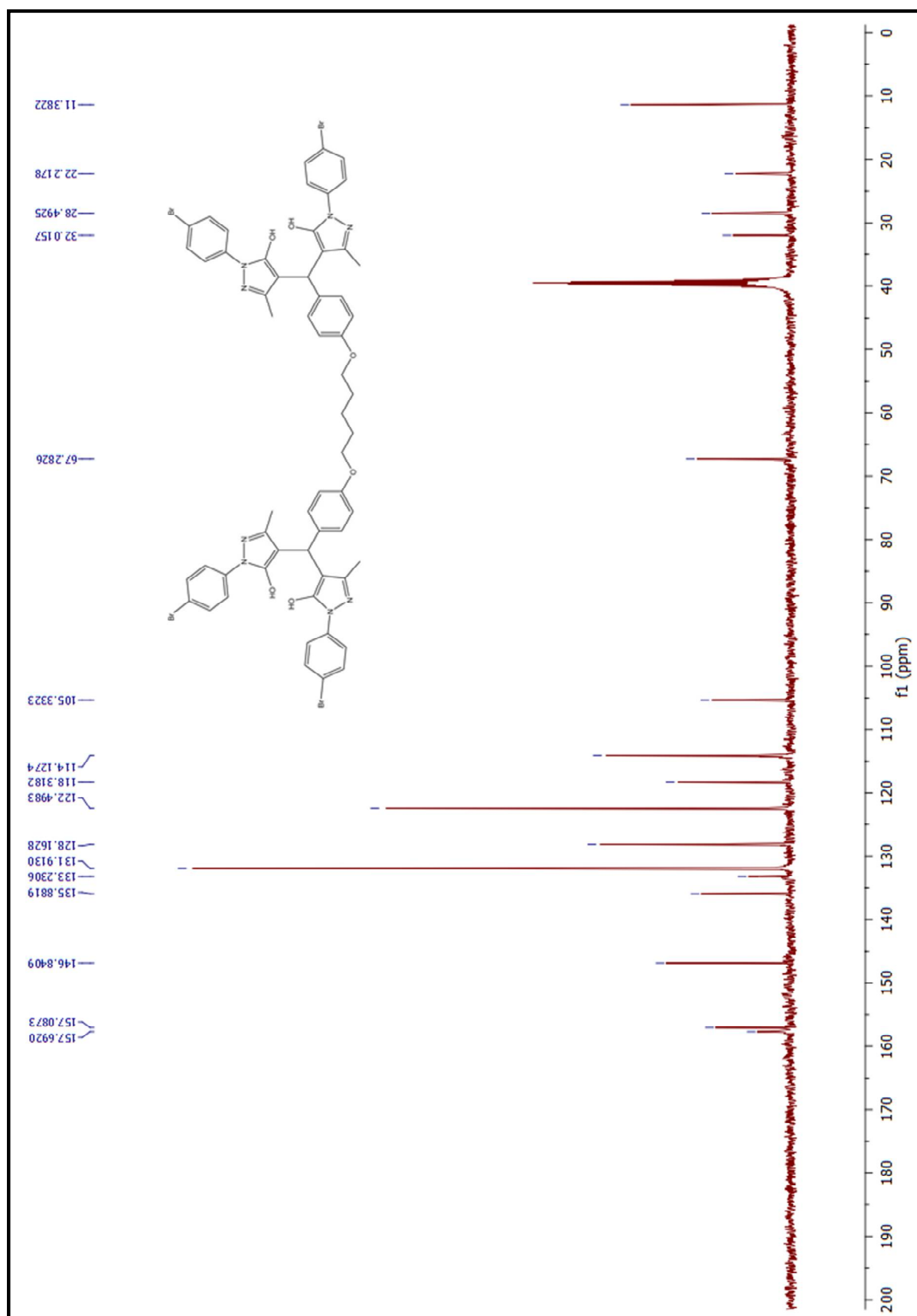
Figure 113. ^{13}\text{C} -NMR spectrum of compound (6bp)
