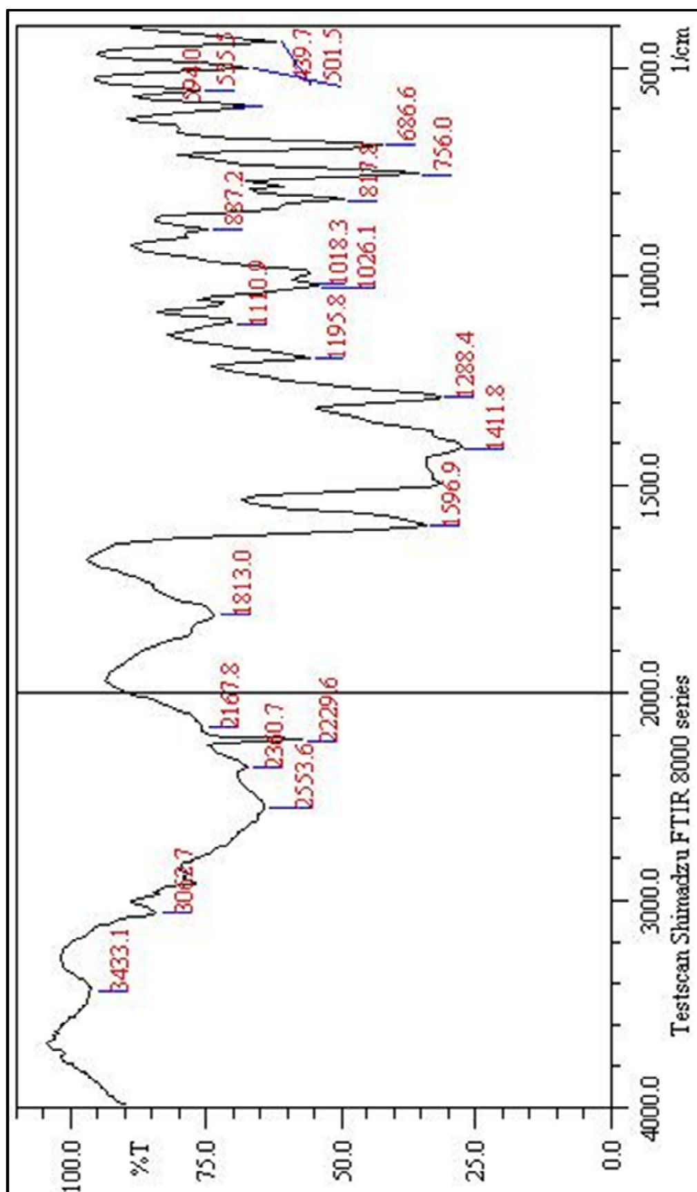
Figure 44. FT-IR spectrum of compound (6aq)
