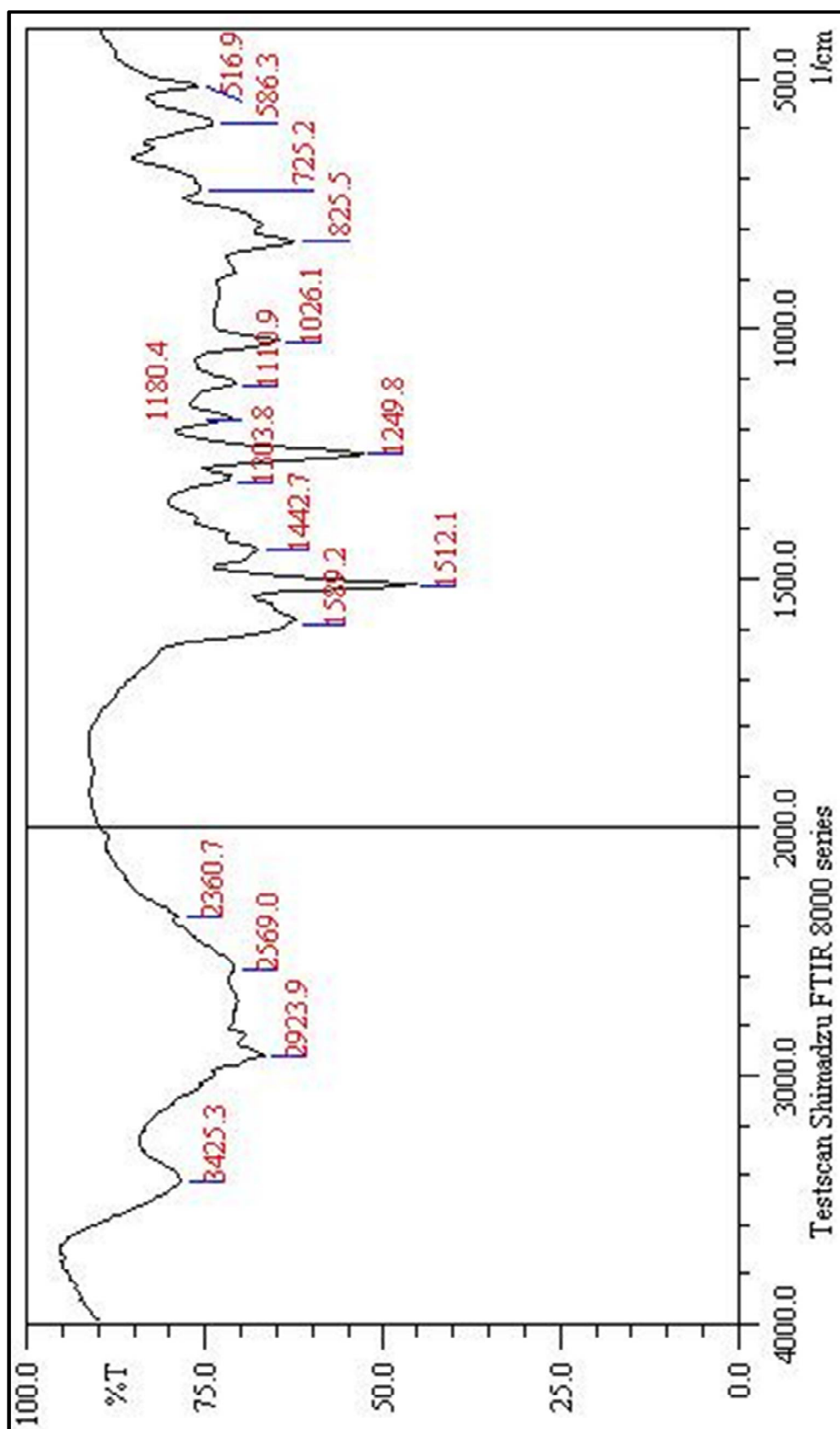
Figure 90. FT-IR spectrum of compound (6bi)
