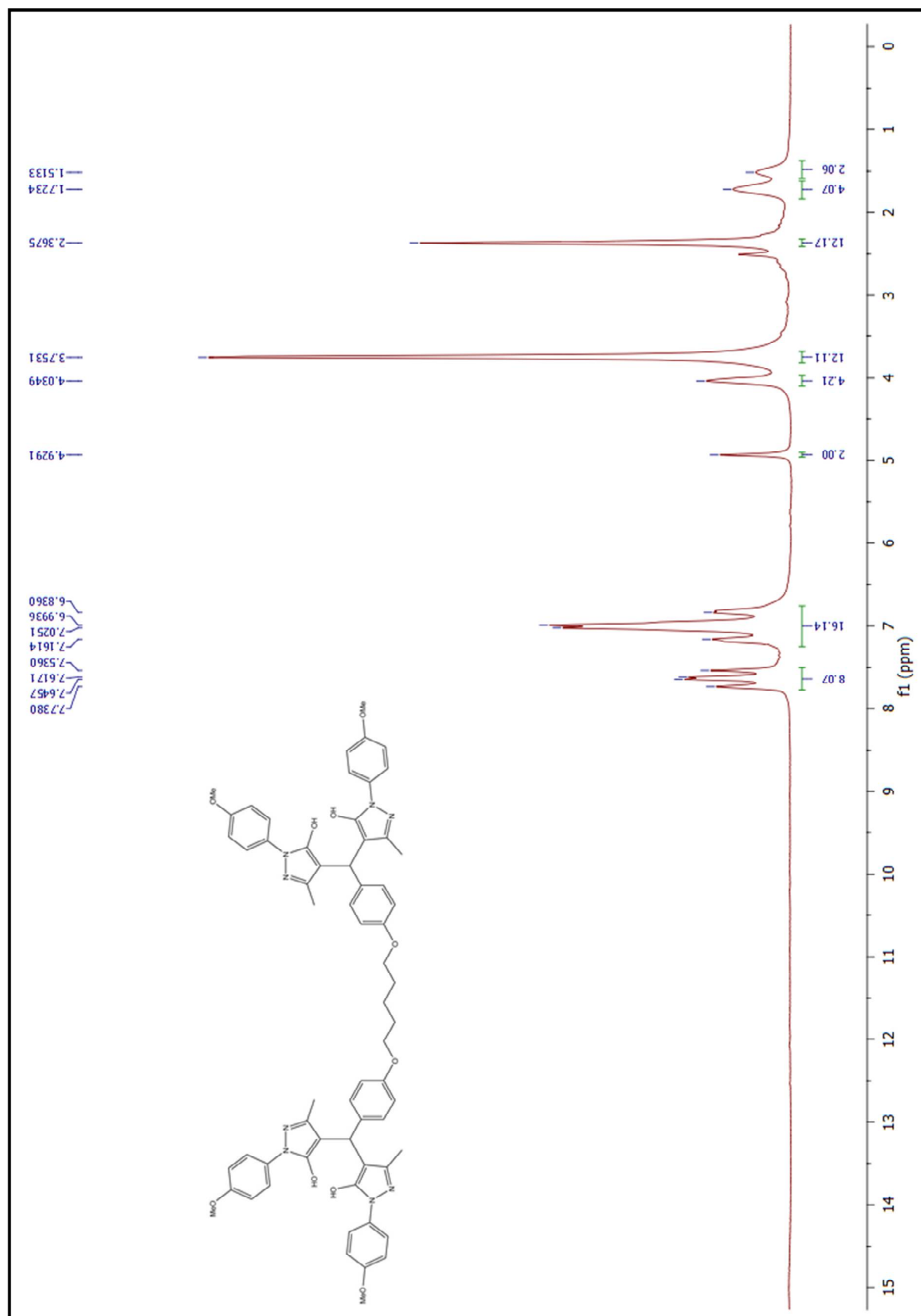
Figure 124. 1 H-NMR spectrum of compound (6bt)
