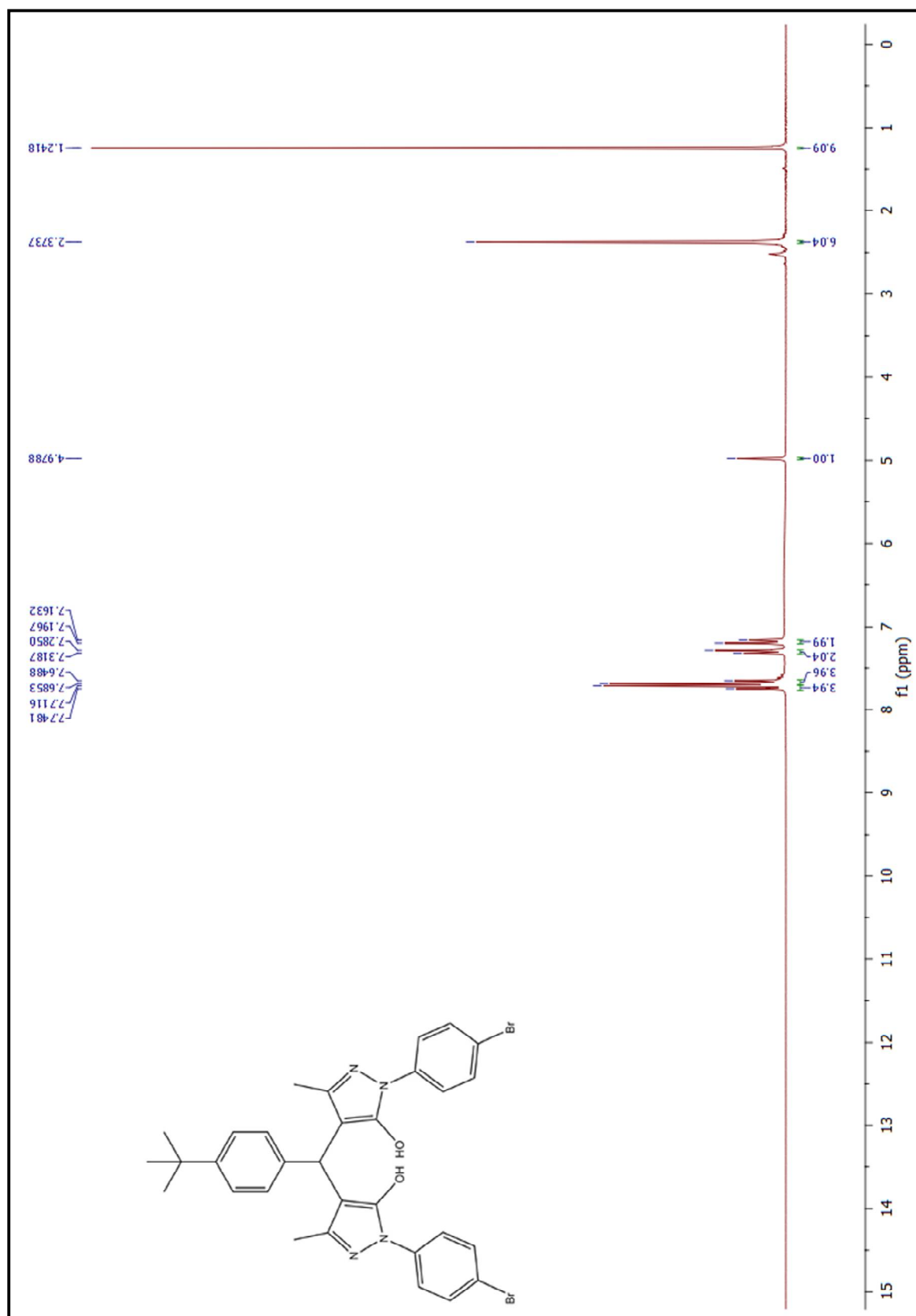
Figure 67. 1 H-NMR spectrum of compound (6ba)
