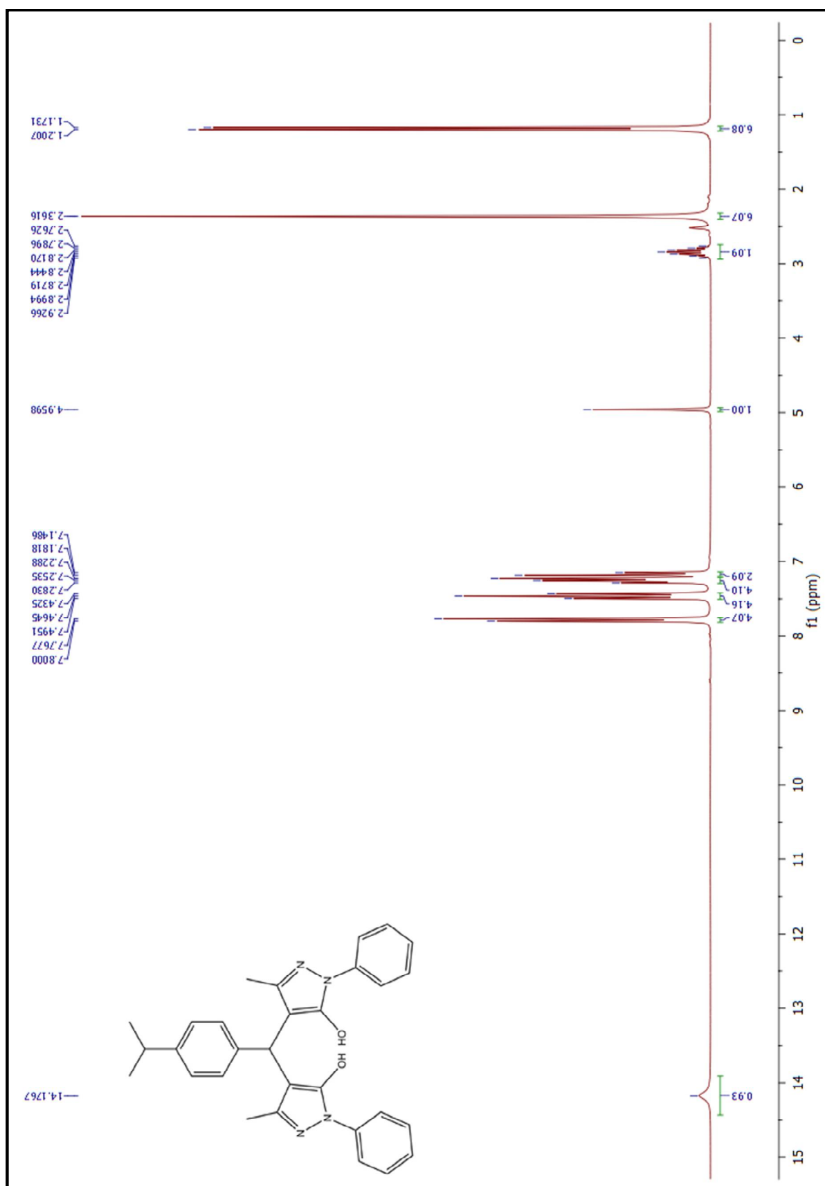
Figure 32. 1 H-NMR spectrum of compound (6ak)
