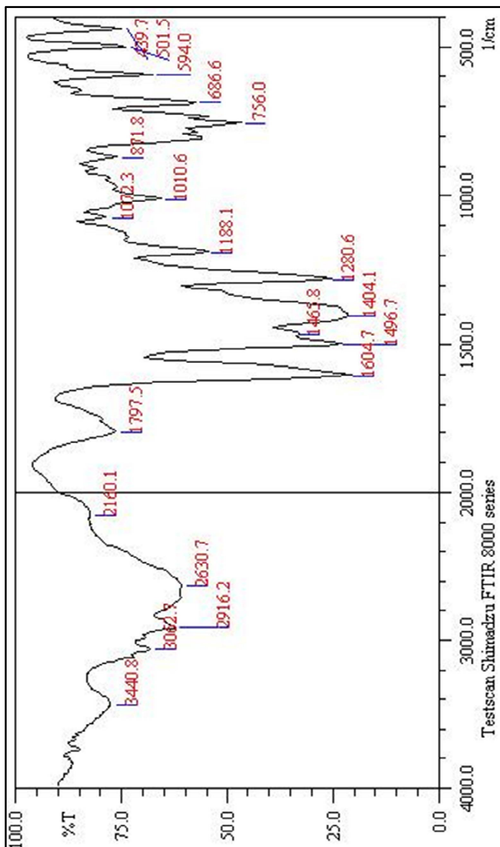
Figure 57. FT-IR spectrum of compound (6aw)
