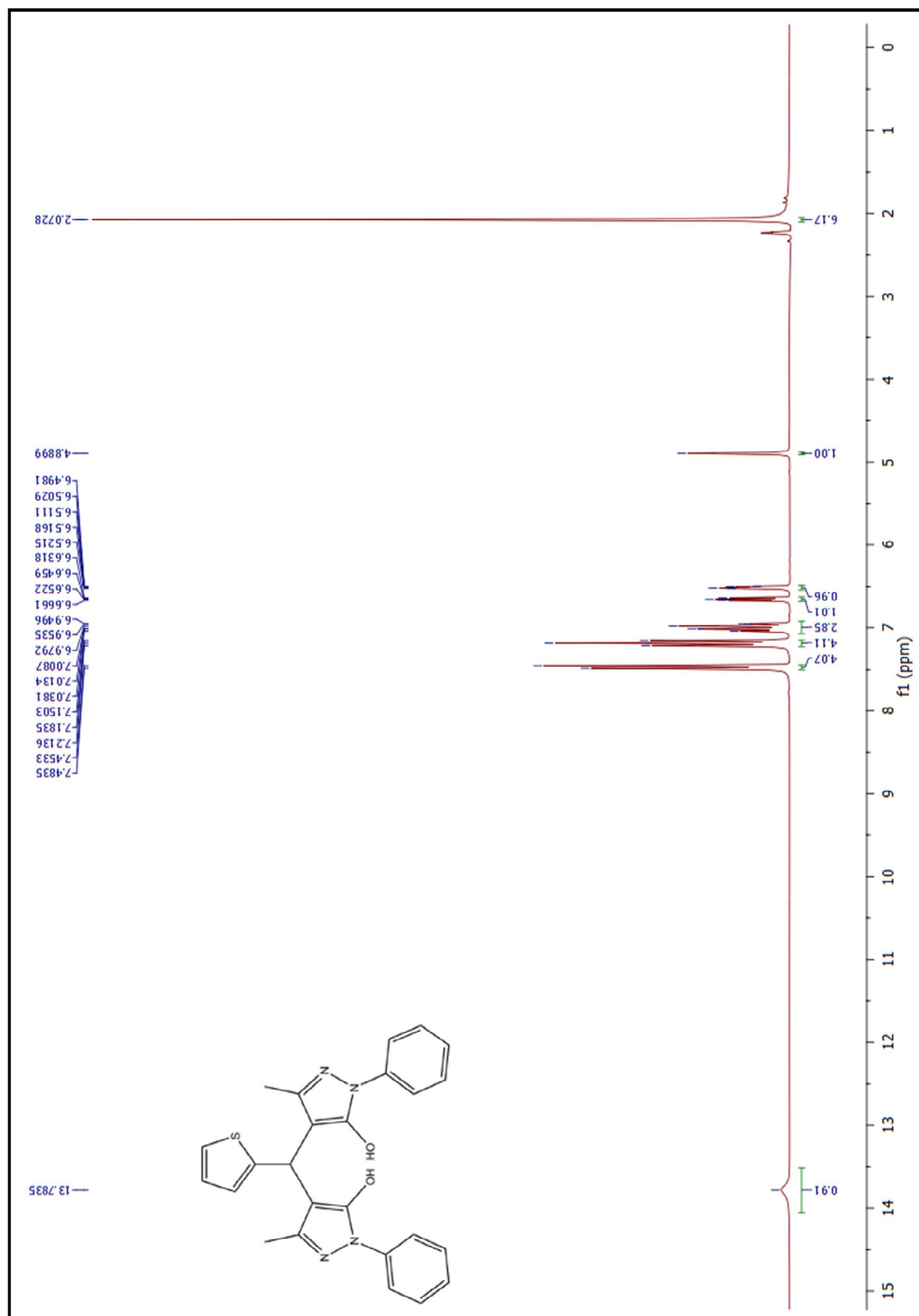
Figure 60. ^1\text{H} -NMR spectrum of compound (6ax)
