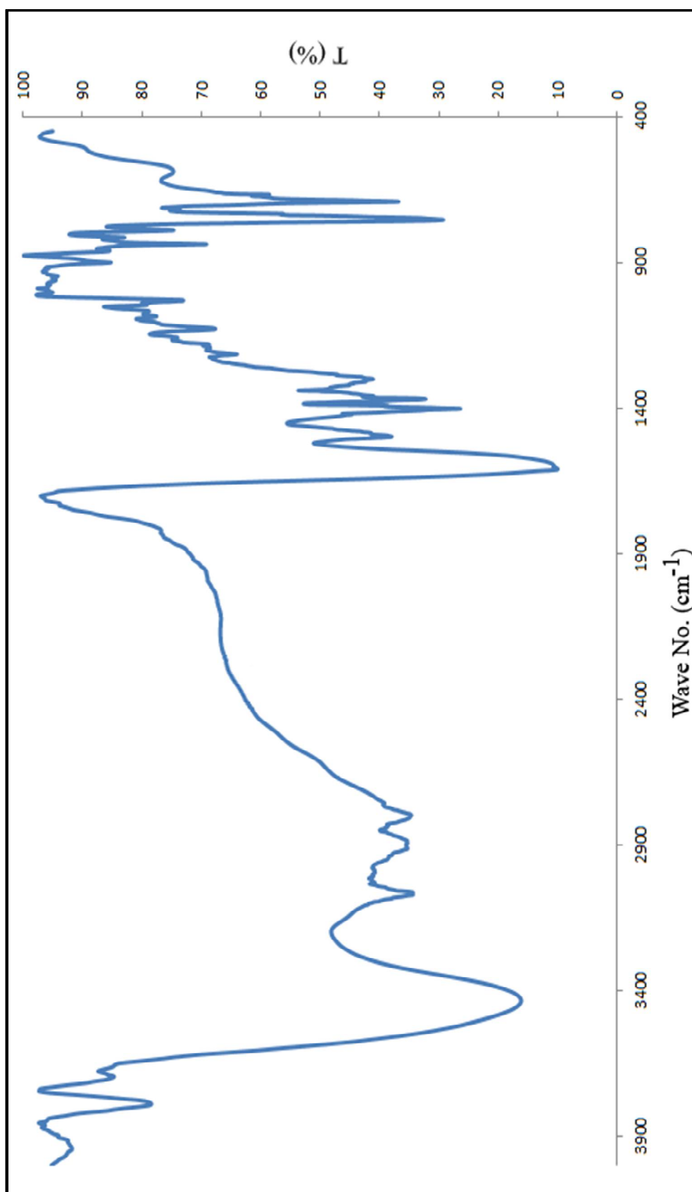
Figure 18. FT-IR spectrum of compound (6ae)
