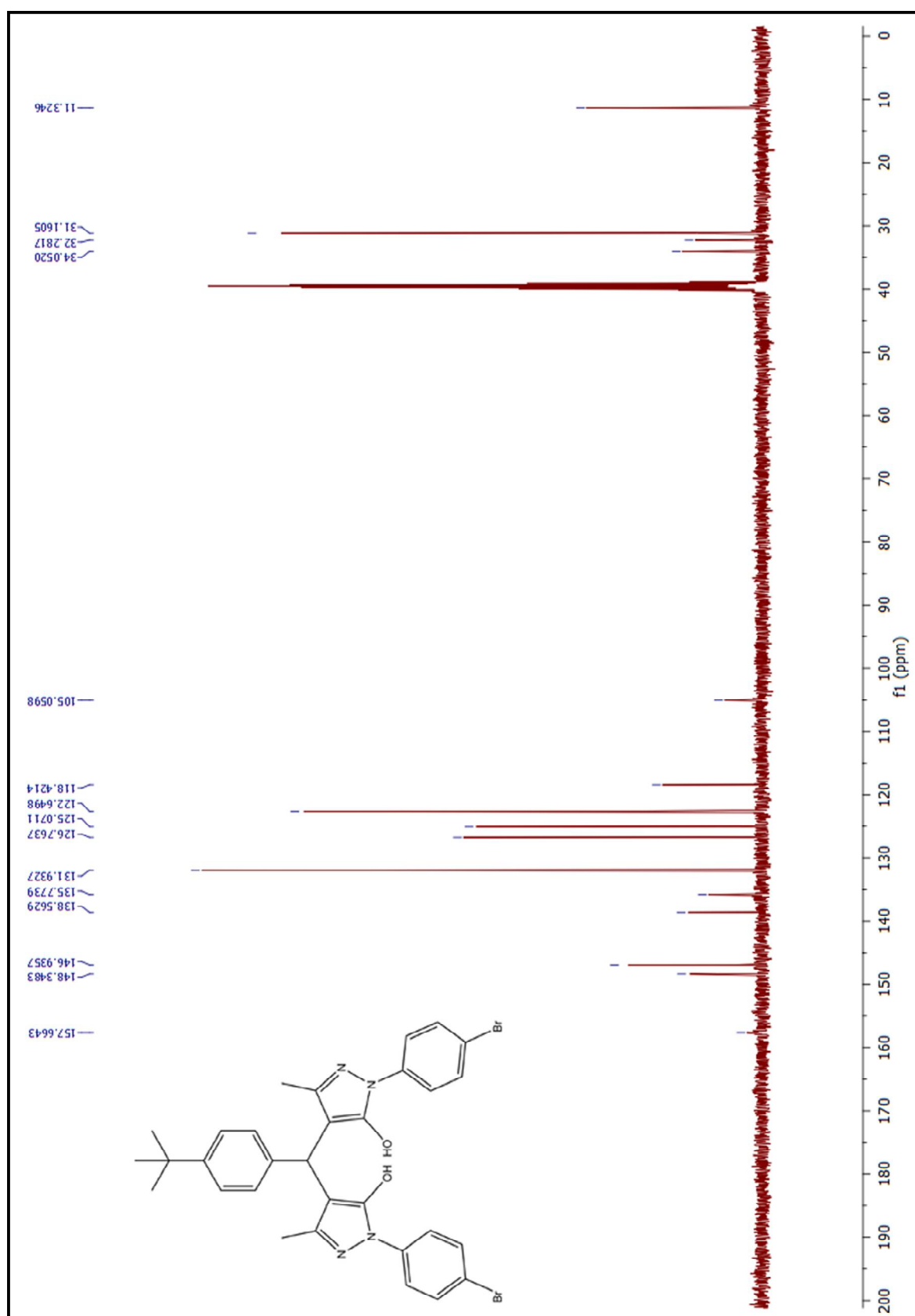
Figure 68. ^{13}\text{C} -NMR spectrum of compound (6ba)
