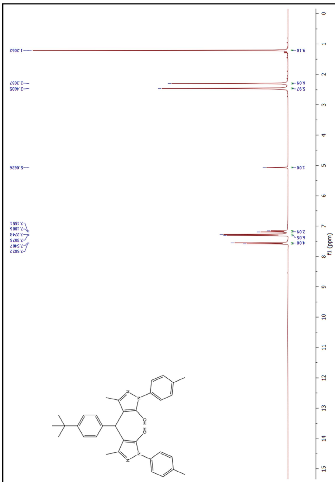
Figure 76. ^1\text{H} -NMR spectrum of compound (6bd)
