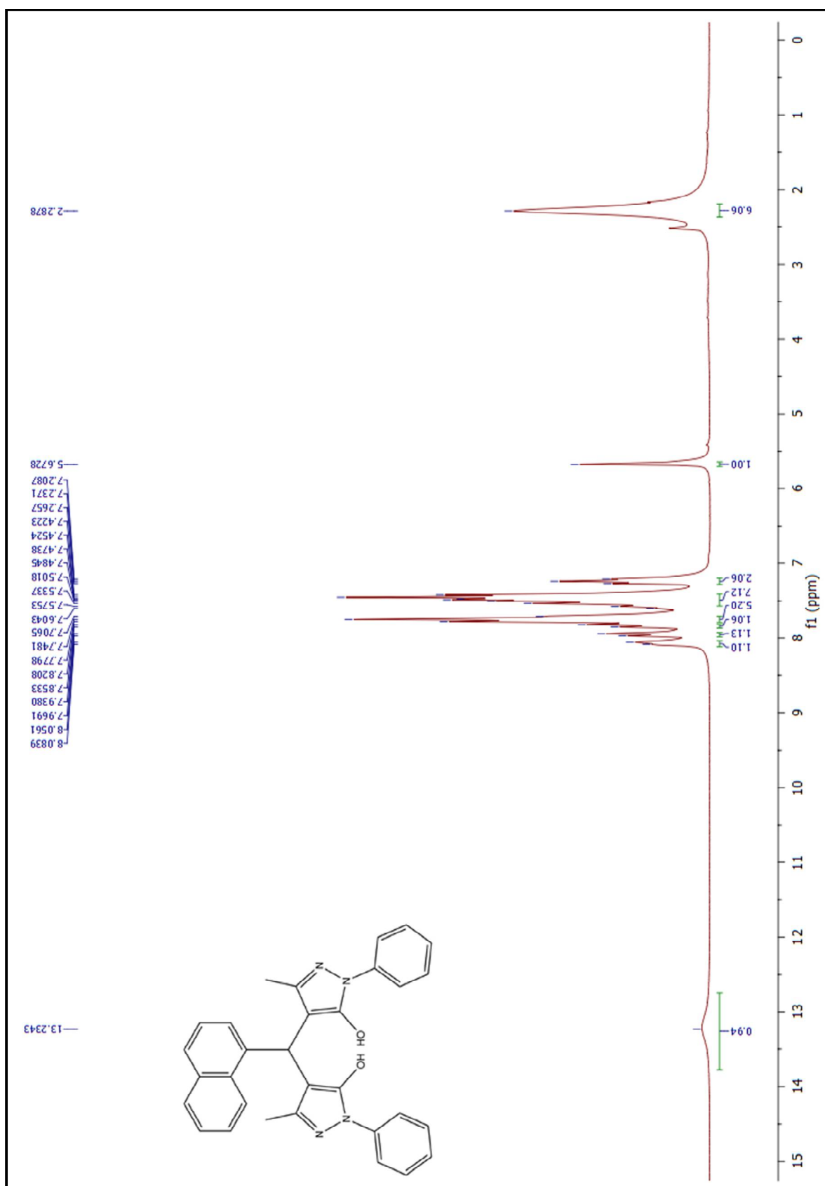
Figure 56. 1 H-NMR spectrum of compound (6av)
