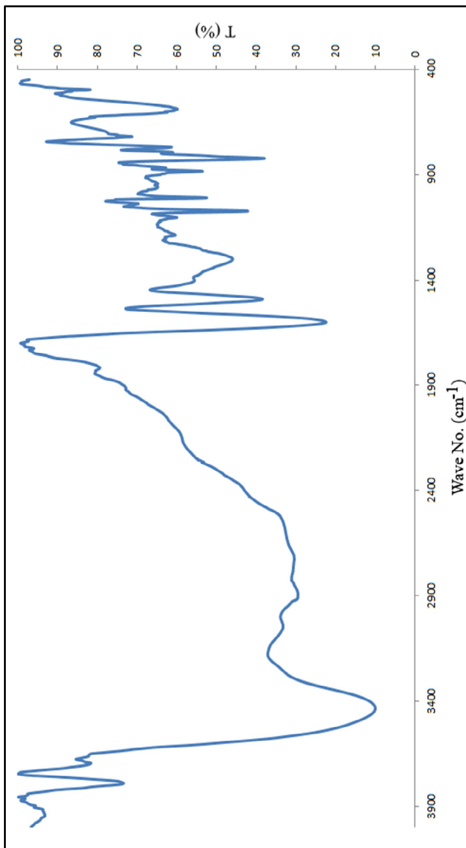
Figure 63. FT-IR spectrum of compound (6az)
