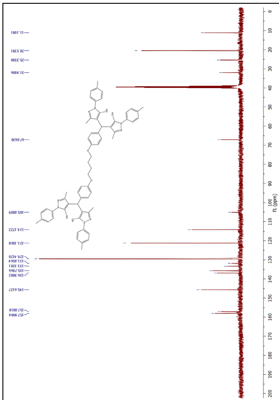
Figure 119. ^{13}\text{C} -NMR spectrum of compound (6br)
