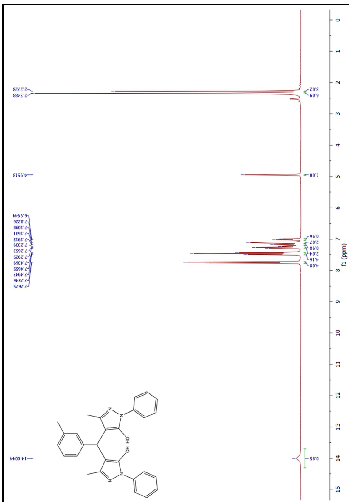
Figure 30. 1 H-NMR spectrum of compound (6aj)
