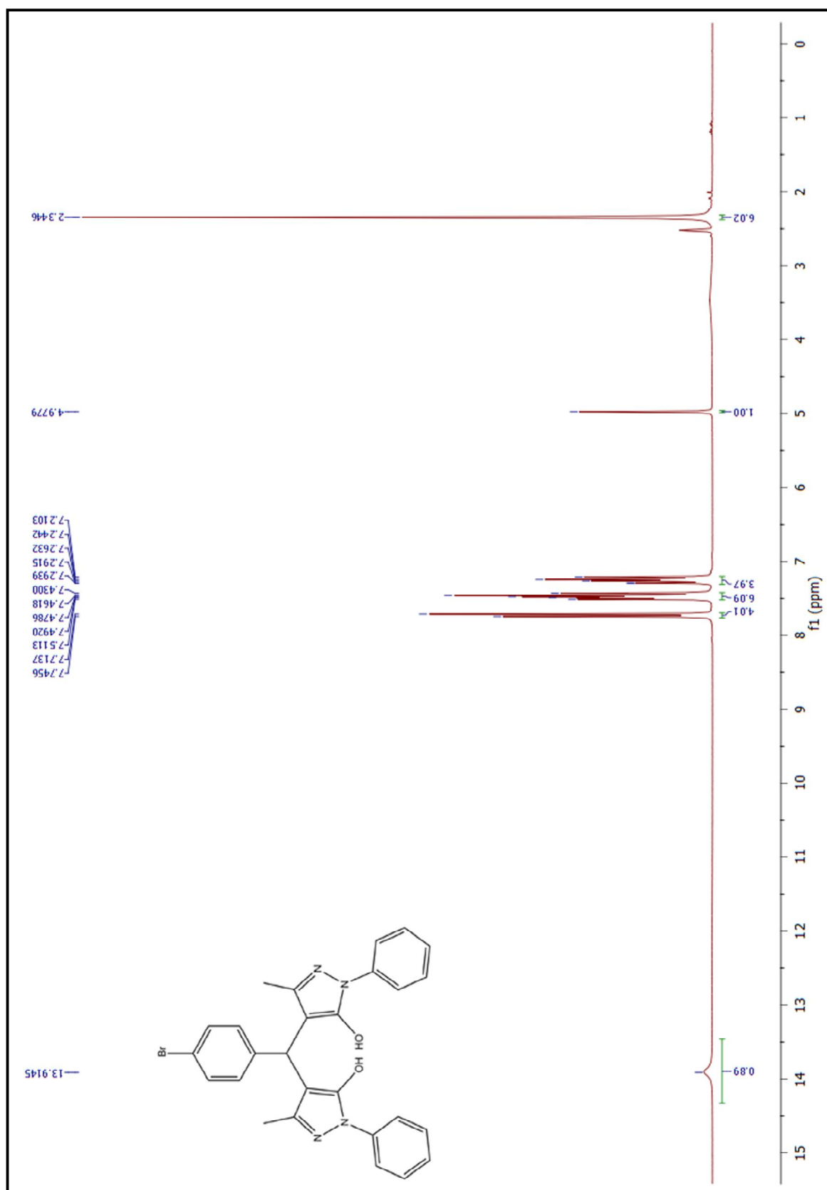
Figure 24. ^1\text{H} -NMR spectrum of compound (6ag)
