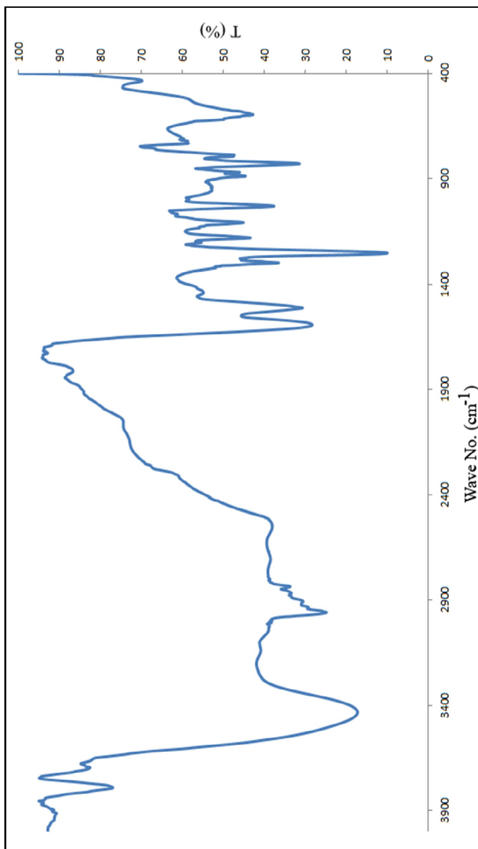
Figure 93. FT-IR spectrum of compound (6bj)
