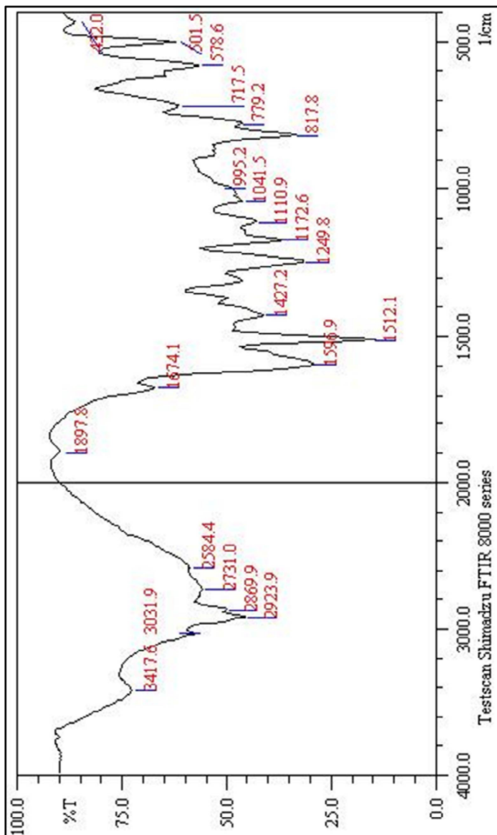
Figure 117. FT-IR spectrum of compound (6br)
