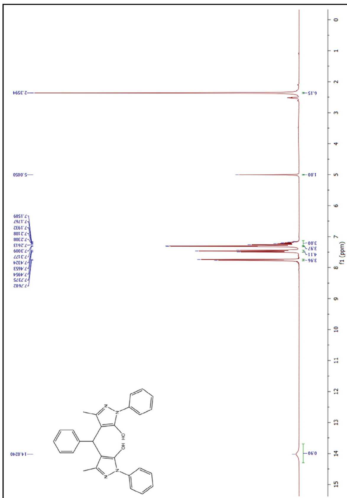
Figure 11. ^1\text{H} -NMR spectrum of compound (6aa)
