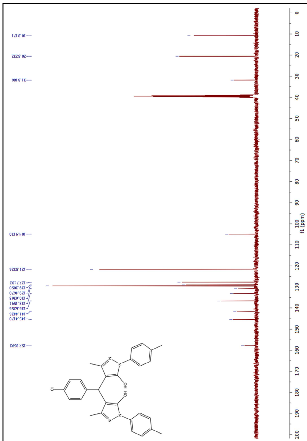
Figure 74. ^{13}\text{C} -NMR spectrum of compound (6bc)
