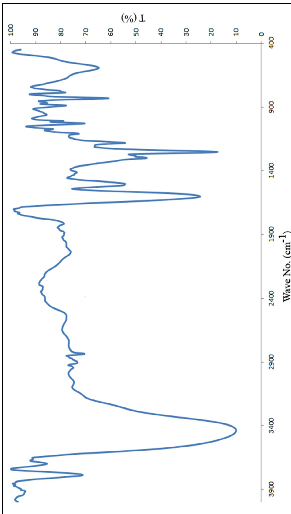
Figure 87. FT-IR spectrum of compound (6bh)
