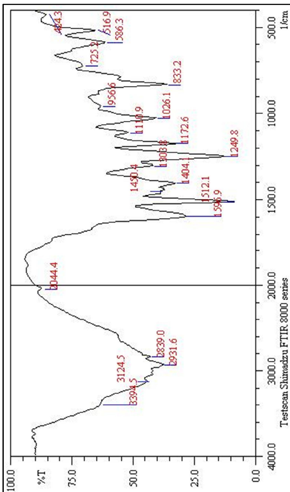
Figure 120. FT-IR spectrum of compound (6bs)
