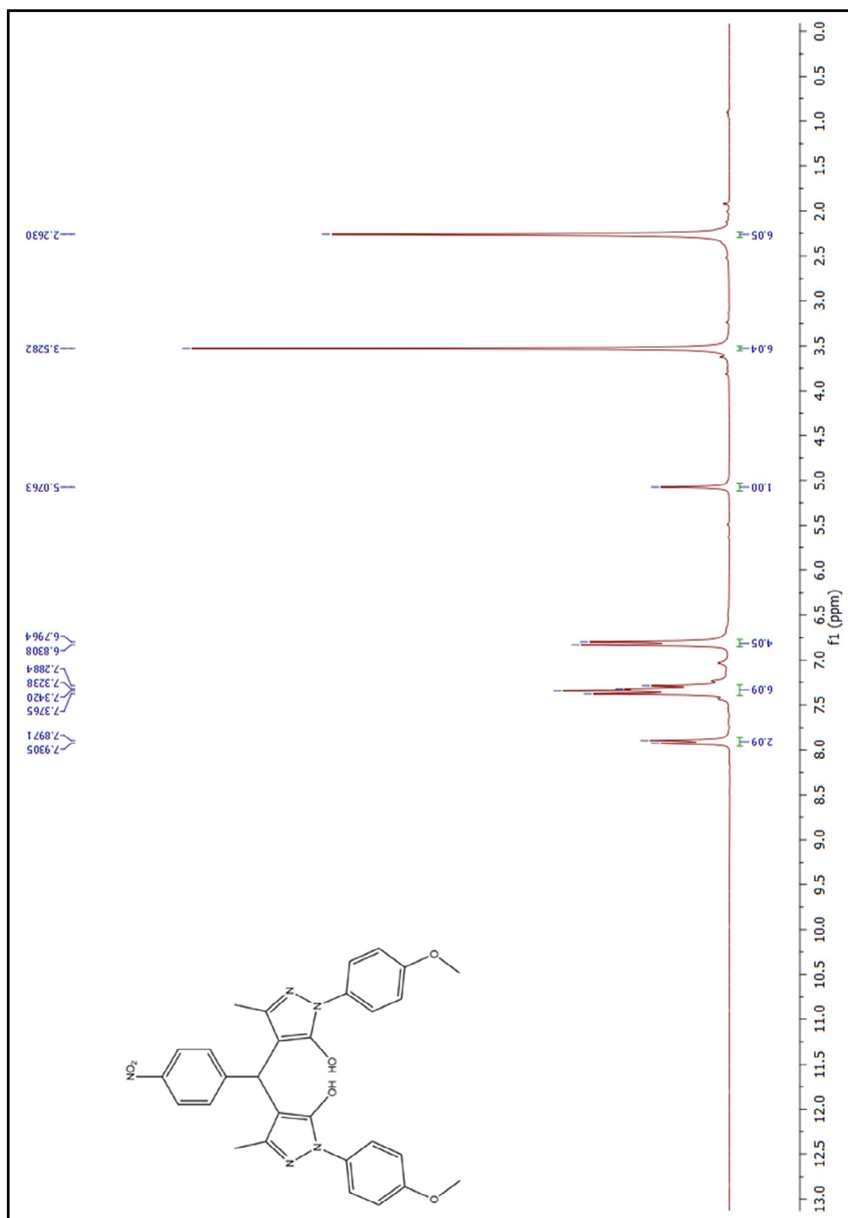
Figure 97. ^1\text{H} -NMR spectrum of compound (6bk)
