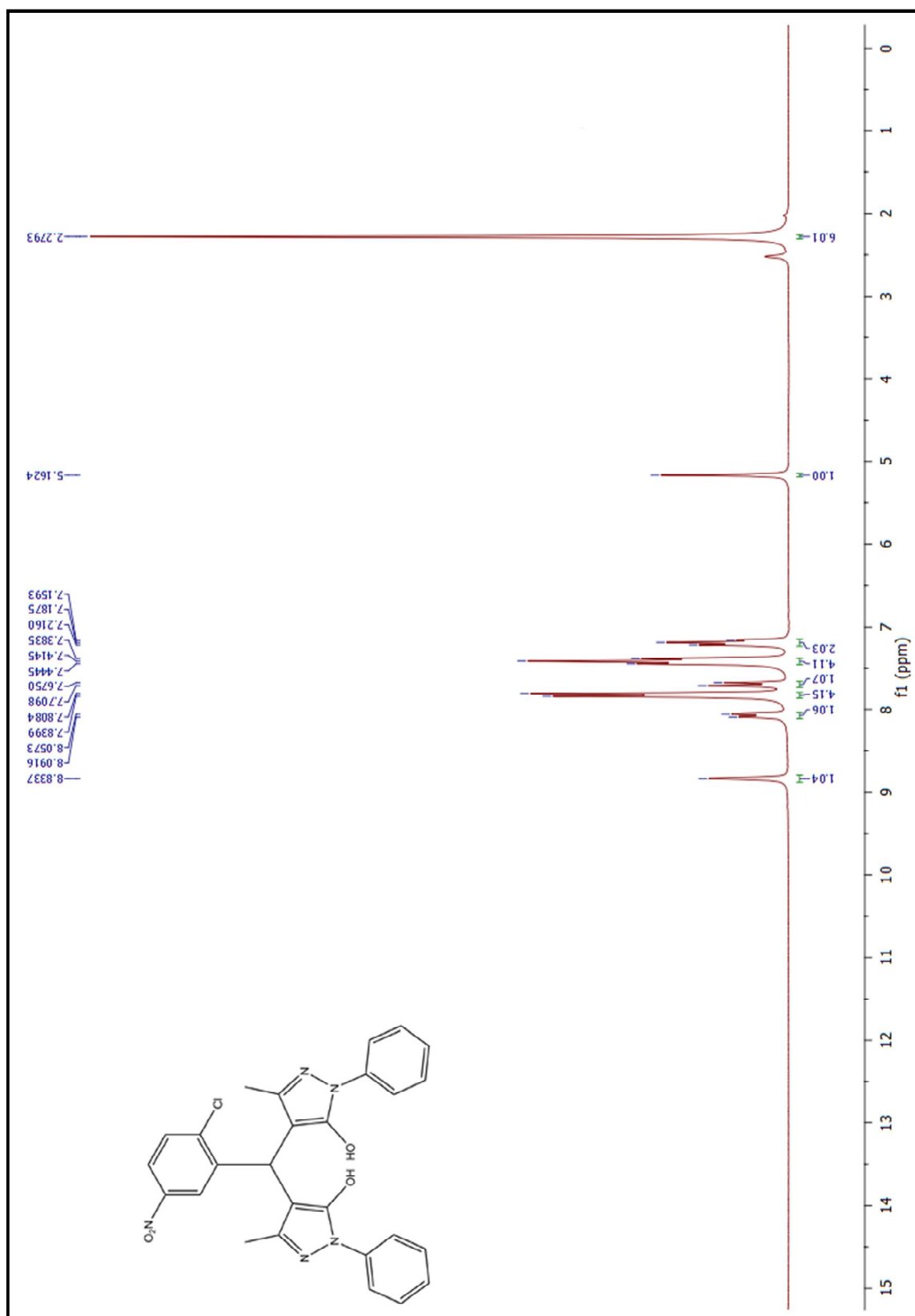
Figure 53. 1 H-NMR spectrum of compound (6au)
