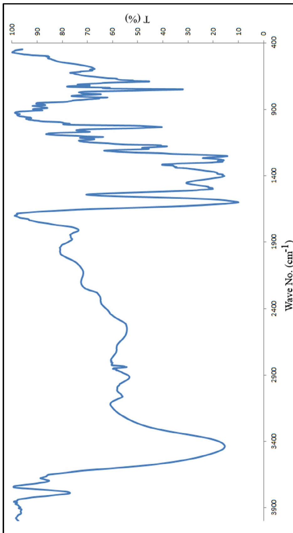
Figure 38. FT-IR spectrum of compound (6an)
