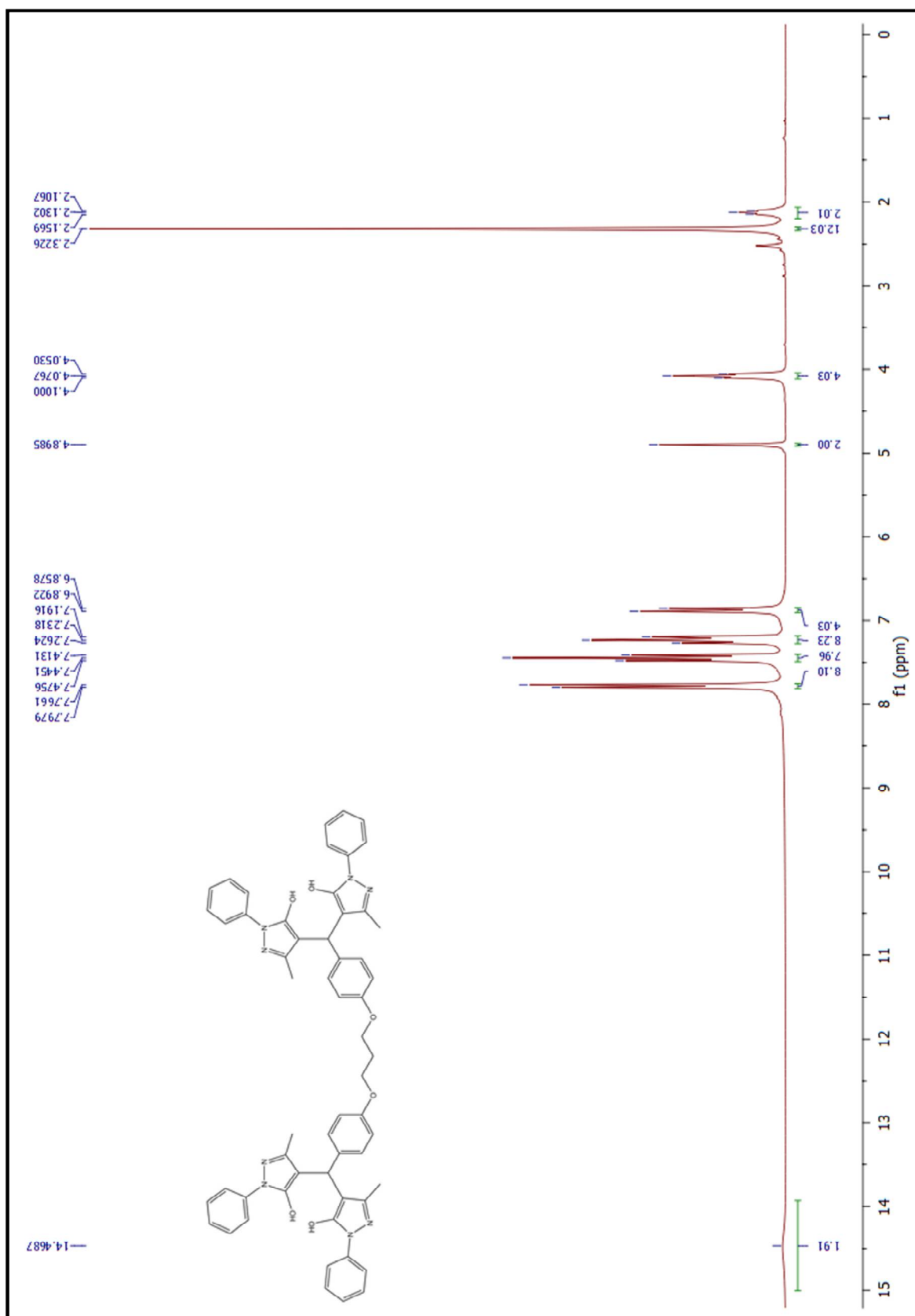
Figure 100. 1 H-NMR spectrum of compound (6bl)
