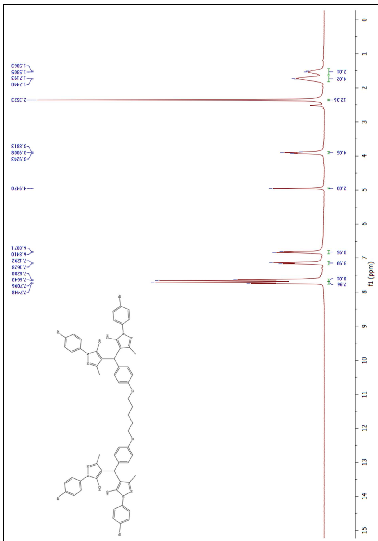
Figure 112. ^1\text{H} -NMR spectrum of compound (6bp)
