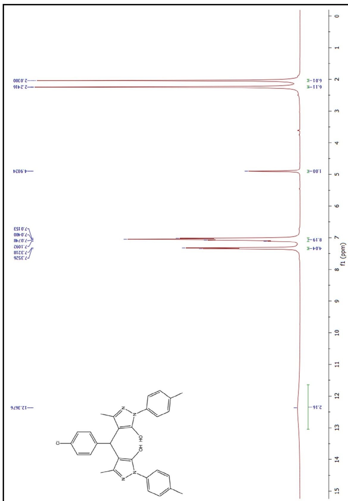
Figure 73. 1 H-NMR spectrum of compound (6bc)
