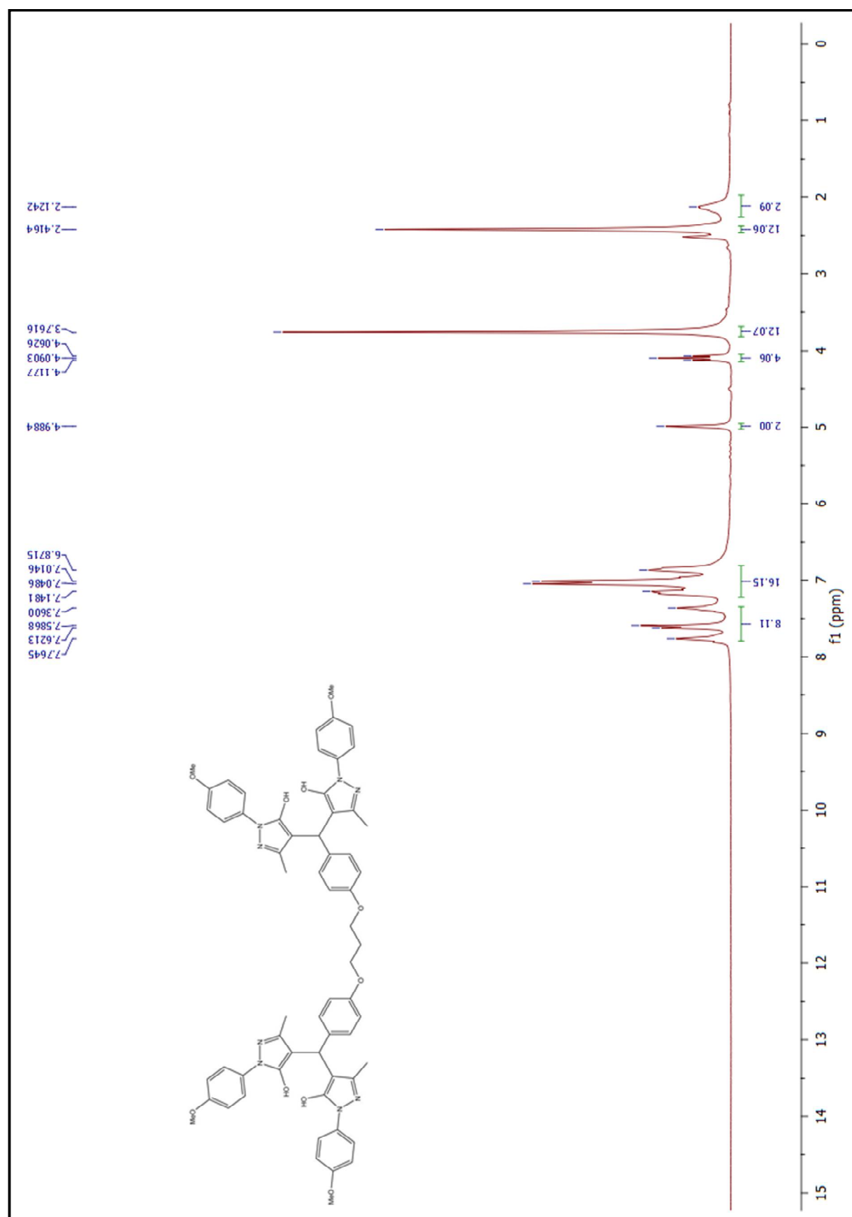
Figure 121. ^1\text{H} -NMR spectrum of compound (6bs)
