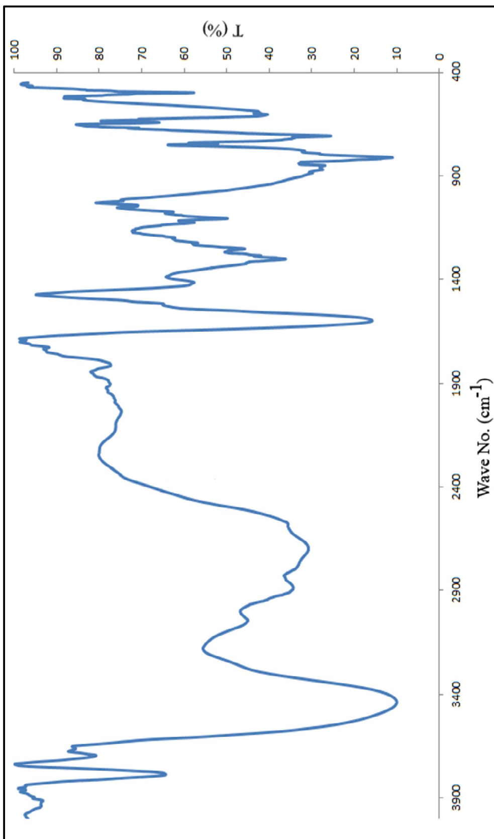
Figure 81. FT-IR spectrum of compound (6bf)
