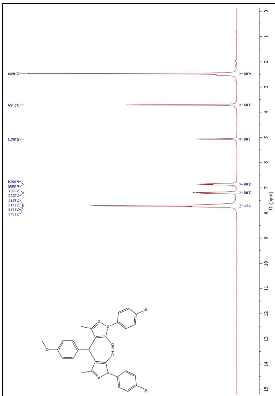
Figure 70. 1 H-NMR spectrum of compound (6bb)
