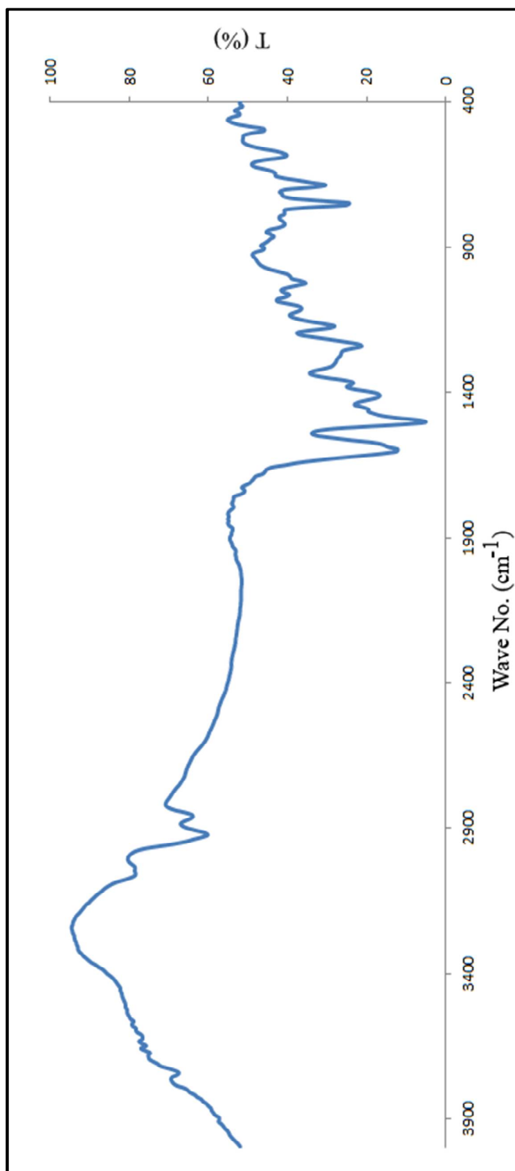
Figure 105. FT-IR spectrum of compound (6bn)
