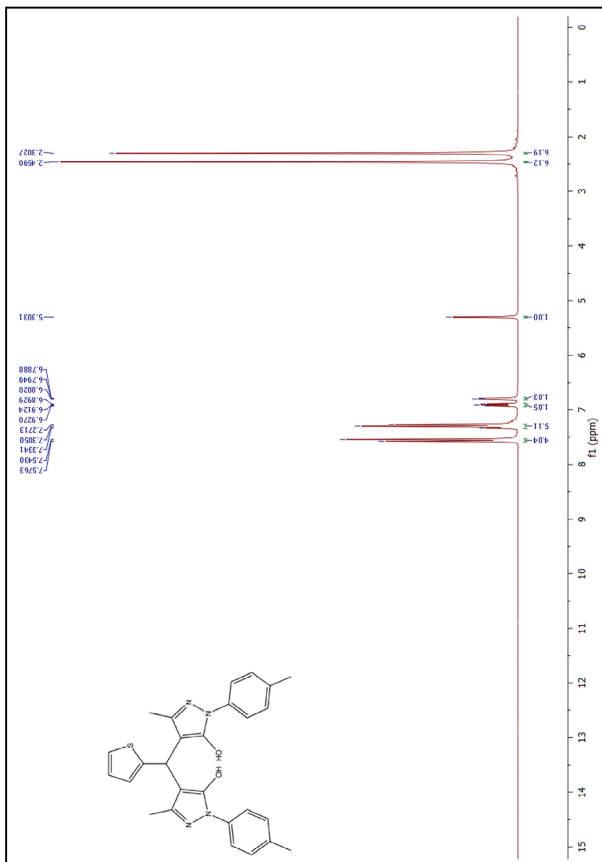
Figure 82. 1 H-NMR spectrum of compound (6bf)
