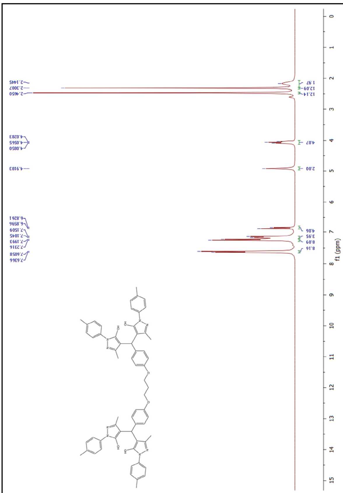
Figure 115. ^1\text{H} -NMR spectrum of compound (6bq)
