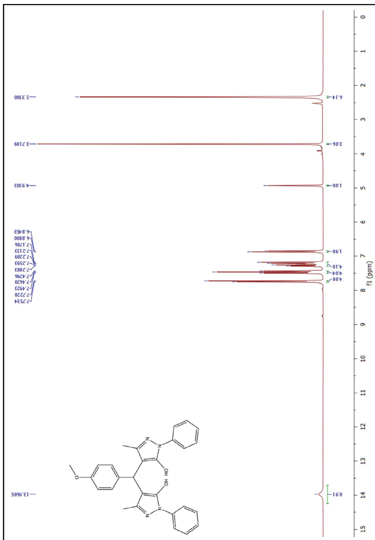
Figure 39. 1 H-NMR spectrum of compound (6an)
