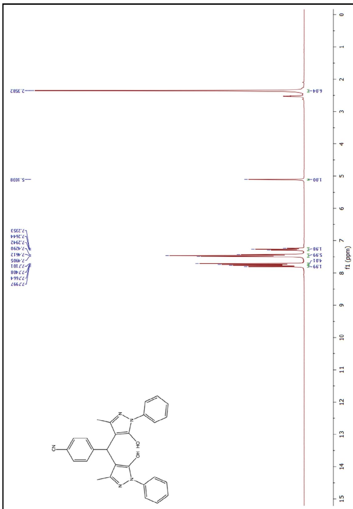
Figure 45. 1 H-NMR spectrum of compound (6aq)
