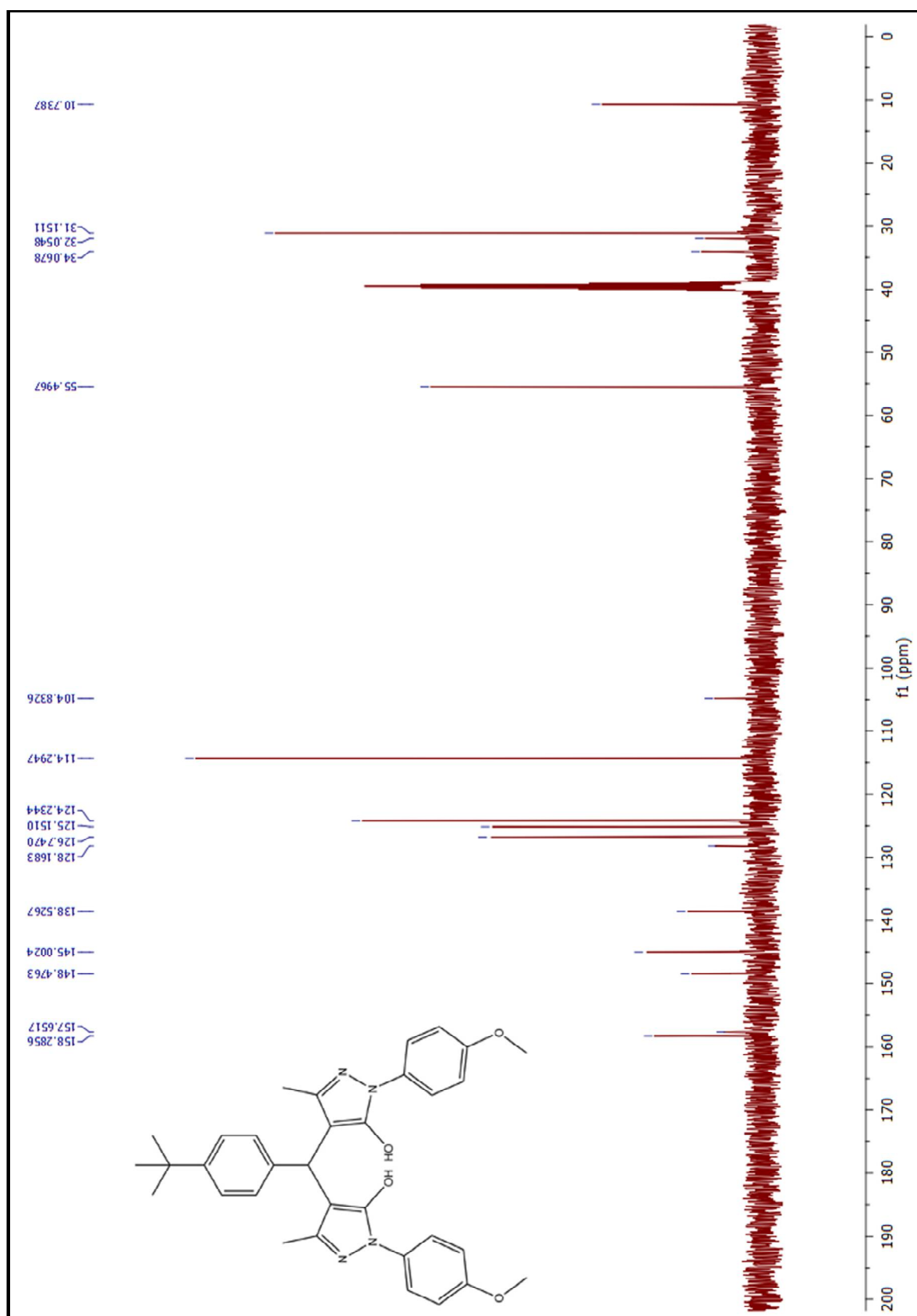
Figure 95. ^{13}\text{C} -NMR spectrum of compound (6bj)
