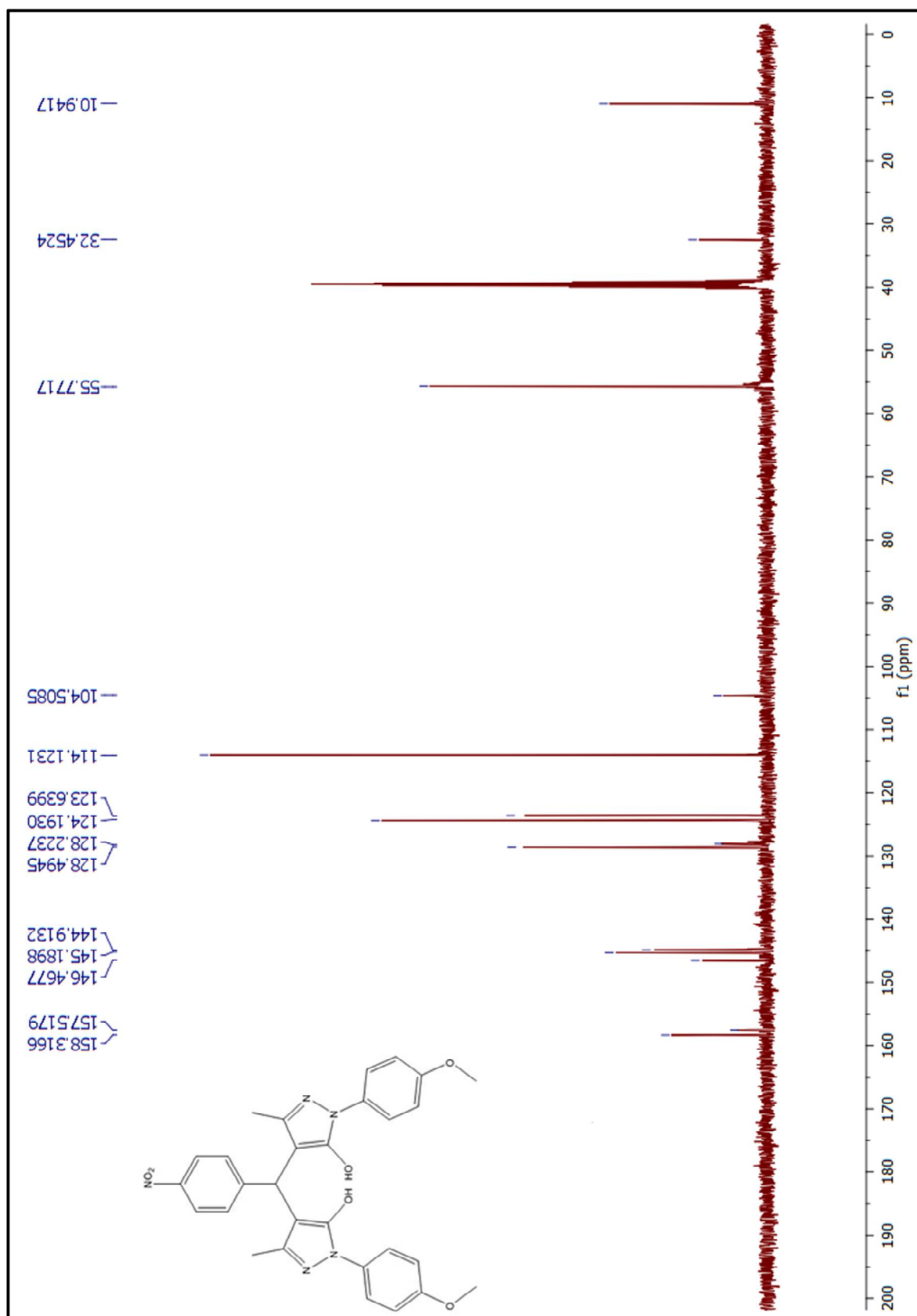
Figure 98. ^{13}\text{C} -NMR spectrum of compound (6bk)
