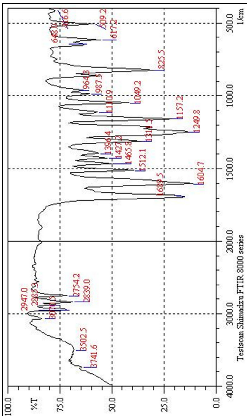
Figure 1. FT-IR spectrum of compound (4a)
