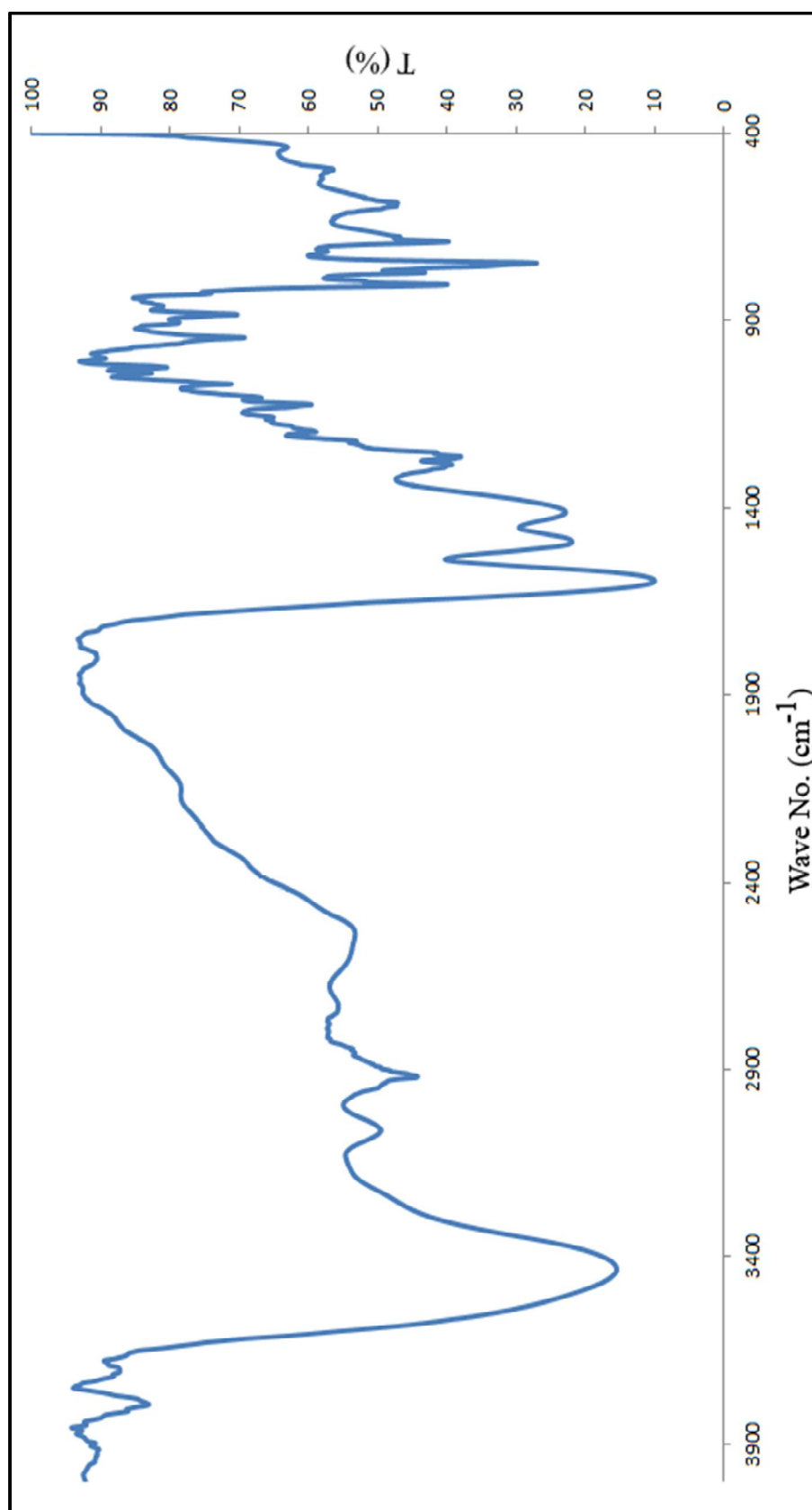
Figure 14. FT-IR spectrum of compound (6ac)
