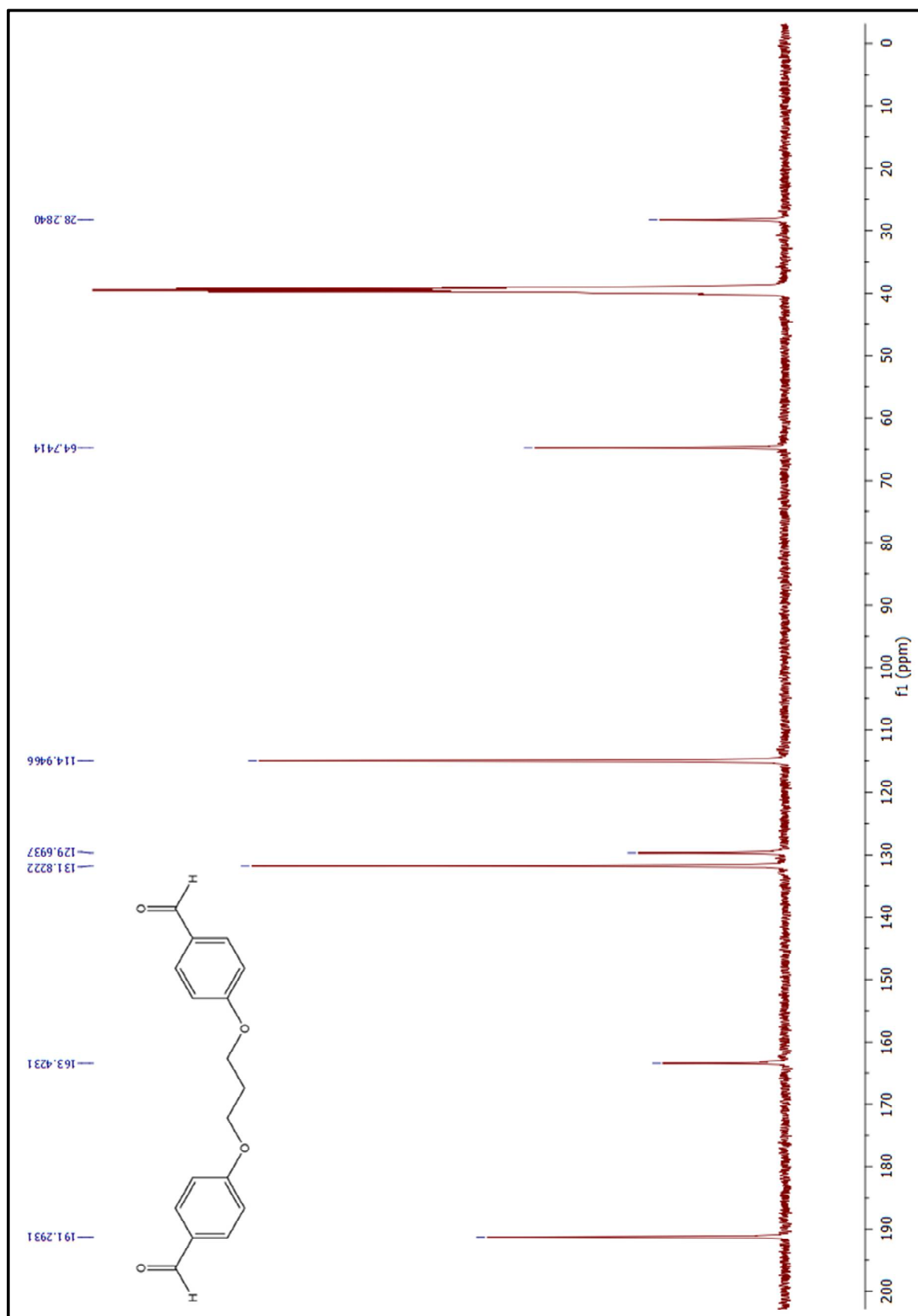
Figure 3. ^{13}\text{C} -NMR spectrum of compound (4a)
