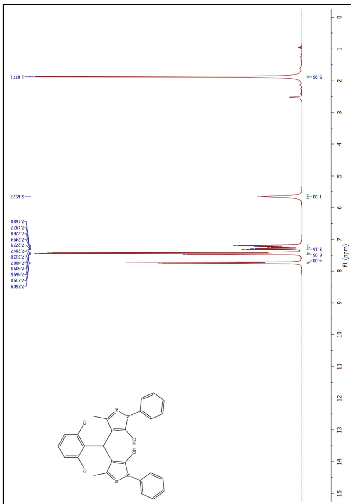
Figure 21. ^1\text{H} -NMR spectrum of compound (6af)
