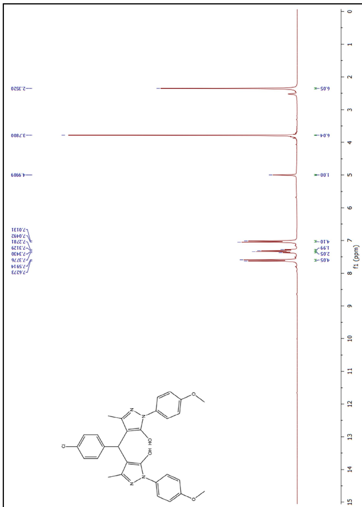
Figure 85. 1 H-NMR spectrum of compound (6bg)
