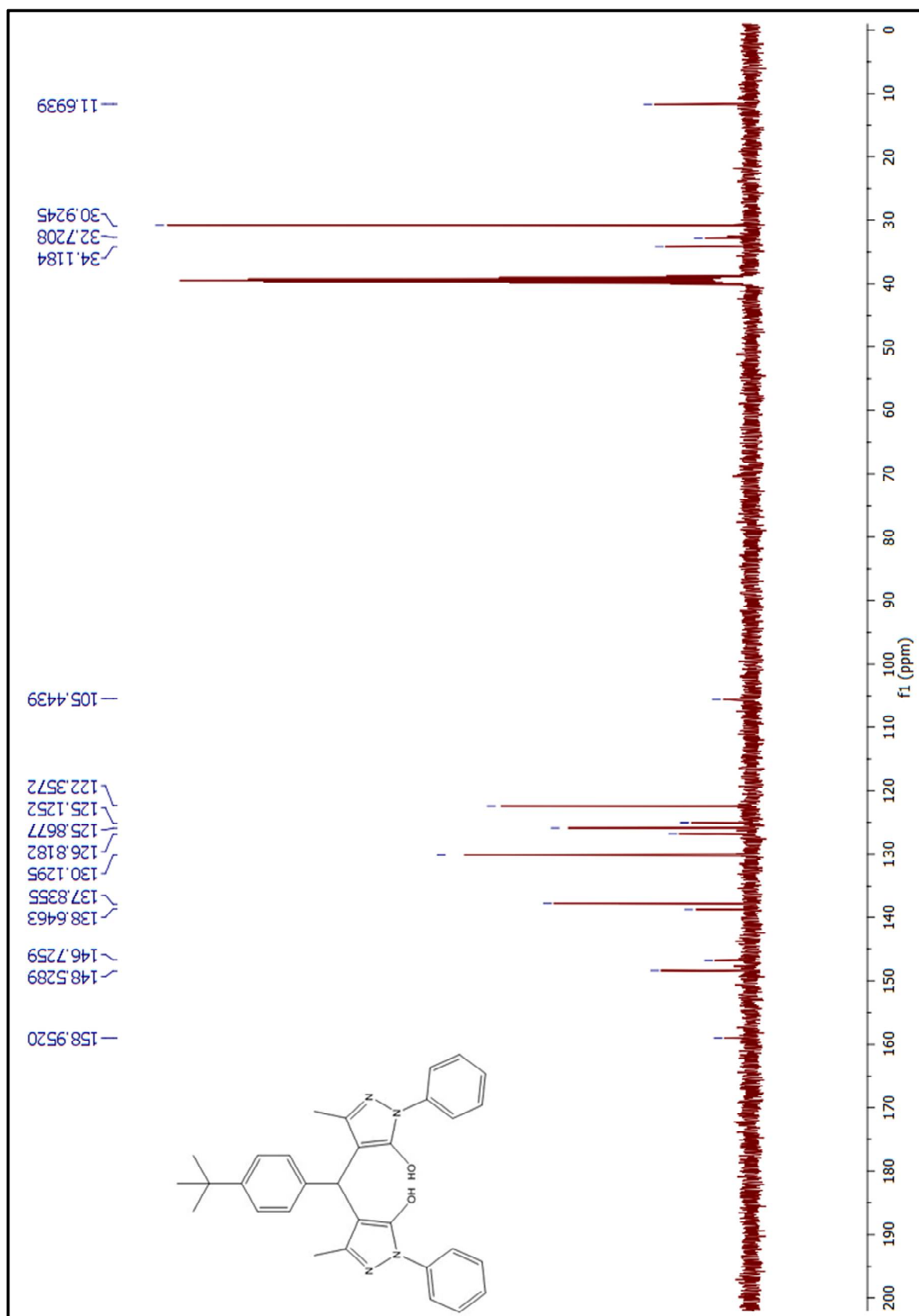
Figure 35. ^{13}\text{C} -NMR spectrum of compound (6al)
