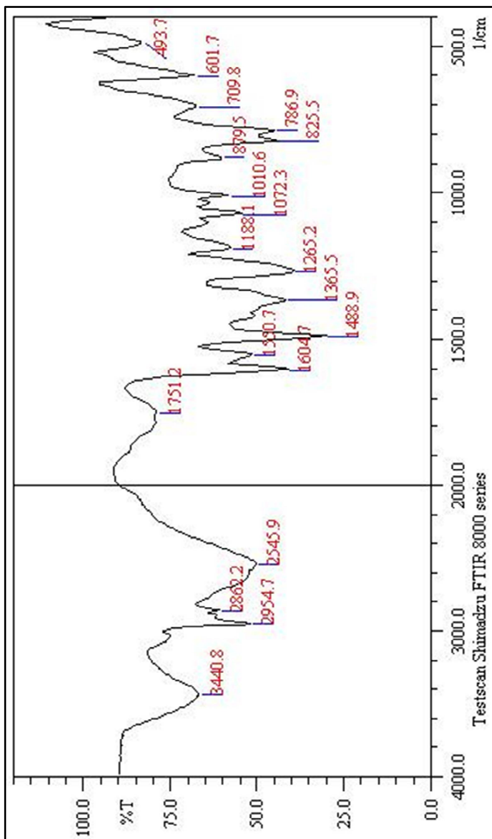
Figure 66. FT-IR spectrum of compound (6ba)
