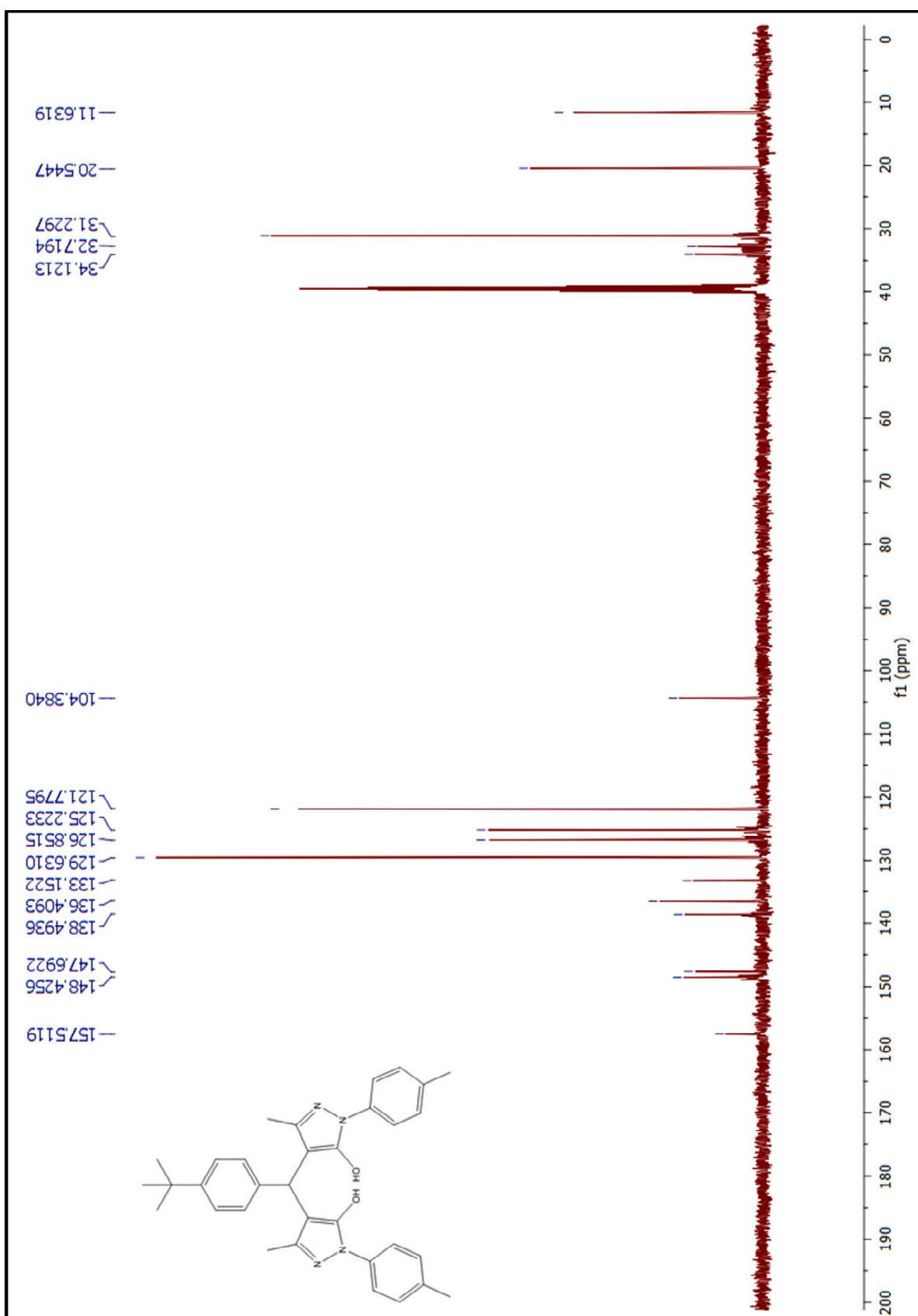
Figure 77. 13 C-NMR spectrum of compound (6bd)
