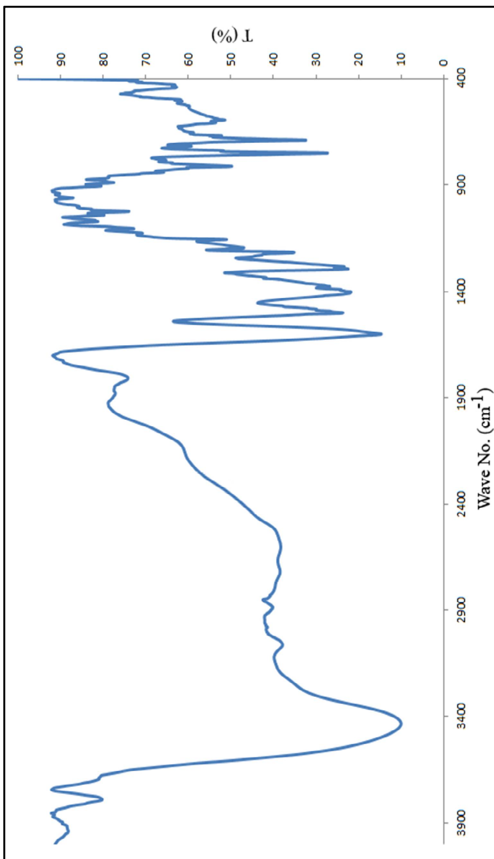
Figure 12. FT-IR spectrum of compound (6ab)
