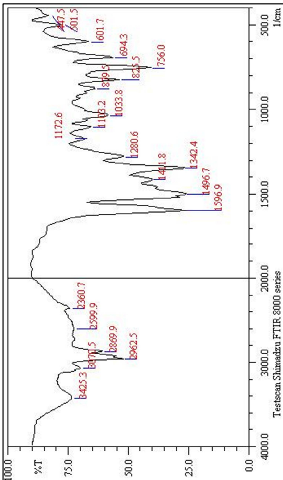
Figure 52. FT-IR spectrum of compound (6au)
