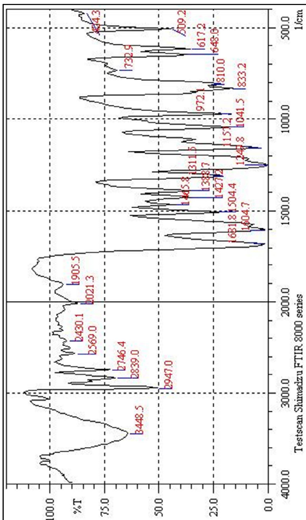
Figure 4. FT-IR spectrum of compound (4b)
