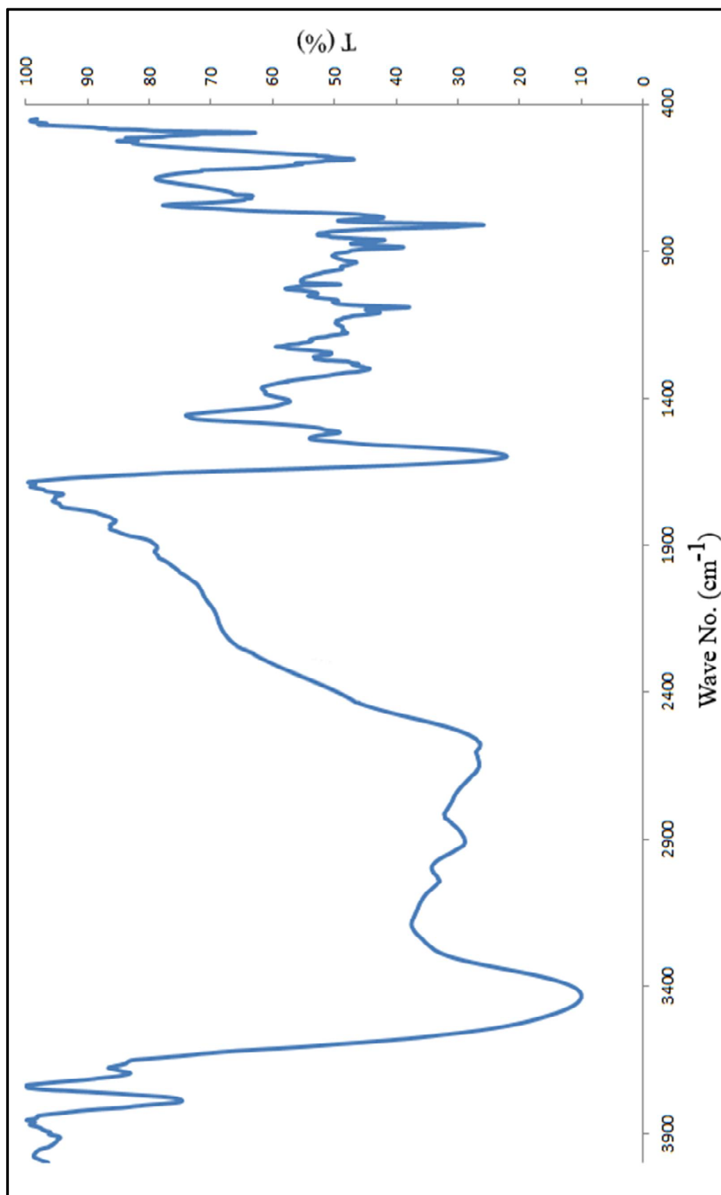
Figure 72. FT-IR spectrum of compound (6bc)
