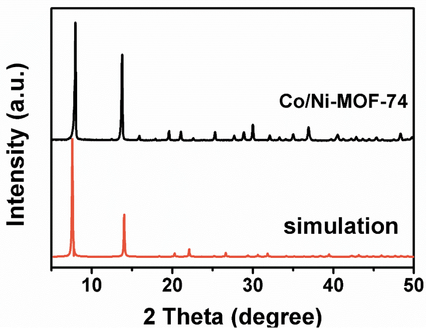
Fig. S1 XRD patterns of Co/Ni-MOF-74
