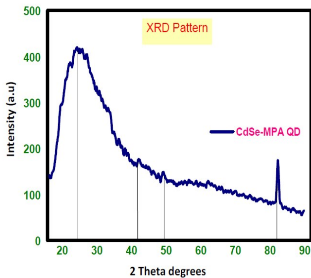
Fig. S2 XRD pattern of CdSe-MPA QD
