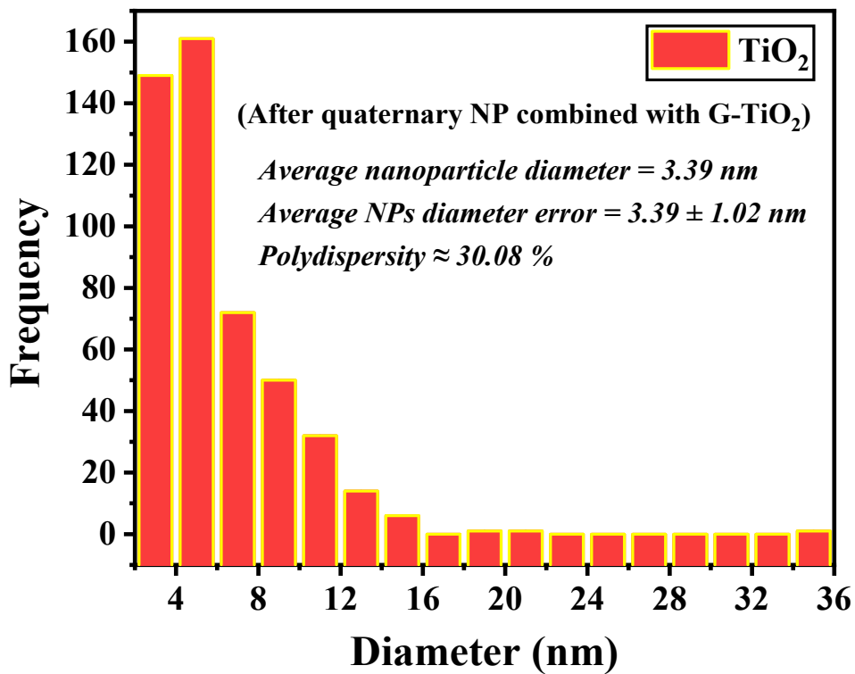
Figure S3. Nanoparticle size histogram of TiO 2 after quaternary nanoparticle combined with Graphene-TiO 2 .
