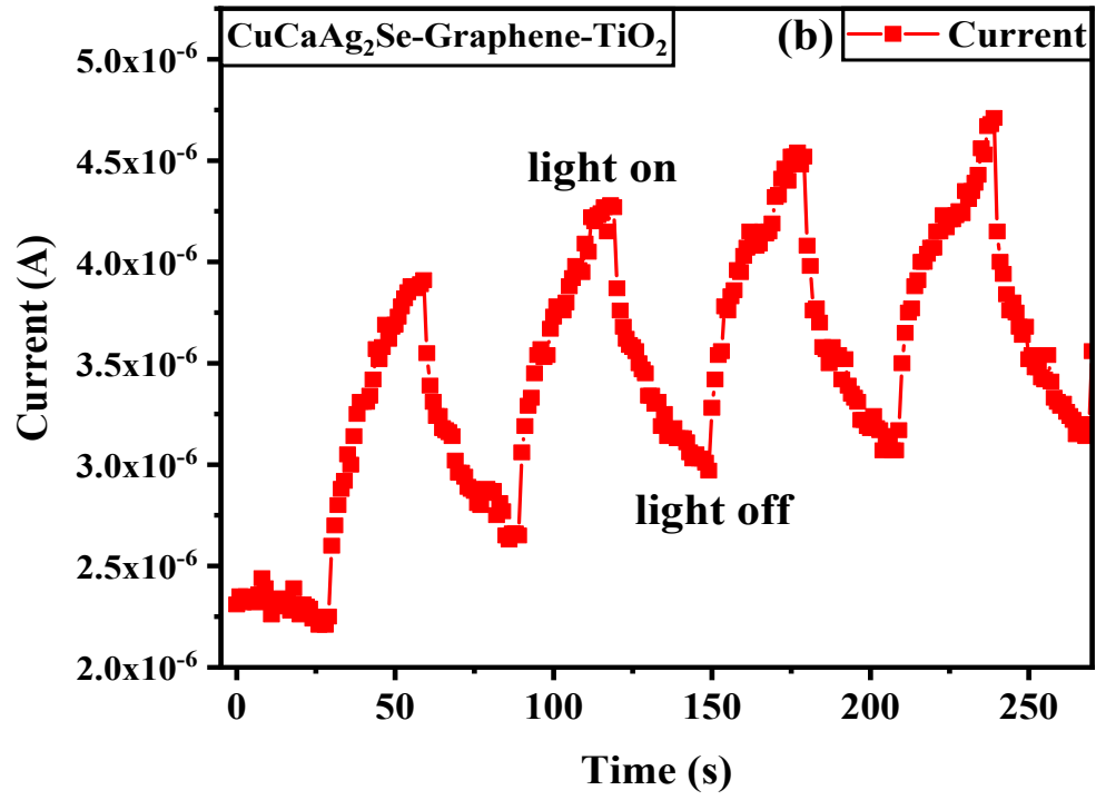
Figure S5. Photocurrent result of CuCaAg 2 Se and CuCaAg 2 Se-Graphene-TiO 2 nanocomposite.
