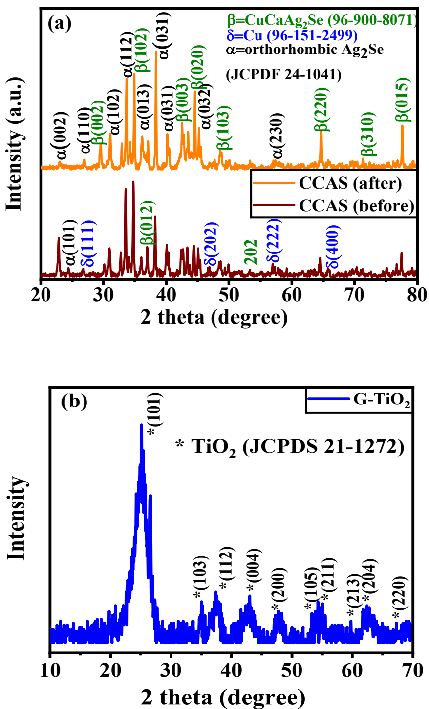
Figure S1. XRD pattern of (a) CuCaAg 2 Se (b) G-TiO 2 nanocomposite.
