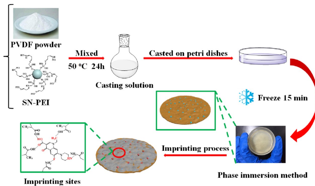
Fig. S1 The synthesis pathway of SPEIMs.
