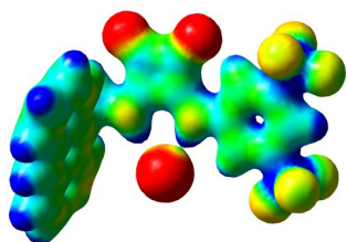
3-Cl -
