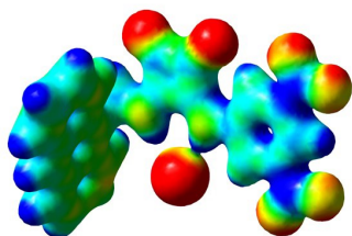
5-Cl -
