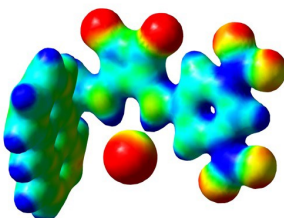
5-Br -
