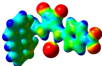
4-Cl -
