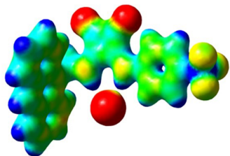
2-Cl -
