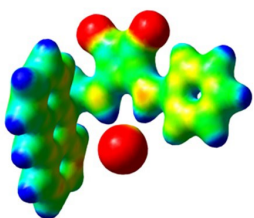
1-Br
