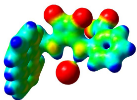
6-Cl -
