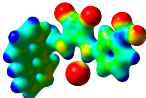
7-Cl -
