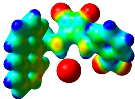
9-Cl -
