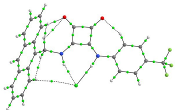
2-Cl -
