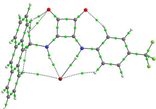
2-Br
