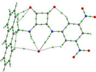
5-Br
