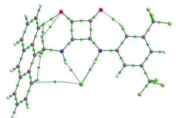
3-Cl -
