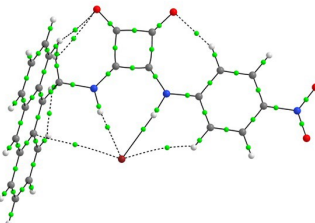
4-Br
