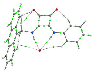
1-Br
