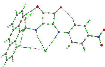
4-Cl -
