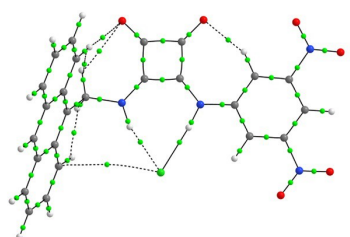
5-Cl -
