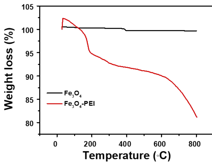
Fig. SI 1 Thermogravimetric analysis of hydrothermally synthesised Fe 3 O 4 and Fe 3 O 4 -PEI nanocomposite.
