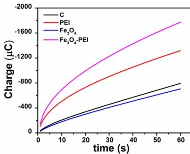
Fig. SI 2 Chronocoulometry for C, Fe 3 O 4 NPs, PEI and Fe 3 O 4 -PEI nanocomposite in 5 mM K 3 [Fe (CN) 6 ] 3- in 0.1 M KNO 3 solution.
