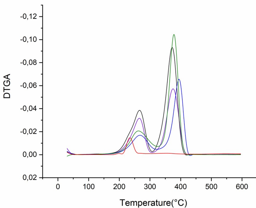
Figure SM1: Thermogravimetric curves and derived thermogravimetric curves (DTGA), of 8HQ-Pt compound, NLC A , (8HQ-Pt)-NLC A , NLC B and (8HQ-Pt)-NLC B nanoparticles.
