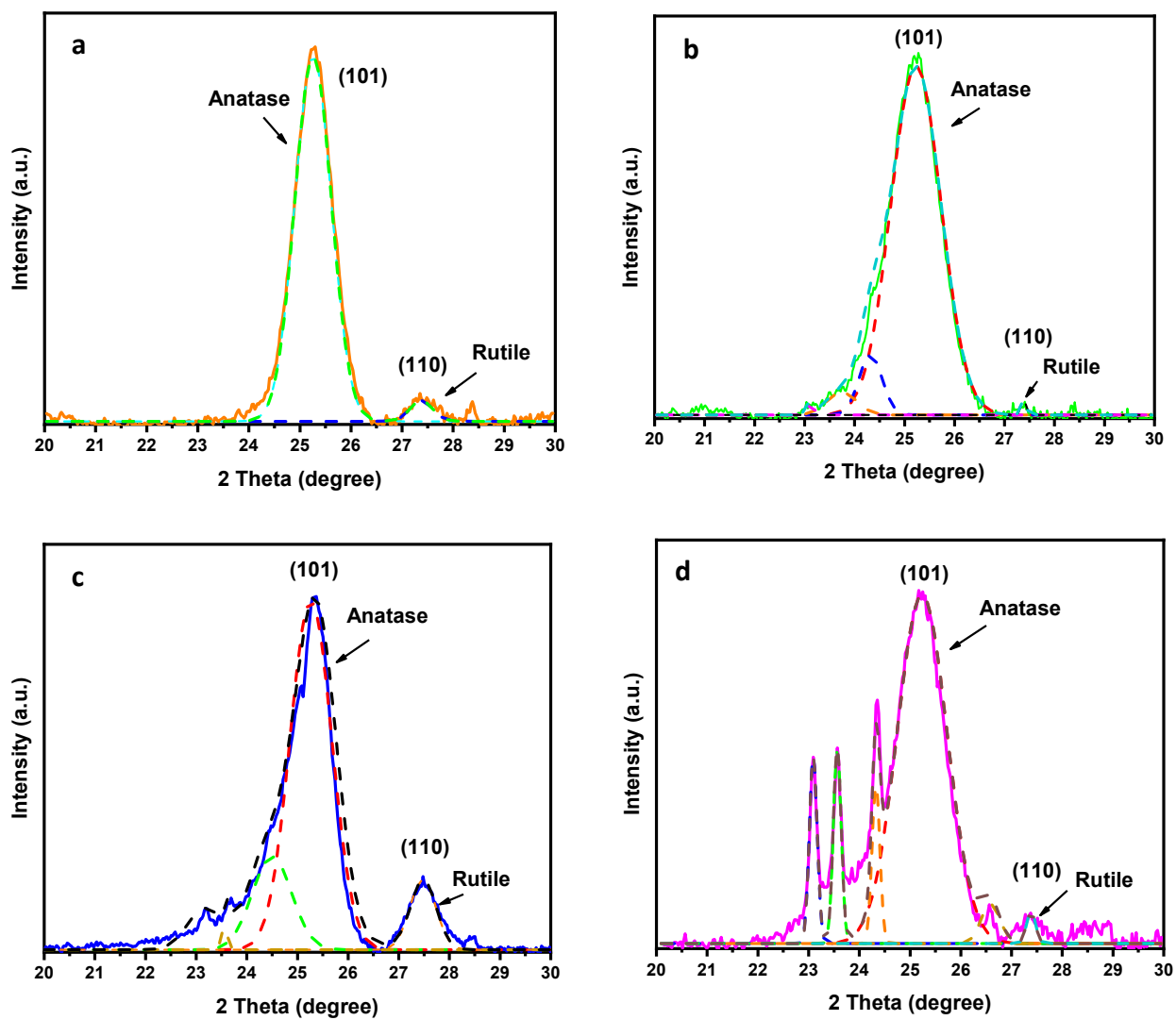
Fig. S1. The anatase (101) and rutile (110) peaks for a) G:TiO 2 , b) G:TiO 2 /WO 3 (90:10), c) G:TiO 2 /WO 3 (80:20), and d) G:TiO 2 /WO 3 (70:30).
