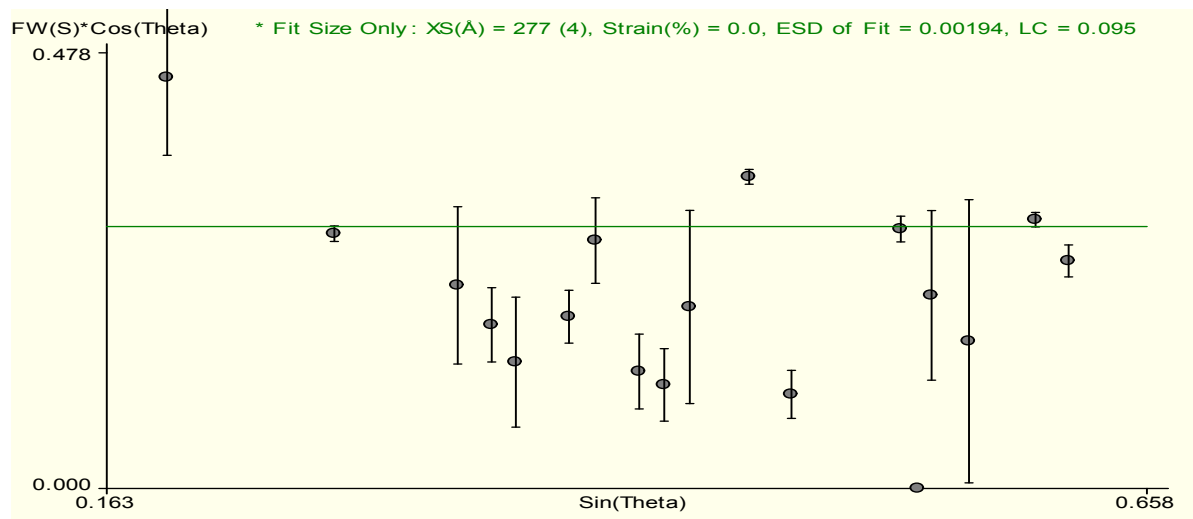
Figure S1: Size calculation using Williamson Hull Equation.
