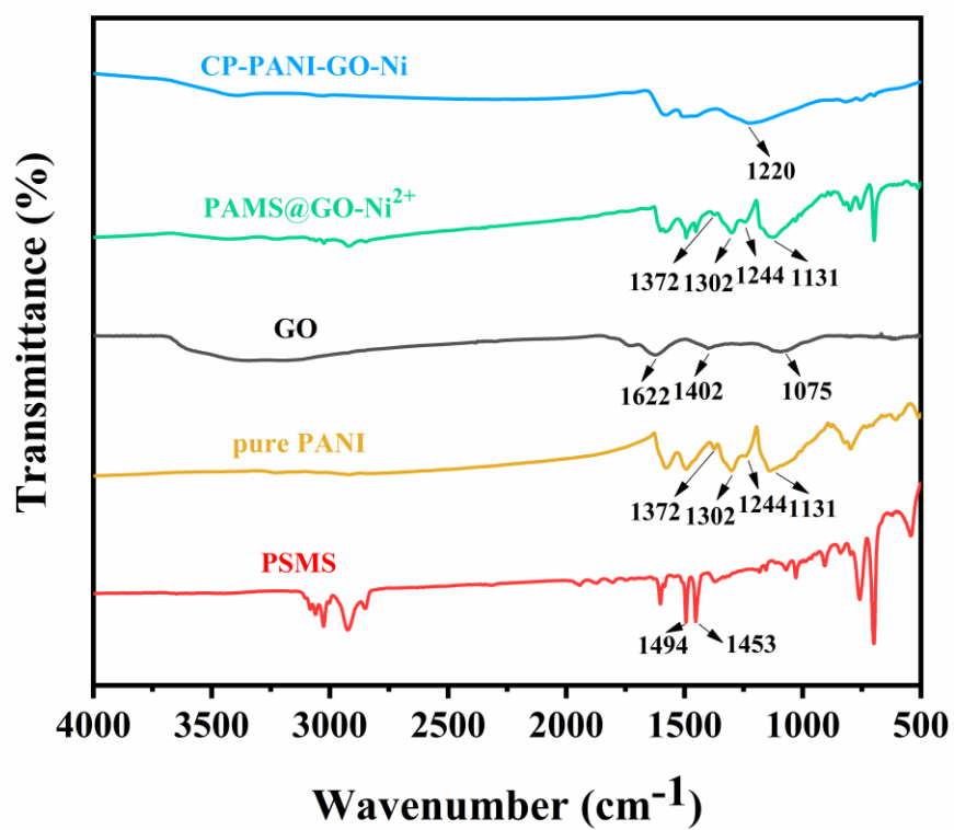
Figure S1. FT-IR spectra of the PSMS, PANI, GO, PAMS@GO-Ni 2+ , and CP-PANI-GO-Ni.
