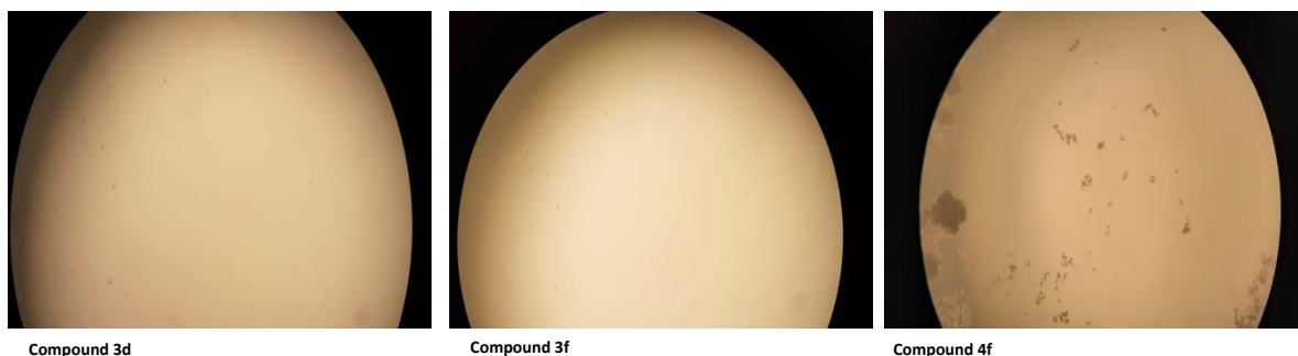
Figure S1 Compound 3d (no live cells), 3f (no live cells), and 4f (minimal cells) nucleoid morphology of Mycobacterium tuberculosis with Fluorescent micrograph.
