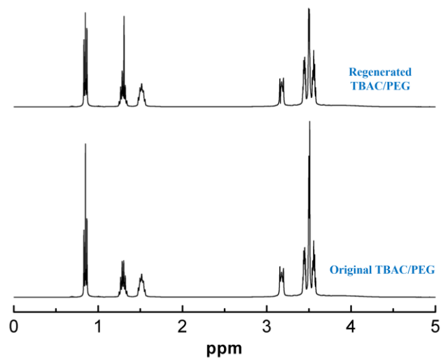
Fig. S1 1 H NMR spectra of original and regenerated TBAC/PEG.
