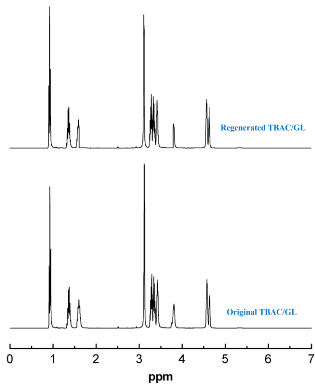
Fig. S3 ^1\text{H} NMR spectra of original and regenerated TBAC/GL.
