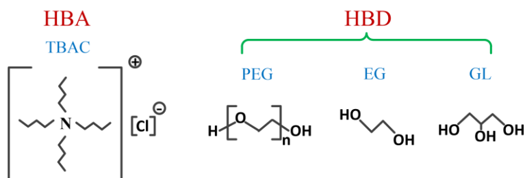
Scheme S1 Molecular structure of HBA (TBAC) and HBD (PEG, EG and GL).
