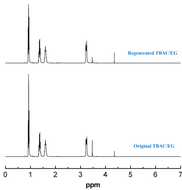
Fig. S2 1 H NMR spectra of original and regenerated TBAC/EG.
