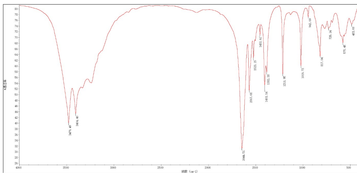
Figure S4 IR spectrum of [\text{Sr}(\text{AFCA})_2(\text{H}_2\text{O})_2] \cdot 2\text{H}_2\text{O}
