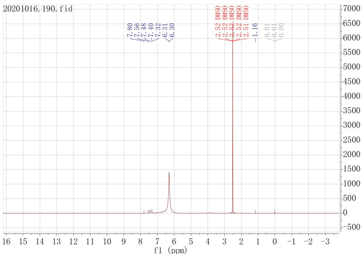
Figure S1 The ^1\text{H} NMR spectrum of 4-aminofurazan-3-carboxylic acid
