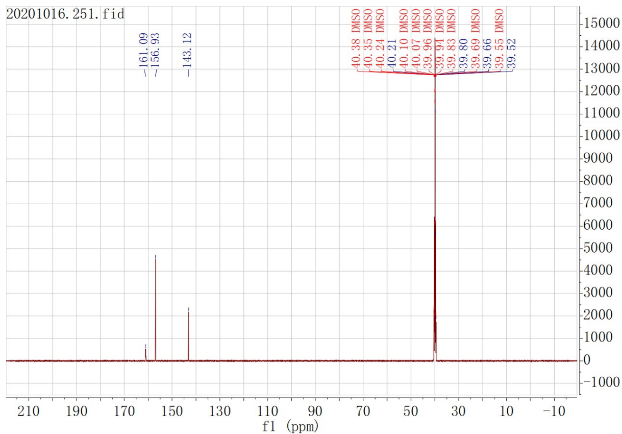
Figure S2 The ^{13}\text{C} NMR spectrum of 4-aminofurazan-3-carboxylic acid
