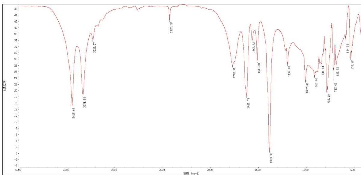
Figure S3 IR spectrum of 4-aminofurazan-3-carboxylic acid
