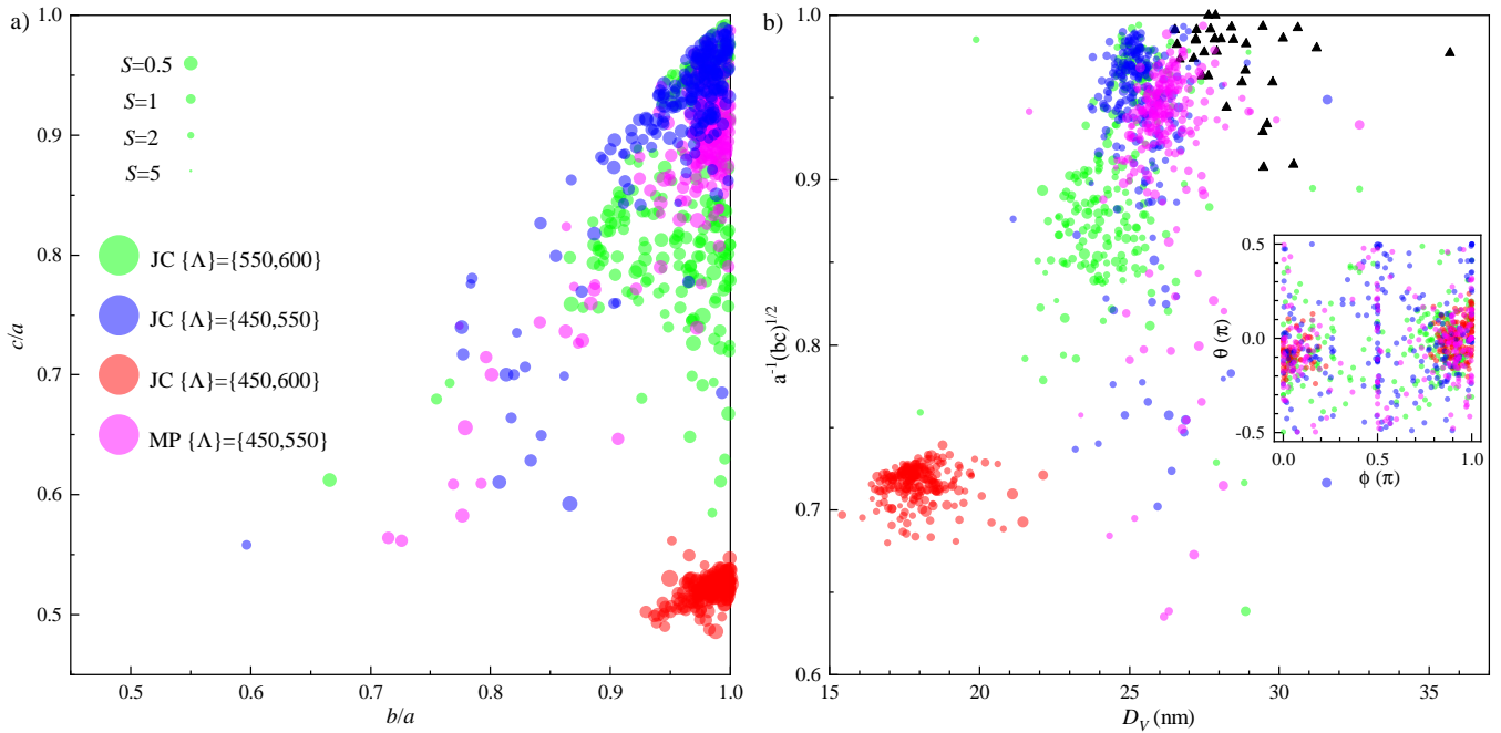
Figure S10. As Fig. 7 a) and b), but using different colour channels and permittivity data as indicated. Johnson & Cristy (JC) [S3] for \{\Lambda\} = \{550, 600\} , \{\Lambda\} = \{450, 550\} , and \{\Lambda\} = \{450, 600\} , as well as McPeak et al. (MP) [S4] for \{\Lambda\} = \{450, 550\} .
