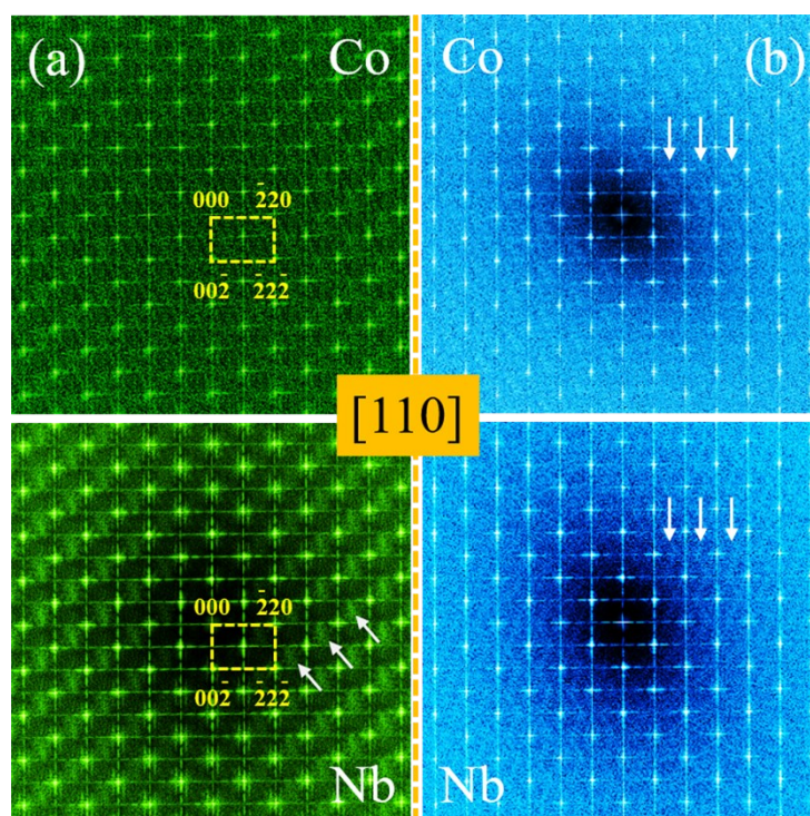
Fig. S2 FFT of the constructed model (a) with actual intensity and ideal atomic position, (b) with actual atomic position and ideal intensity, set to be 1.
