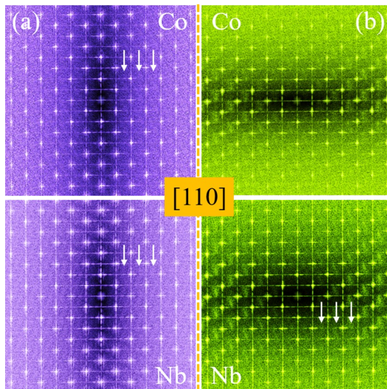
Fig. S3 FFT of the constructed model of Co and Nb, (a) with actual horizontal atomic position and ideal vertical data, (b) with actual vertical atomic position and ideal horizontal data.
