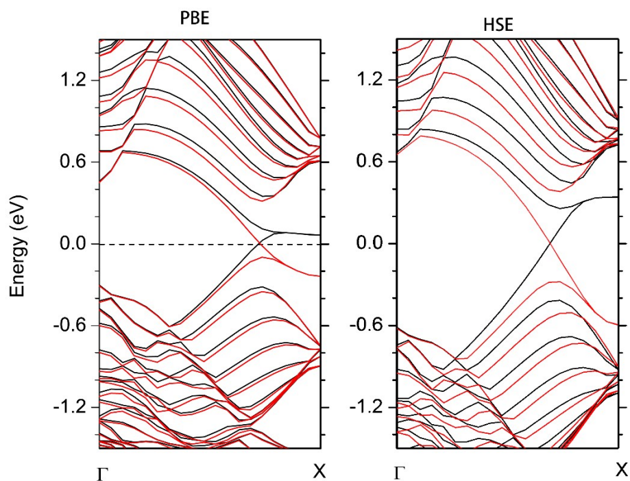
Figure S1. Band structures of stanene zigzag nanoribbon with the edges passivated by H atoms with PBE and HSE calculations.
