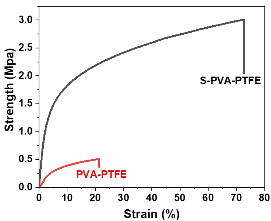
Figure S1. The tensile properties of PVA-PTFE composite membrane and sintered PVA-PTFE composite membrane.
