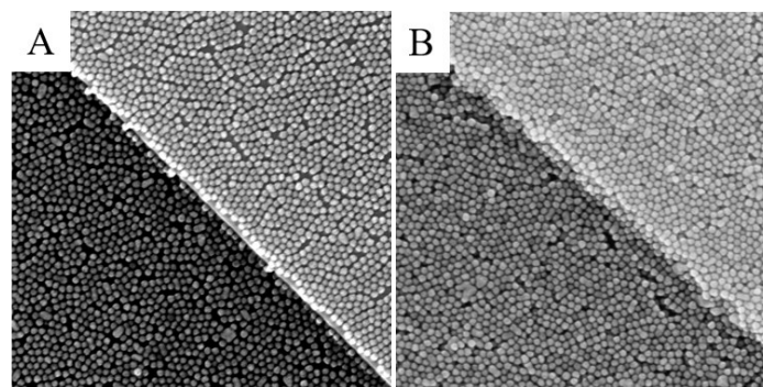
Figure S3 Local enlarged SEM images of Au plate-Au nanoparticles monolayer film coupled system (A) and Au plate-Au nanoparticles bilayer films coupled system (B).
