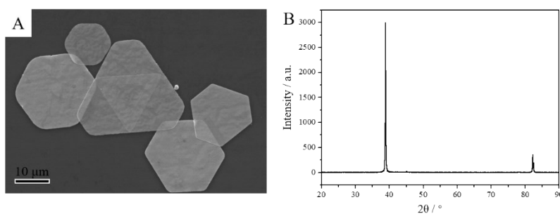
Figure S2 SEM image of Au plates (A). The corresponding XRD characterization (B).
