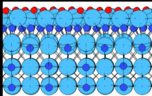
Oxygenated HfN[200]
