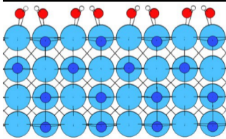
Hydroxylated HfN[200]
