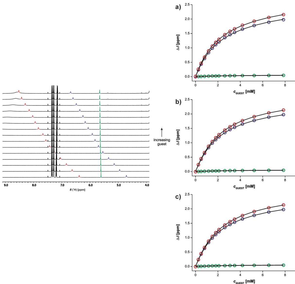
Figure S14. ^1\text{H} NMR (500 MHz, \text{CDCl}_3 , 298 K) titration of bC into P' (0.65 mM). ^1\text{H} NMR spectrum is shown on the left (pyrimidine C-H signal green, N-H signals blue and red). On the right are shown the experimental data (circles) and calculated values (lines) based on a 1:2 binding isotherms using (a) non-cooperative model using identical binding sites, (b) non-cooperative model where K_1 and K_2 were fixed to be the appropriate K_{\text{ref}} and (c) cooperative isotherm where K_1 was fixed to be the appropriate K_{\text{ref}} .
