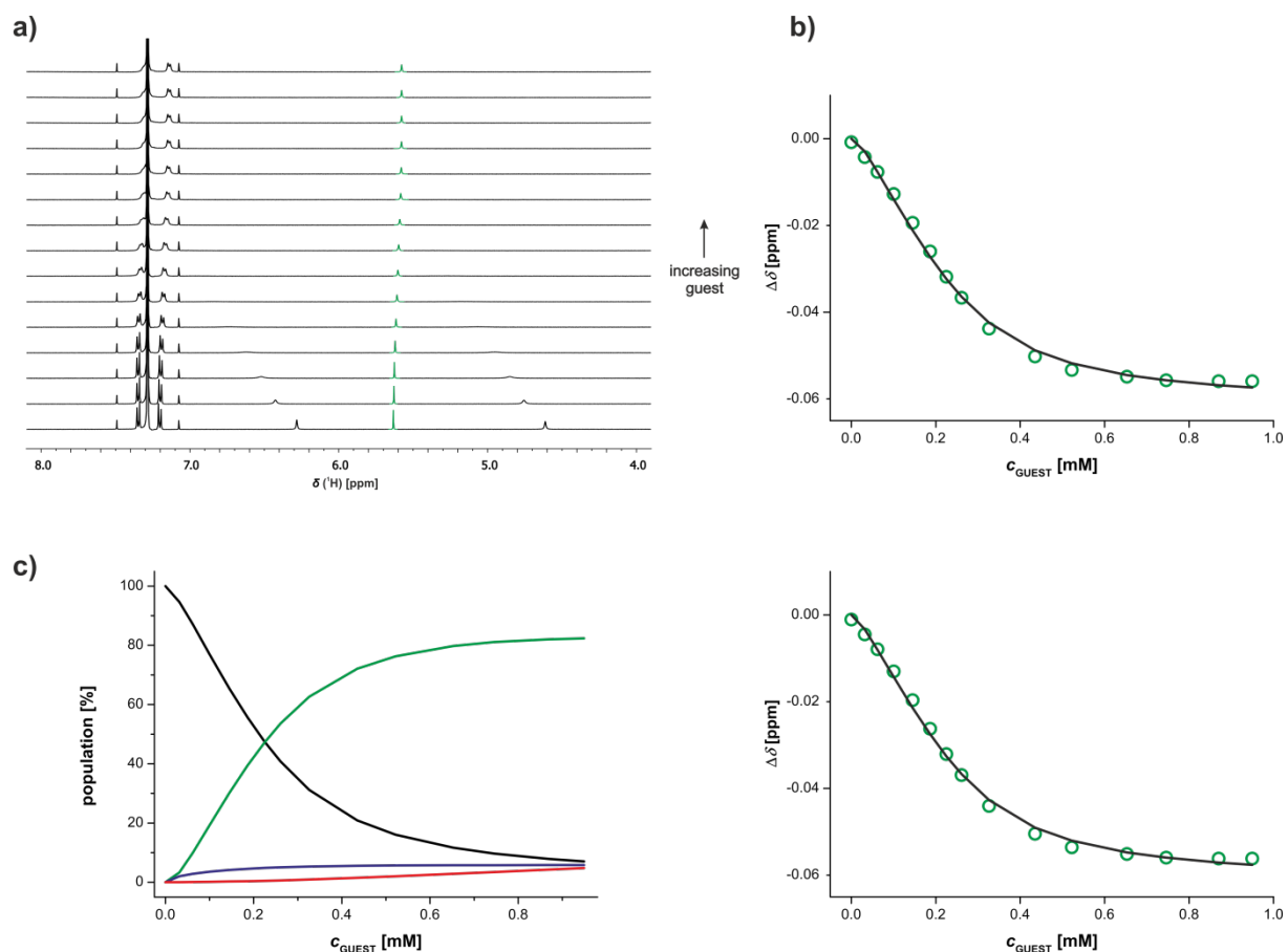
Figure S19. Titration of C into P' (0.26 mM). (a) ^1\text{H} NMR (500 MHz, \text{CDCl}_3 , 298 K) spectrum (pyrimidine C-H signal green). (b) Fitting with an all-or-nothing 3:3 binding isotherm: experimental data (circles) and calculated values (line). (c) Fitting with a 3:3 binding isotherm allowing opening to 1:2 complexes. Fitting is on the right and the distribution diagram on the left ( P' black, P' 3 • C 3 green, P' • C blue and P' • C 2 red).
