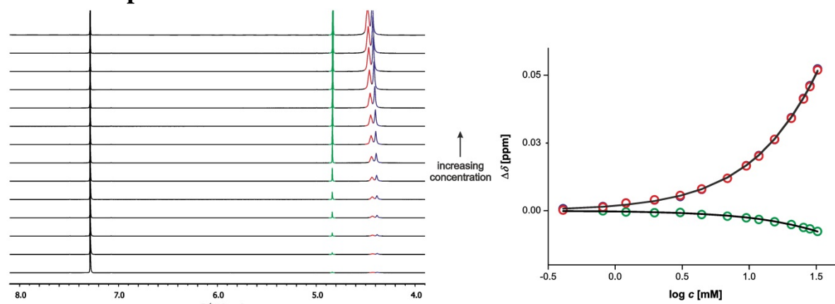
Figure S5. ^1\text{H} NMR (500 MHz, \text{CDCl}_3 , 298 K) dilution experiments for P . The ^1\text{H} NMR spectra are shown on the left (pyrimidine C-H signal green, N-H signals blue and red). On the right are shown the experimental data (circles) and calculated values (lines) based on a dimerisation isotherm.
