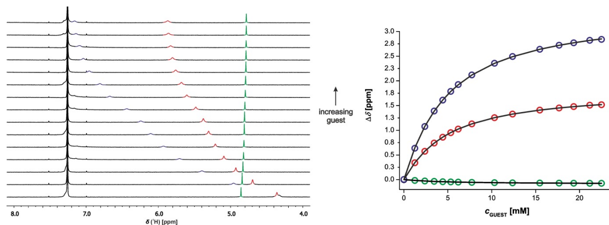
Figure S7. ^1\text{H} NMR (400 MHz, \text{CDCl}_3 , 298 K) titration of bB into bP (1.4 mM). ^1\text{H} NMR spectrum is shown on the left (pyrimidine C-H signal green, N-H signals blue and red). On the right are shown the experimental data (circles) and calculated values (lines) based on a 1:1 binding isotherm.
