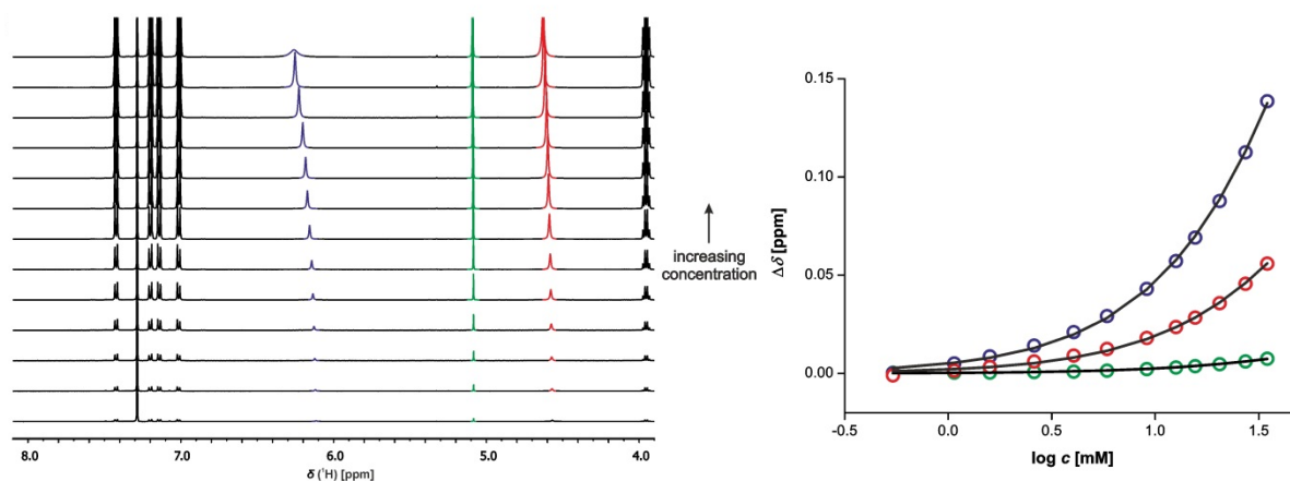
Figure S6. ^1\text{H} NMR (500 MHz, \text{CDCl}_3 , 298 K) dilution experiments for bP' . The ^1\text{H} NMR spectra are shown on the left (pyrimidine C-H signal green, N-H signals blue and red). On the right are shown the experimental data (circles) and calculated values (lines) based on a dimerisation isotherm.
