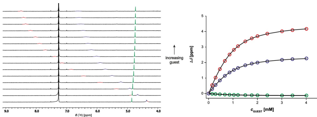
Figure S9. ^1\text{H} NMR (400 MHz, \text{CDCl}_3 , 298 K) titration of bC into bP (0.86 mM). ^1\text{H} NMR spectrum is shown on the left (pyrimidine C-H signal green, N-H signals blue and red). On the right are shown the experimental data (circles) and calculated values (lines) based on a 1:1 binding isotherm.
