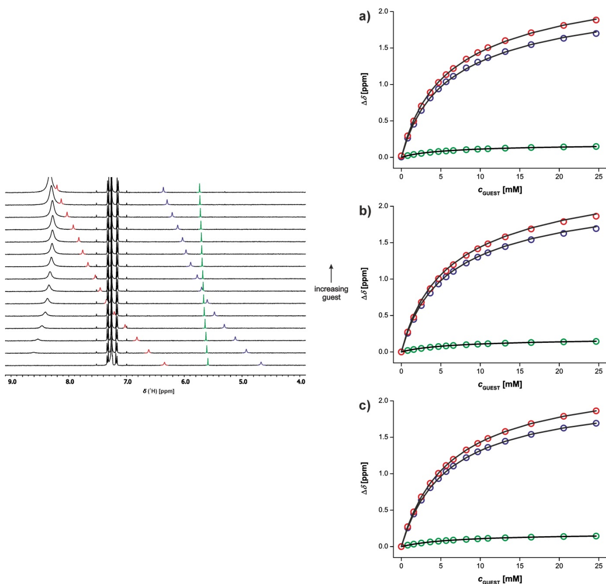
Figure S12. ^1\text{H} NMR (400 MHz, \text{CDCl}_3 , 298 K) titration of bB into P' (0.53 mM). ^1\text{H} NMR spectrum is shown on the left (pyrimidine C-H signal green, N-H signals blue and red). On the right are shown the experimental data (circles) and calculated values (lines) based on a 1:2 binding isotherms using (a) non-cooperative model using identical binding sites, (b) non-cooperative model where K_1 and K_2 were fixed to be the appropriate K_{\text{ref}} and (c) cooperative isotherm where K_1 was fixed to be the appropriate K_{\text{ref}} .
