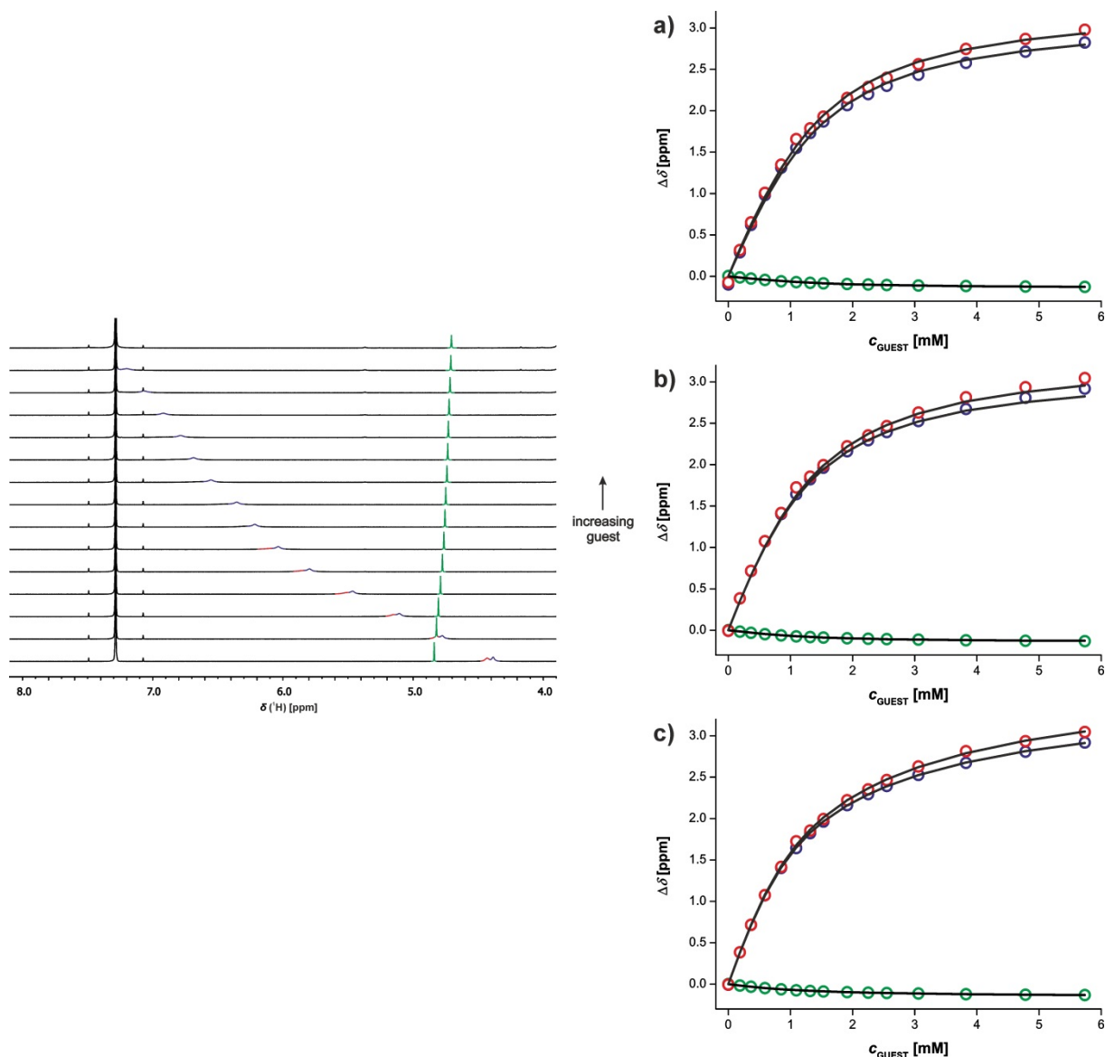
Figure S13. ^1\text{H} NMR (500 MHz, \text{CDCl}_3 , 298 K) titration of bC into P (0.77 mM). ^1\text{H} NMR spectrum is shown on the left (pyrimidine C-H signal green, N-H signals blue and red). On the right are shown the experimental data (circles) and calculated values (lines) based on a 1:2 binding isotherms using (a) non-cooperative model using identical binding sites, (b) non-cooperative model where K_1 and K_2 were fixed to be the appropriate K_{\text{ref}} and (c) cooperative isotherm where K_1 was fixed to be the appropriate K_{\text{ref}} .
