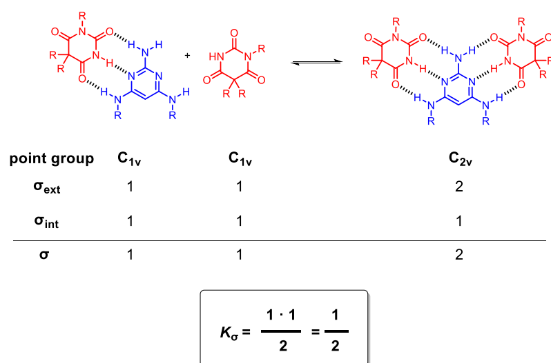
Figure S21. Determination of the statistical factors for the reference 1:2 systems. The statistical factors are identical for the corresponding system based on a barbiturate and blocked-pyrimidines. The statistical factor derived above for the barbiturates can also be applied to the cyanurates thanks to their analogous symmetry
