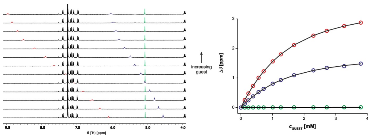
Figure S10. ^1\text{H} NMR (400 MHz, \text{CDCl}_3 , 298 K) titration of bC into bP' (0.83 mM). ^1\text{H} NMR spectrum is shown on the left (pyrimidine C-H signal green, N-H signals blue and red). On the right are shown the experimental data (circles) and calculated values (lines) based on a 1:1 binding isotherm.
