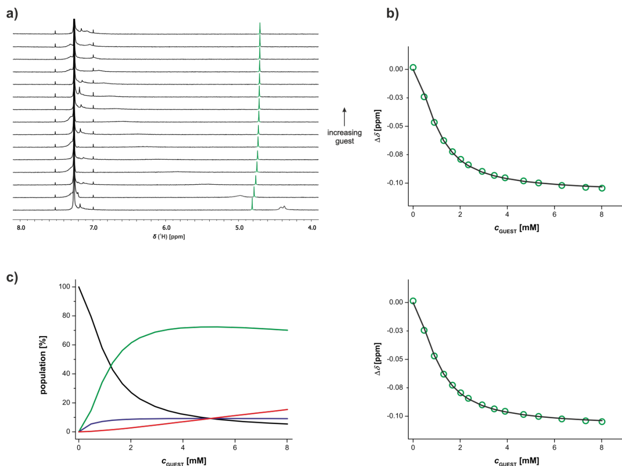
Figure S16. Titration of B into P (0.88 mM). (a) ^1\text{H} NMR (400 MHz, \text{CDCl}_3 , 298 K) spectrum (pyrimidine C-H signal green). (b) Fitting with an all-or-nothing 3:3 binding isotherm: experimental data (circles) and calculated values (line). (c) Fitting with a 3:3 binding isotherm allowing opening to 1:2 complexes. Fitting is on the right and the distribution diagram on the left ( P black, P 3 ·B 3 green, P·B blue and P·B 2 red).
