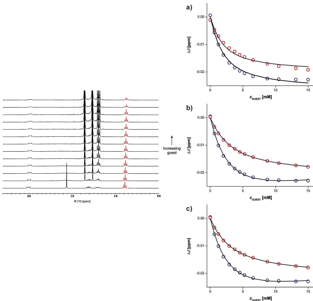
Figure S15. ^1\text{H} NMR (500 MHz, \text{CDCl}_3 , 298 K) titration of bP' into B (0.90 mM). ^1\text{H} NMR spectrum is shown on the left ( \text{CH}_3 signal red, (\text{C}=\text{O})_2\text{C}(\text{CH}_2)_2 signal blue). On the right are shown the experimental data (circles) and calculated values (lines) based on a 1:2 binding isotherms using (a) non-cooperative model using identical binding sites, (b) non-cooperative model where K_1 and K_2 were fixed to be the appropriate K_{\text{ref}} and (c) cooperative isotherm where K_1 was fixed to be the appropriate K_{\text{ref}} .
