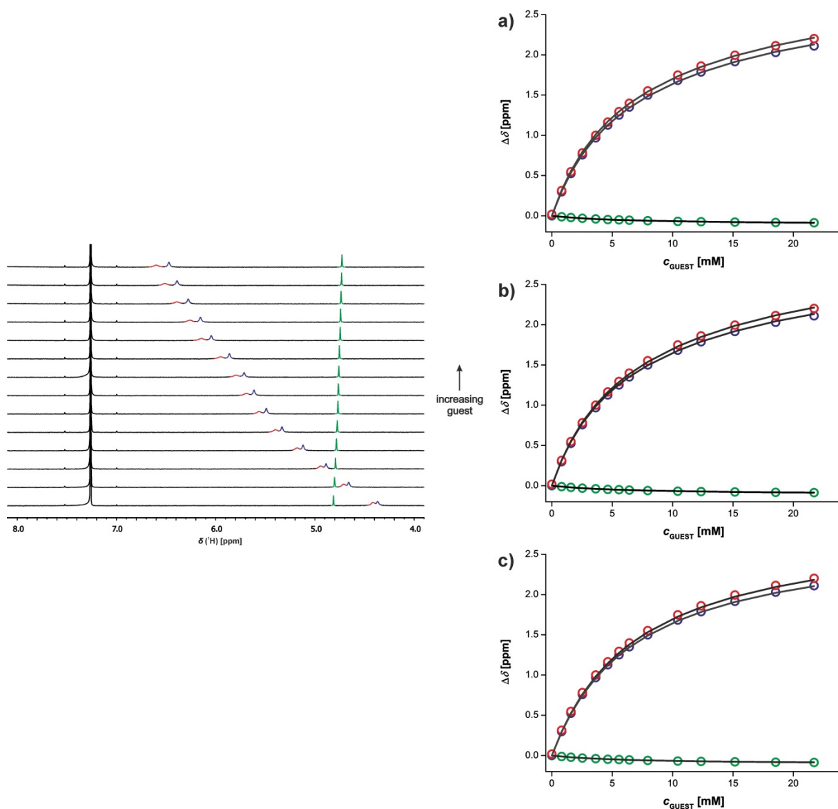
Figure S11. ^1\text{H} NMR (400 MHz, \text{CDCl}_3 , 298 K) titration of bB into P (0.99 mM). ^1\text{H} NMR spectrum is shown on the left (pyrimidine C-H signal green, N-H signals blue and red). On the right are shown the experimental data (circles) and calculated values (lines) based on a 1:2 binding isotherms using (a) non-cooperative model using identical binding sites, (b) non-cooperative model where K_1 and K_2 were fixed to be the appropriate K_{\text{ref}} and (c) cooperative isotherm where K_1 was fixed to be the appropriate K_{\text{ref}} .
