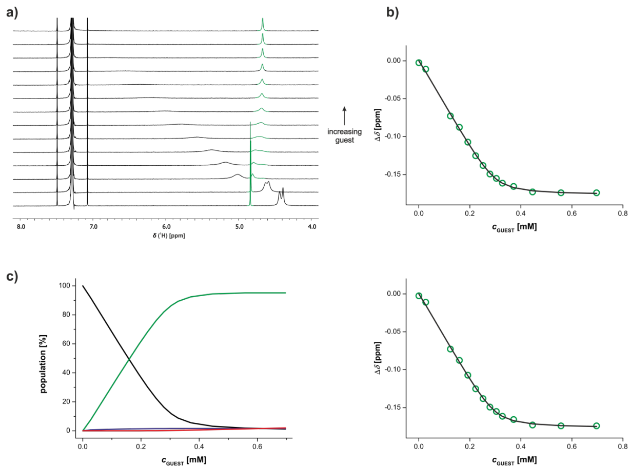
Figure S18. Titration of C into P (0.30 mM). (a) ^1\text{H} NMR (500 MHz, \text{CDCl}_3 , 298 K) spectrum (pyrimidine C-H signal green). (b) Fitting with an all-or-nothing 3:3 binding isotherm: experimental data (circles) and calculated values (line). The weight averaging was used to obtain the average chemical shift of pyrimidine C-H signal. (c) Fitting with a 3:3 binding isotherm allowing opening to 1:2 complexes. Fitting is on the right and the distribution diagram on the left ( P black, \text{P}_3\cdot\text{C}_3 green, \text{P}\cdot\text{C} blue and \text{P}\cdot\text{C}_2 red).
