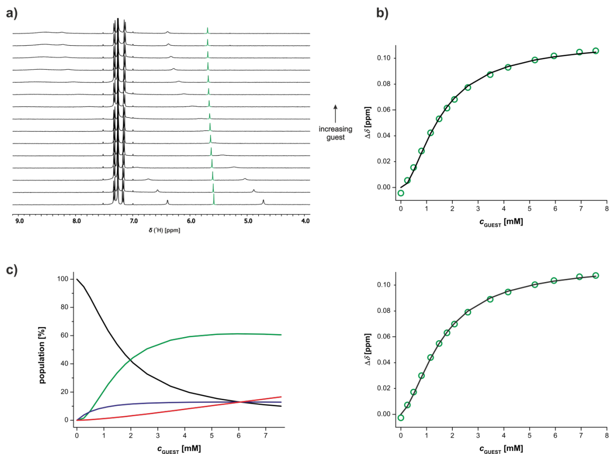
Figure S17. Titration of B into P' (1.1 mM). (a) ^1\text{H} NMR (400 MHz, \text{CDCl}_3 , 298 K) spectrum (pyrimidine C-H signal green). (b) Fitting with an all-or-nothing 3:3 binding isotherm: experimental data (circles) and calculated values (line). (c) Fitting with a 3:3 binding isotherm allowing opening to 1:2 complexes. Fitting is on the right and the distribution diagram on the left ( P' black, P' 3 B 3 green, P'•B blue and P'•B 2 red).
