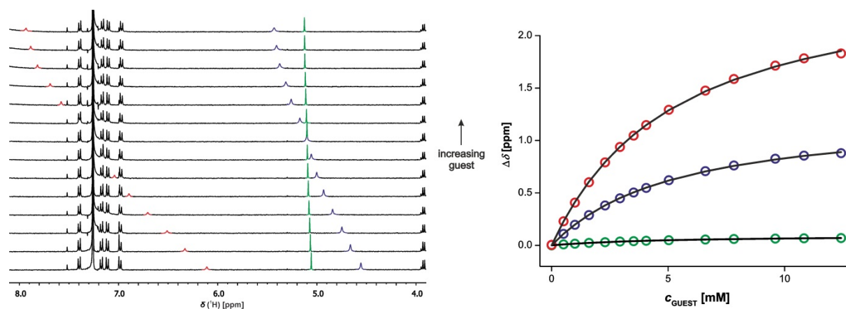
Figure S8. ^1\text{H} NMR (400 MHz, \text{CDCl}_3 , 298 K) titration of bB into bP' (0.53 mM). ^1\text{H} NMR spectrum is shown on the left (pyrimidine C-H signal green, N-H signals blue and red). On the right are shown the experimental data (circles) and calculated values (lines) based on a 1:1 binding isotherm.
