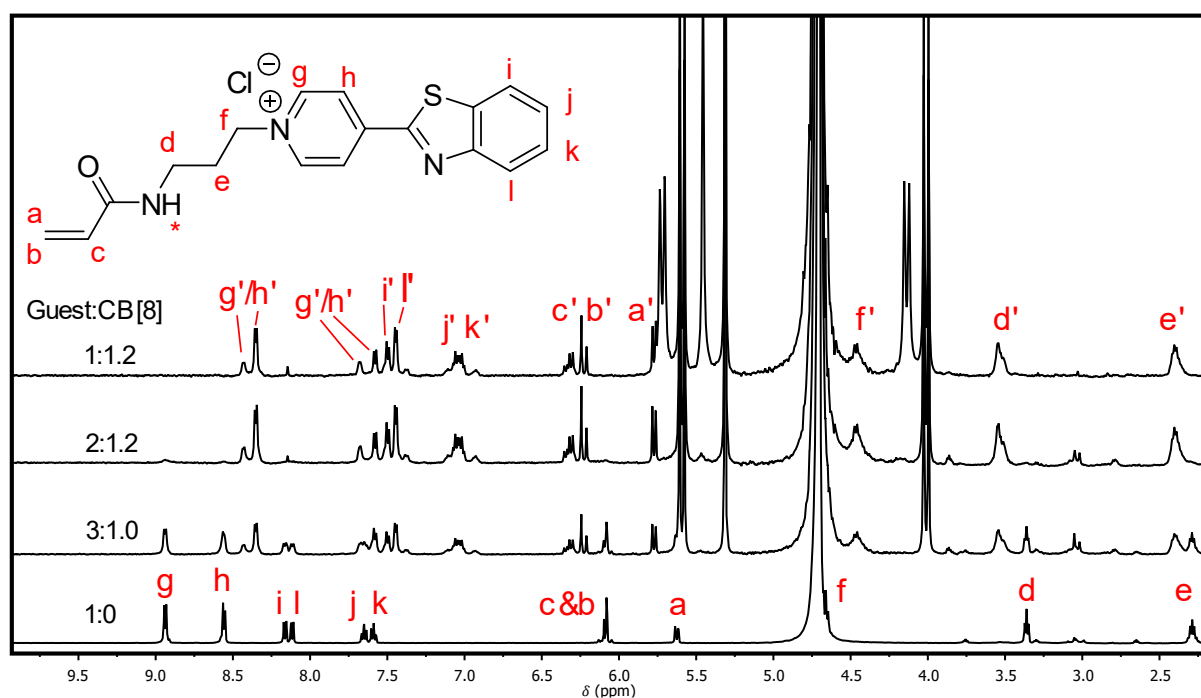
Figure S 7: Titration of BTPyPrAm into CB[8] monitored using ^1\text{H} NMR spectroscopy and showing upfield shifts for \text{H}_g\text{-H}_i and downfield shifts for \text{H}_a\text{-H}_f .
