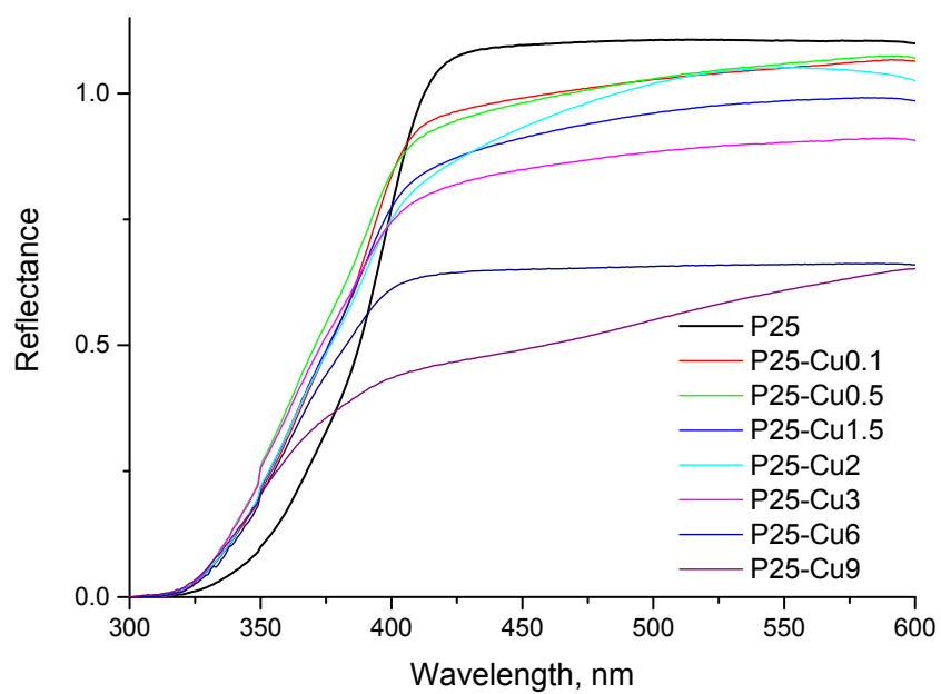
Figure S2. UV-Vis Diffuse Reflectance spectra of P25 and of the studied Cu-containing catalysts supported on P25.
