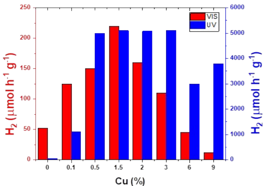
Figure S1. Hydrogen production ( \mu\text{mol h}^{-1} \text{g}^{-1} ) of P25 and of the studied Cu-containing catalysts supported on P25 under ultraviolet and visible irradiation.
