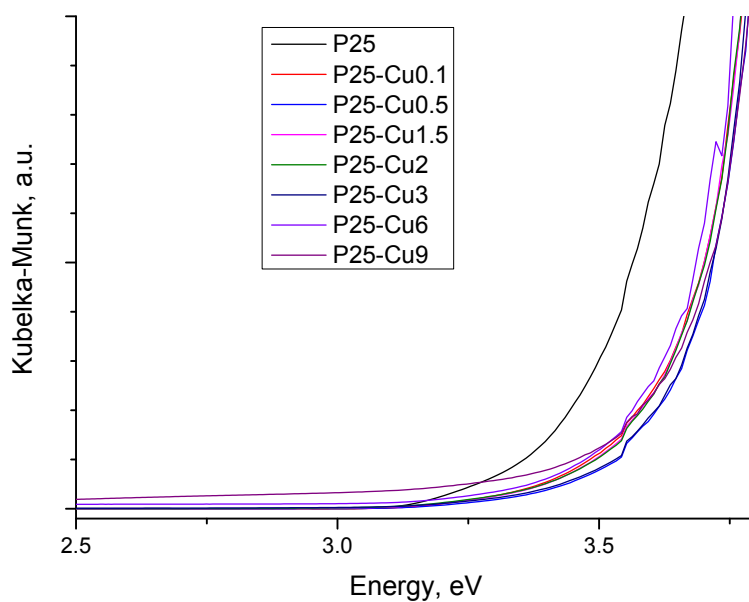
Fig. S3. Kubelka-Munk function for P25 and spectra of P25 and of the studied Cu-containing catalysts supported on P25.
