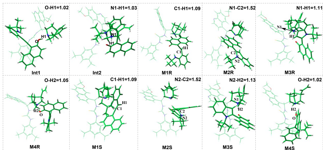
Fig. S2. Optimized geometries of intermediates for the catalytic cycle (Distances are in angstroms).
