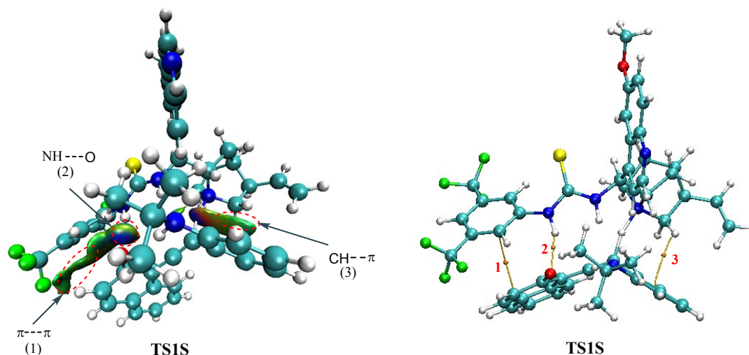
Fig. S1 NCI analysis and topological analysis of bond critical points (BCPs) along the bond paths for the transition state TS1S .
