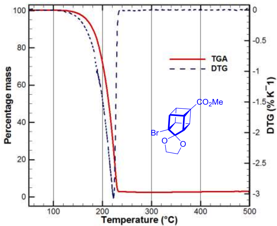
Fig-T10. TGA-DTG of Compound 19 at 15\text{K min}^{-1}
