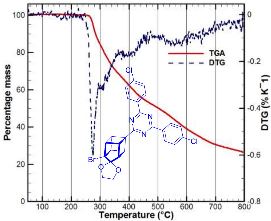
Fig-T16. TGA-DTG of Compound 30b at 15\text{K min}^{-1}
