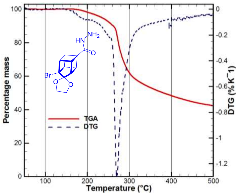
Fig-T12. TGA-DTG of Compound 25 at 15K min -1
