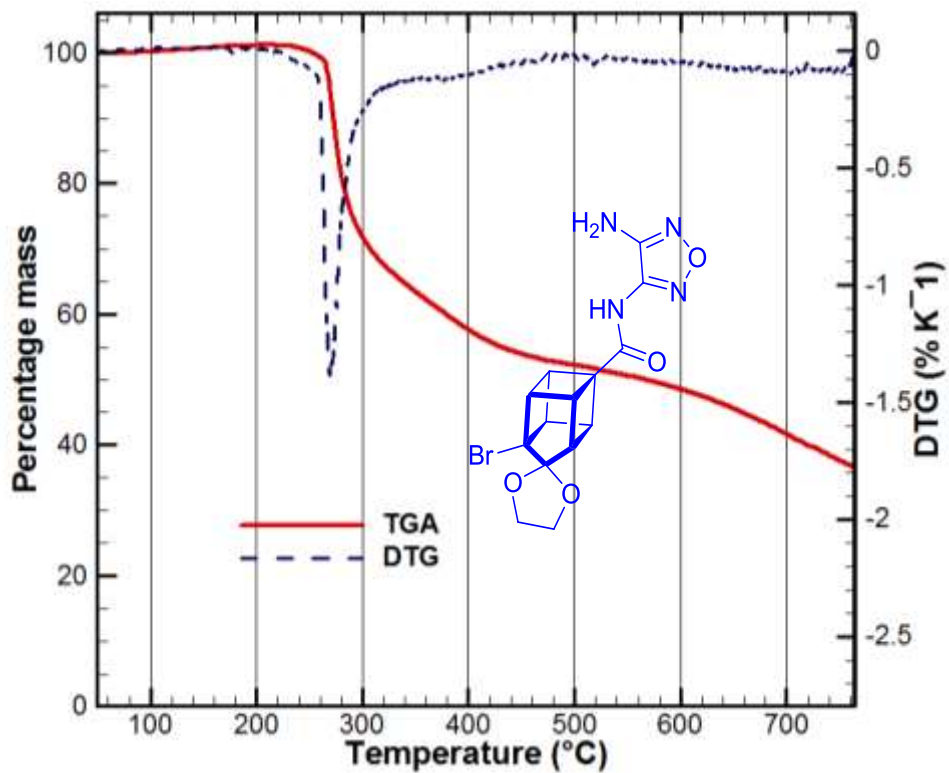
Fig-T13. TGA-DTG of compound 27 at 15K min -1
