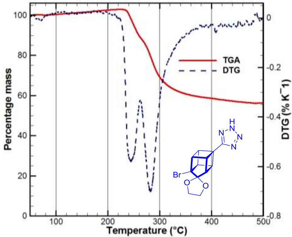
Fig-T8. TGA-DTG of Compound 15 at 15\text{K min}^{-1}
