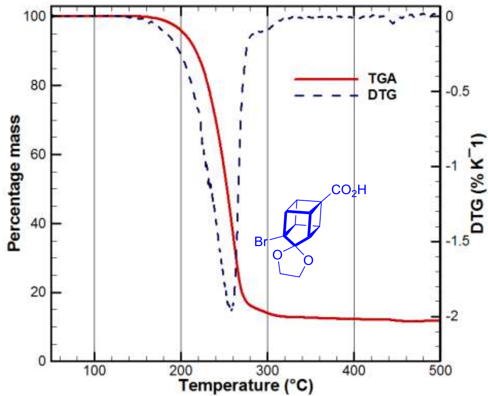
Fig-T1. TGA-DTG of Compound 8 at 15\text{K min}^{-1}
