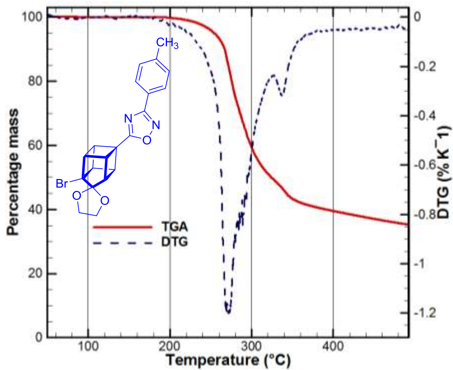
Fig-T11. TGA-DTG of compound 21a at 15K min -1
