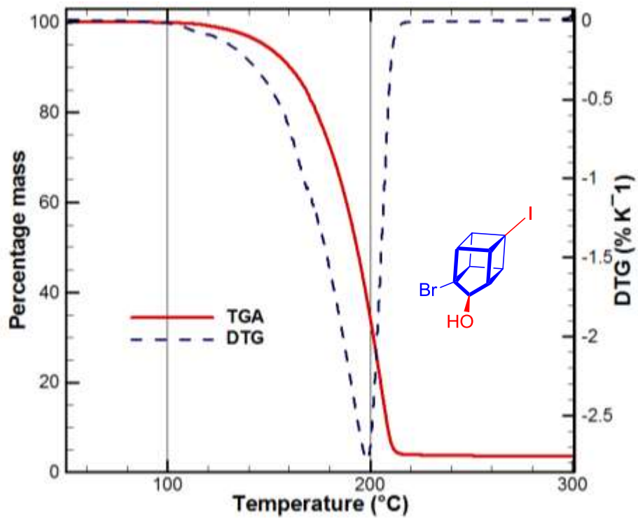
Fig-T5. TGA-DTG of Compound 12 at 15K min -1
