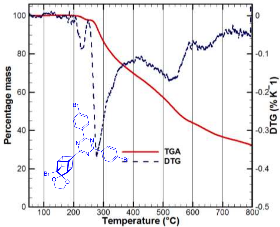
Fig-T17. TGA-DTG of Compound 30c at 15K min -1
