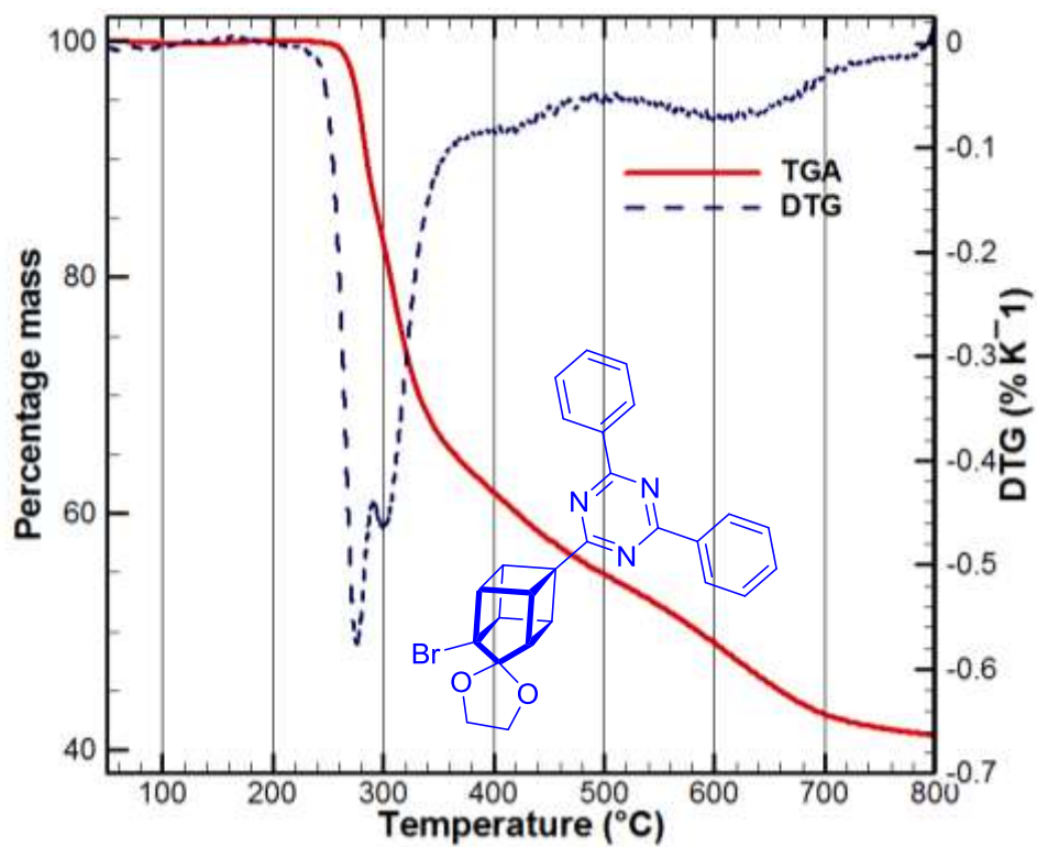
Fig-T15. TGA-DTG of Compound 30a at 15\text{K min}^{-1}
