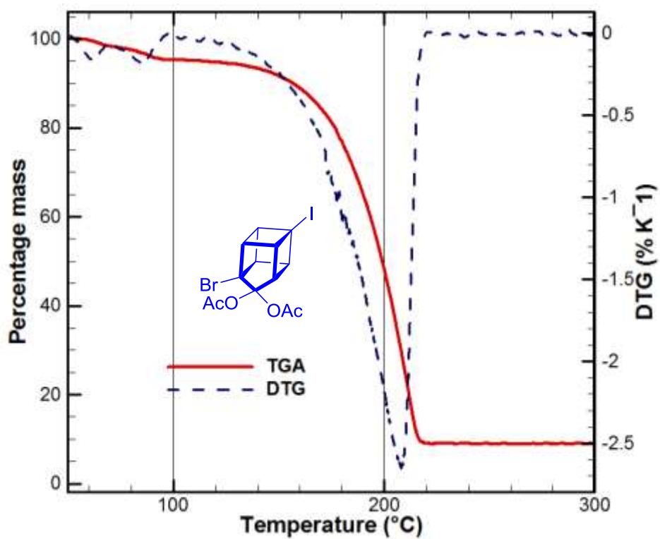
Fig-T3. TGA-DTG of compound 10 at 15K min -1
