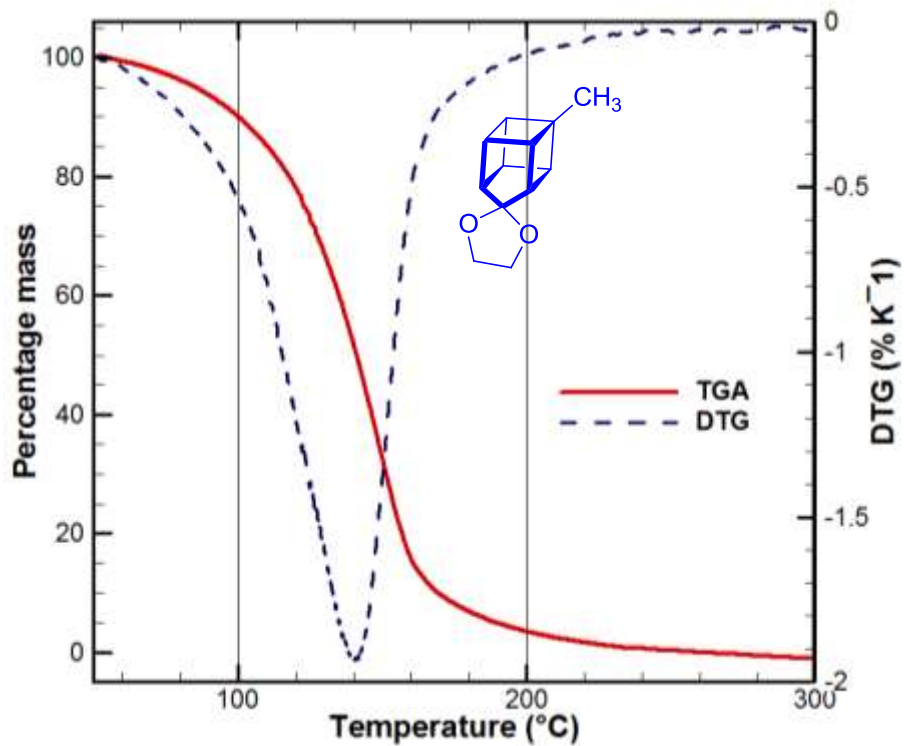
Fig-T9. TGA-DTG of Compound 18 at 15\text{K min}^{-1}
