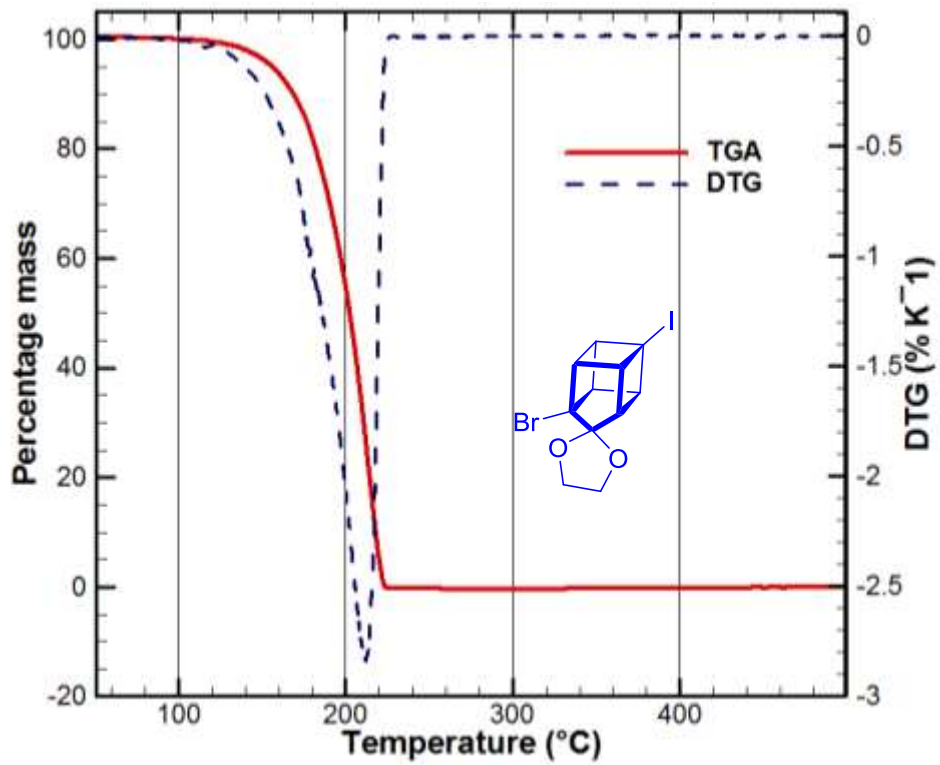
Fig-T2. TGA-DTG of compound 9 at 15\text{K min}^{-1}
