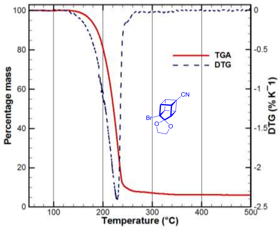
Fig-T7. TGA-DTG of Compound 14 at 15\text{K min}^{-1}
