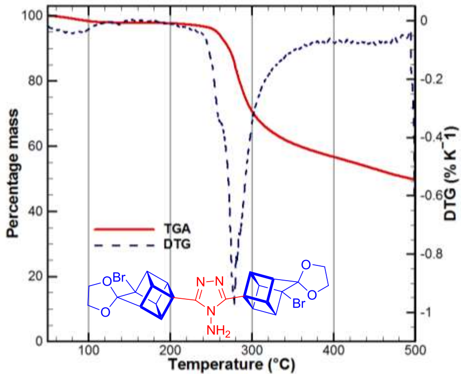
Fig-T14. TGA-DTG of Compound 28 at 15K min -1
