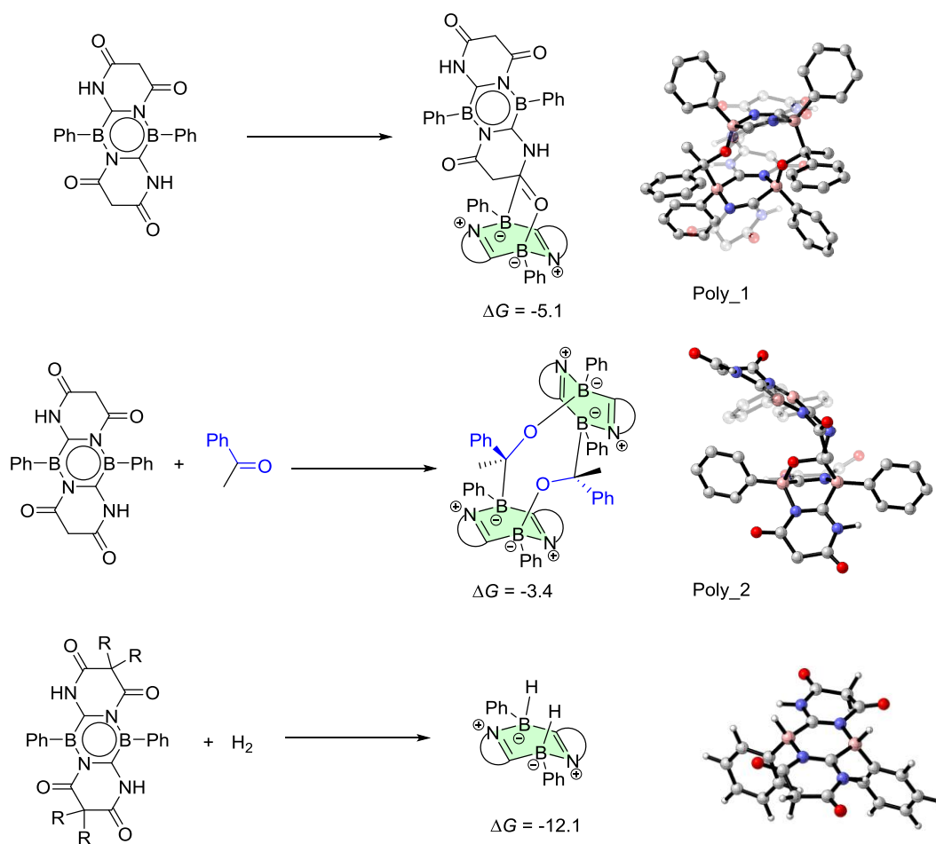
Figure S2. The thermodynamics of the polymerization of compound B calculated at B3LYP-D3/6-311+(d,p)//B3LYP-D3/6-31(d) level of theory.
