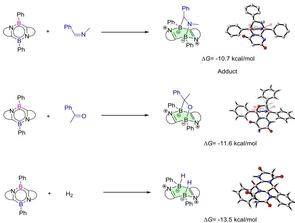
Figure S4. The [4 + 2] cycloaddition reaction of compound B with benzaldehyde and acetophenone.
