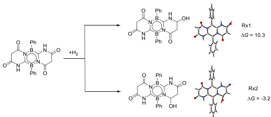
Figure S3. The thermodynamics of the reduction of carbonyl groups in the presence of \text{H}_2 calculated at B3LYP-D3/6-311+(d,p)//B3LYP-D3/6-31(d) level of theory.
