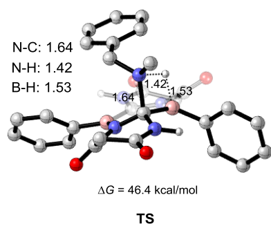
Figure S7. The optimized structure of transition state corresponding for the direct abstract of H 2 starting from IM 2 N.
