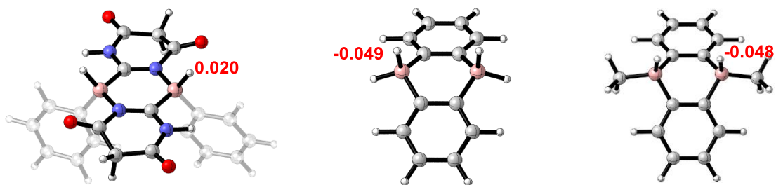
Figure S5. The calculated NPA charge of B-H 2 and [DBA-H 2 ] 2- .
