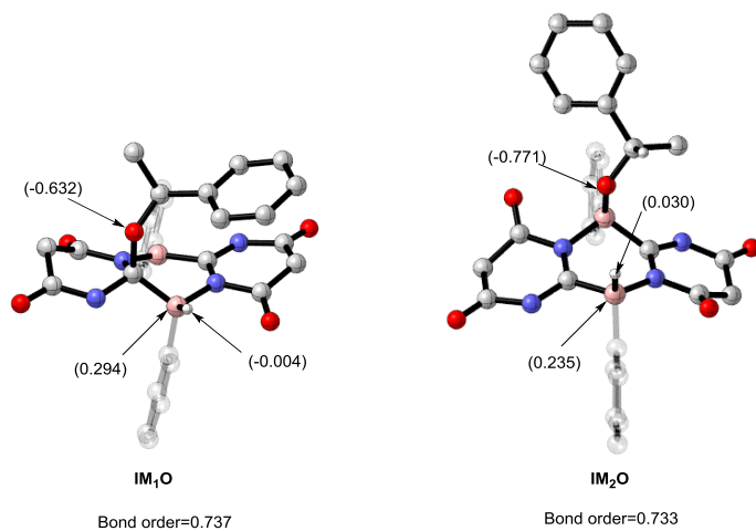
Figure S8. The calculated NPA charge of IM 1 O and IM 2 O.
