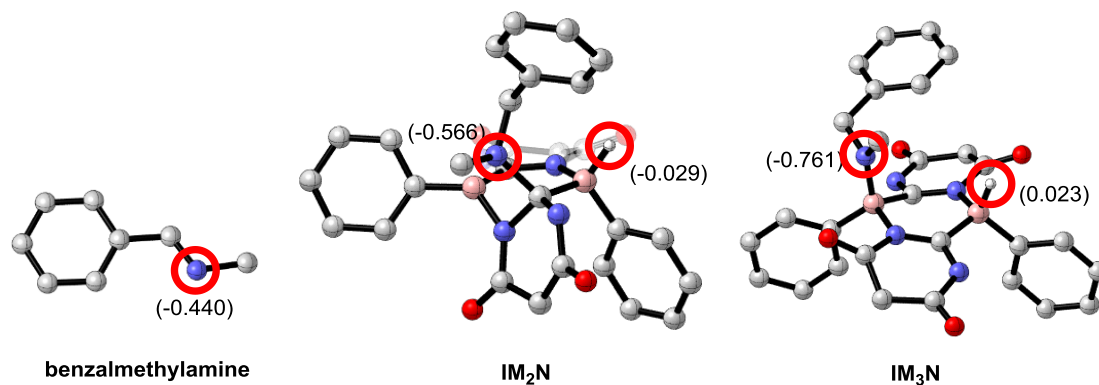
Figure S6. The calculated NPA charge of IM 2 N and IM 3 N.
