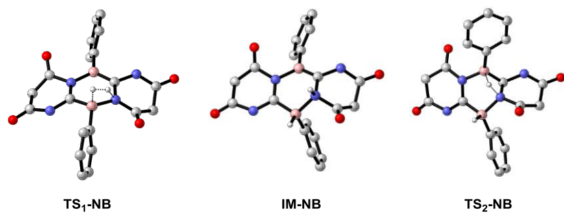
Figure S1. Alternative stepwise mechanism of compound B catalyzed H_2 activation.
