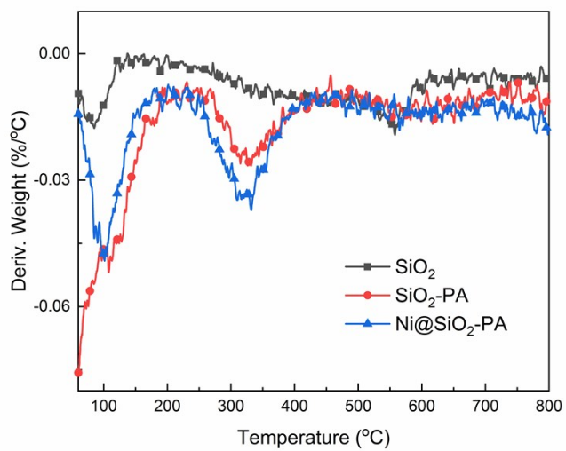
Fig. S1 DTG curves of SiO 2 , SiO 2 -PA and Ni@SiO 2 -PA under N 2 atmosphere.
