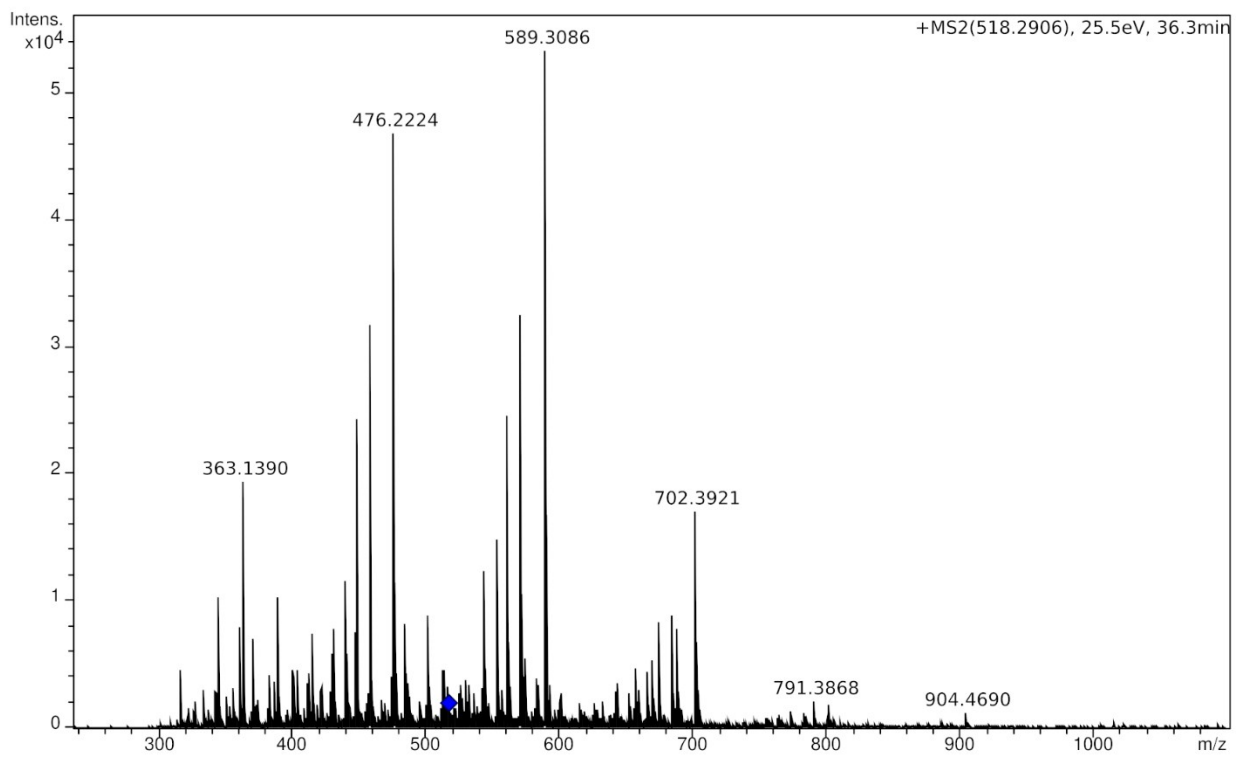
Fig S1. ESI-Q-TOF MS/MS spectrum of (a) m/z 546.7745 identified as ETSGMKPTEL, and (b) m/z 518.2904 identified as ISSMGILVCL.
