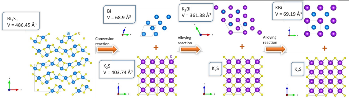
Fig. 4 Electrochemical K storage mechanism of \text{Bi}_2\text{S}_3 in the composite electrode and volume changes. The insets show the detailed crystalline parameters computed in previous reports on LIB and SIBs. 5,16 \text{Bi}_2\text{S}_3 typically undergoes subsequent conversion and alloying reactions during the
