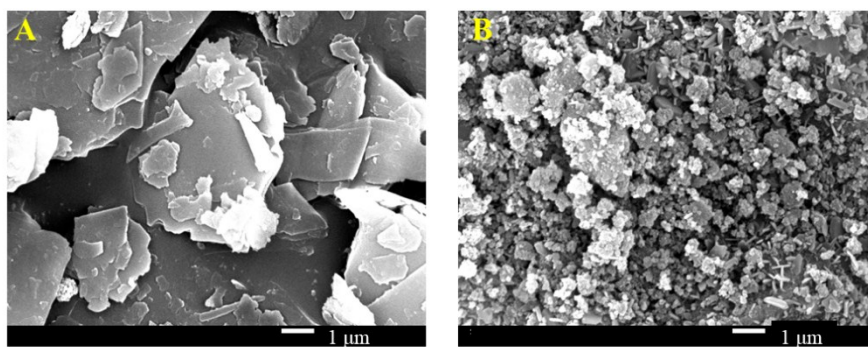
Fig. S-1 SEM images of the raw talc and the D-600 sample
