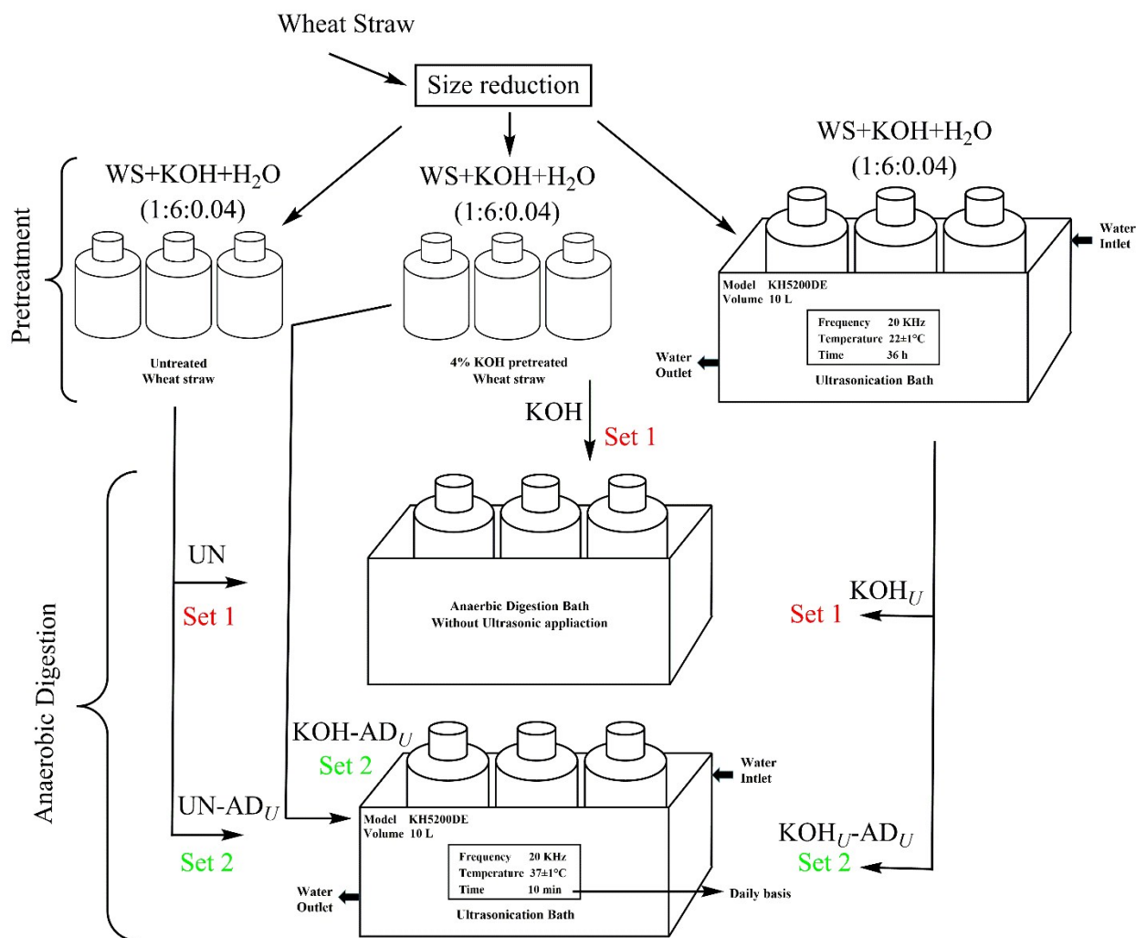
Fig. S1 Experimental design and operating conditions during pretreatment and anaerobic digestion
