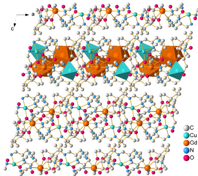
Fig.S2 3D supramolecular framework of 1 .
