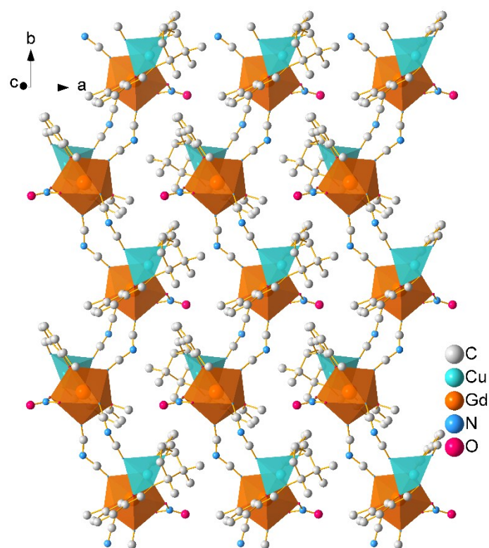
Fig.S1 2D layer of 1 in the ab plane.
