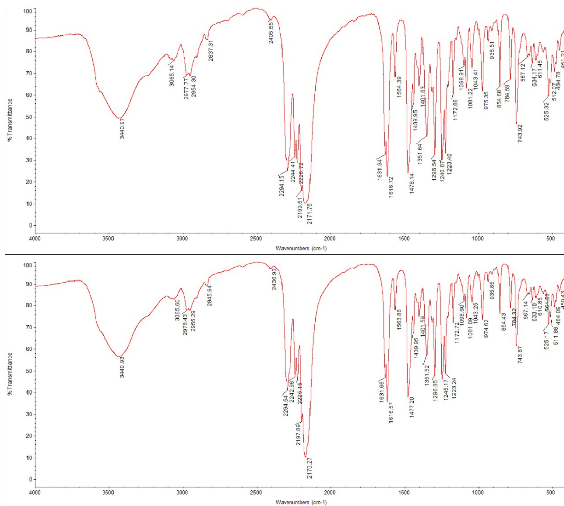
Fig.S3 Infrared spectra of 1 (up) and 2 (down).
