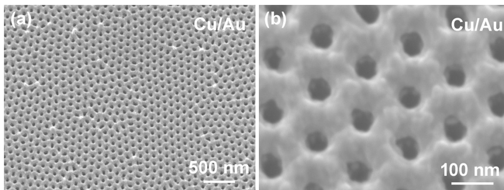
Figure S1 (a) and (b) SEM images of the nanoporous Cu/Au film.
