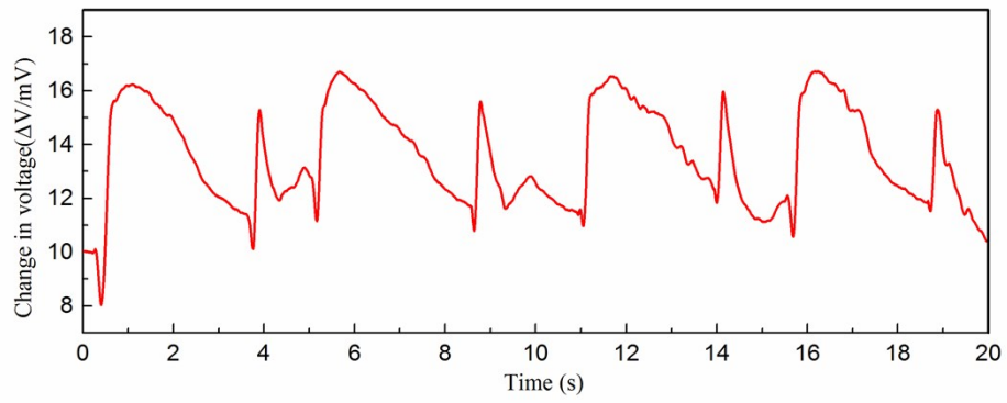
Figure S4 Breathing test of Chinese wine (53% ethanol content)
