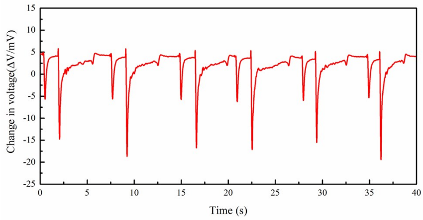
Figure S3 Breathing test of 100% alcohol
