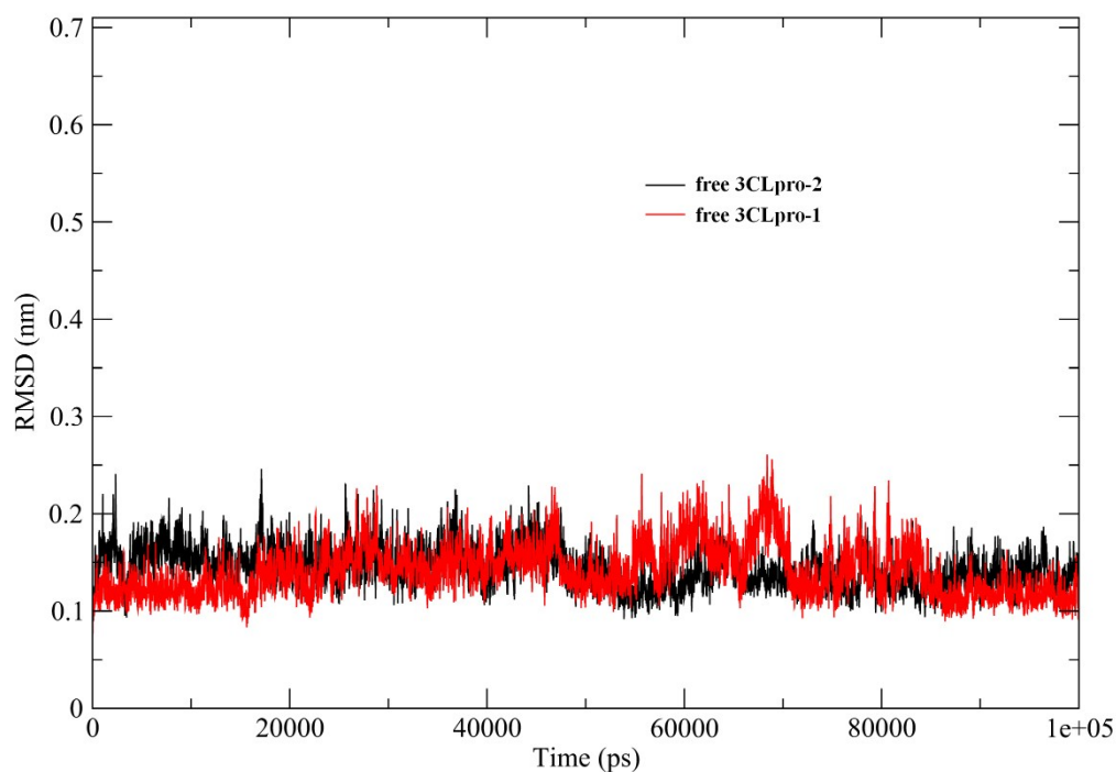
Fig. S2. Time evolution of backbone RMSD values of SARS HCoV 3CLpro with respect to the starting structure during the free enzyme MD simulations.
