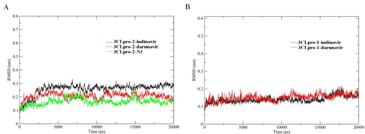
Fig. S1. Time evolution of backbone RMSD values of SARS HCoV 3CLpro with respect to the starting structure during the enzyme-inhibitor complex MD simulations. (A) 3CLpro-2-inhibitors; (B) 3CLpro-1-inhibitors.
