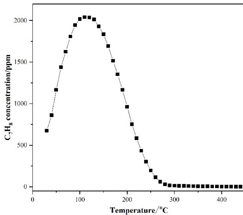
Fig. S4. Desorption curves of AC-800
