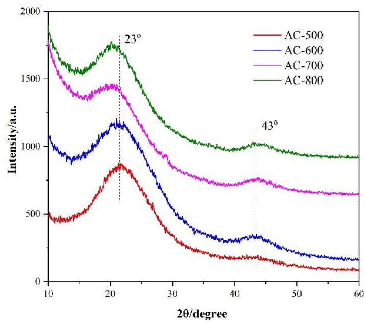
Fig. S5. XRD patterns of activated carbon
