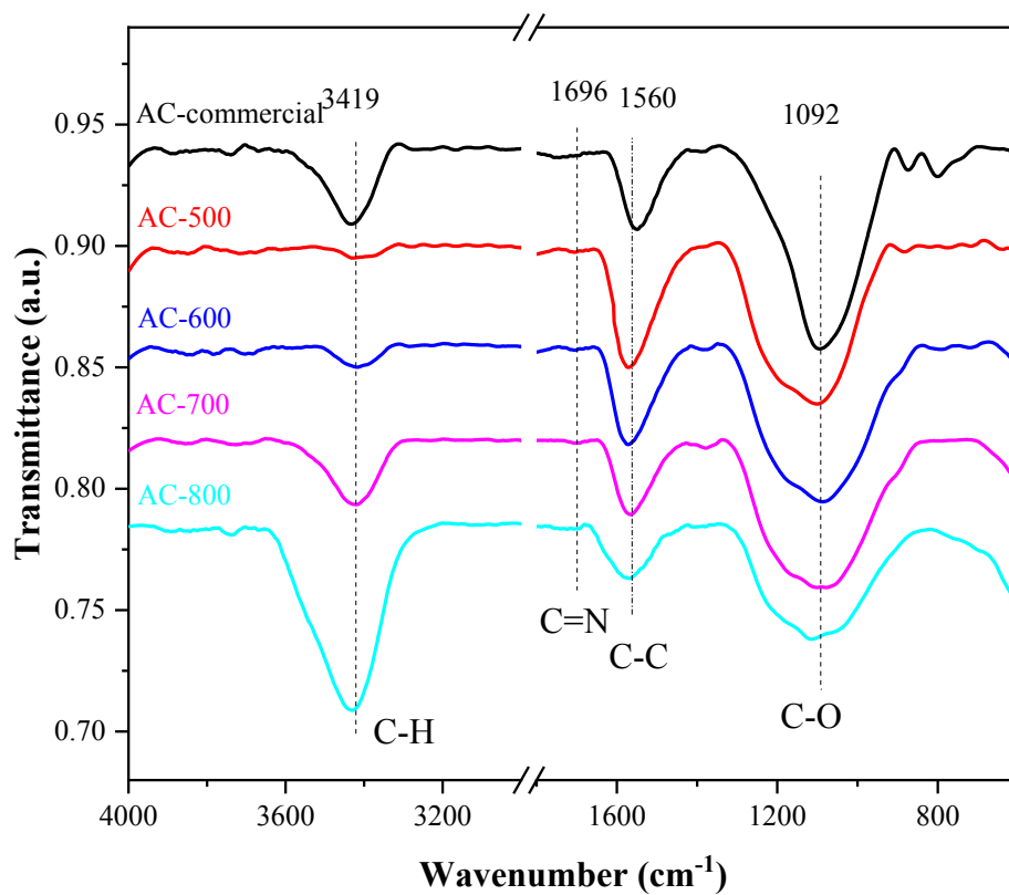
Fig. S3 FTIR spectra of the as-prepared ACs.
