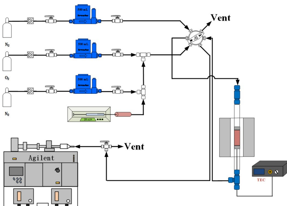
Fig. S1 Scheme of the experimental setup
