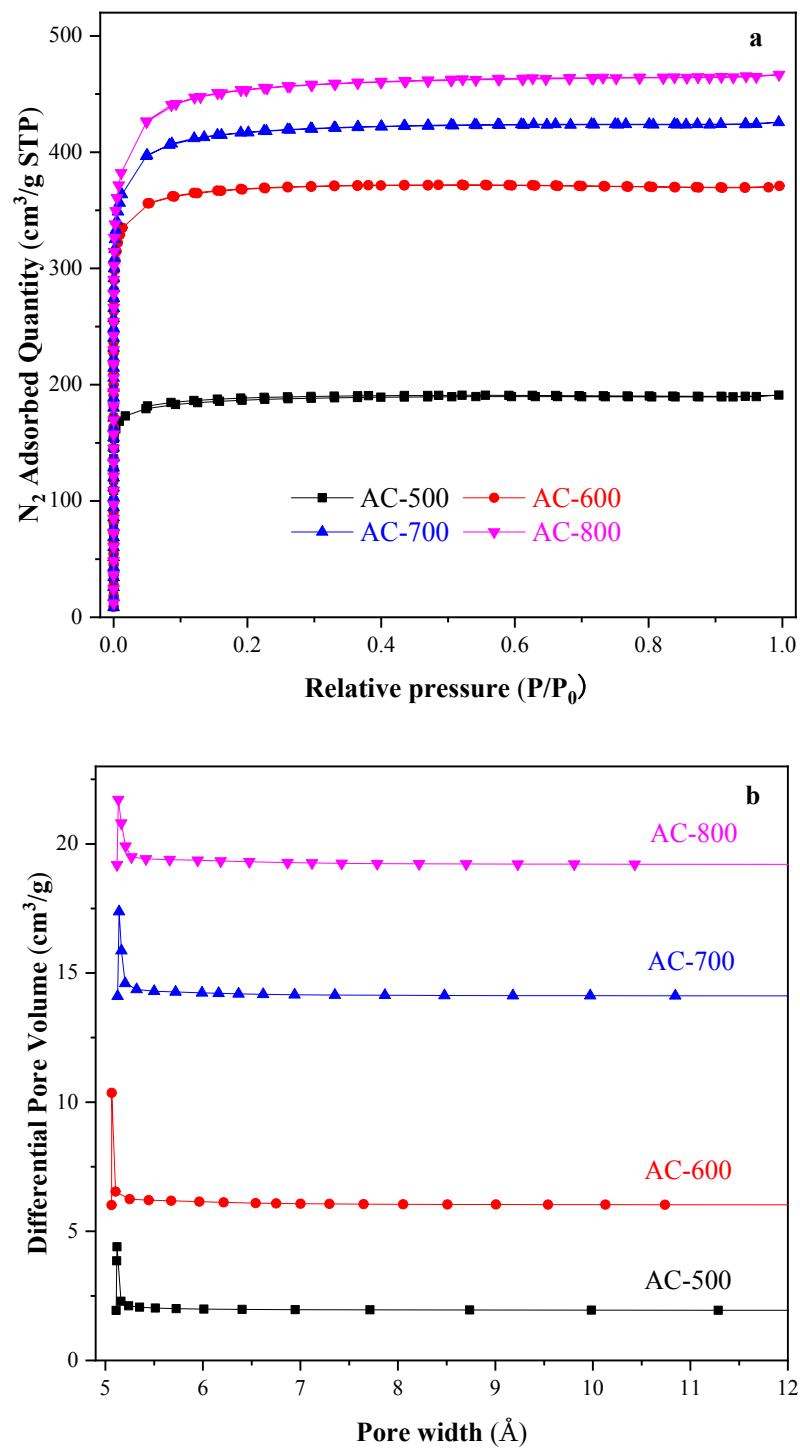
Fig. S2. N 2 adsorption/desorption isotherms (a) and pore size distributions (b) of ACs
