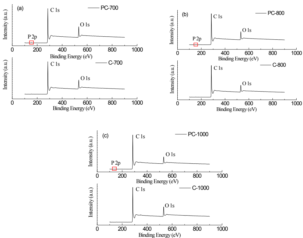
Fig. S1. XPS spectrum of a) C-700 and PC-700, b) C-800 and PC-800, c) C-1000 and PC-1000.
