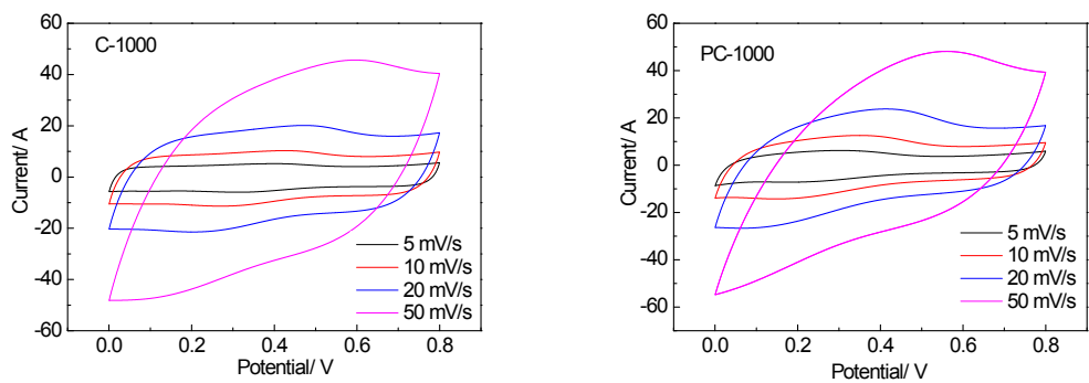
Fig. S2. CV curves of C-700, PC-700, C-800, PC-800, C-1000 and PC-1000.
