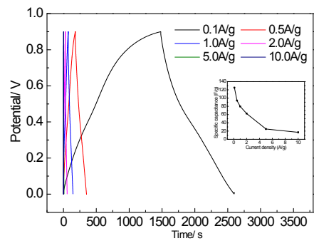
Fig. S4. GCD curves of PC-900 measured on two-electrode system under different current densities. Inset is the specific capacitances of PC-900 at different current densities.
