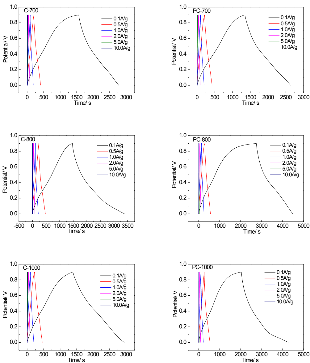
Fig. S3. GCD curves of C-700, PC-700, C-800, PC-800, C-1000 and PC-1000.
