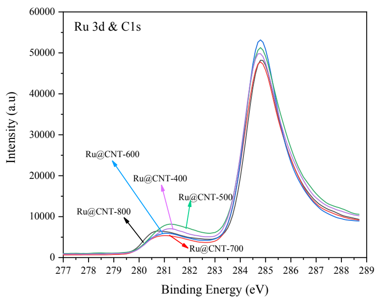
Fig.S3 Ru 3d spectra of all Ru@CNT samples.
