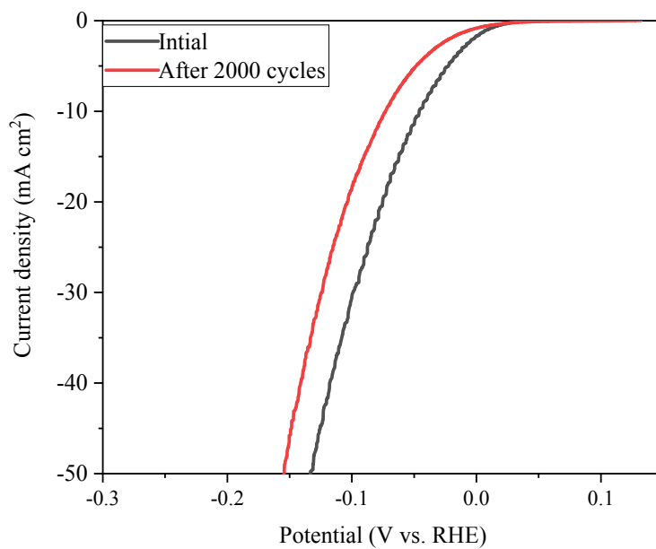
Fig.S4 HER polarization curves recorded before and after 2000 potential cycles.
