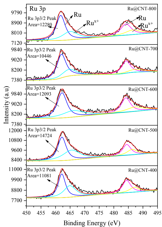
Fig.S2 Ru 3p spectra of all Ru@CNT samples.
