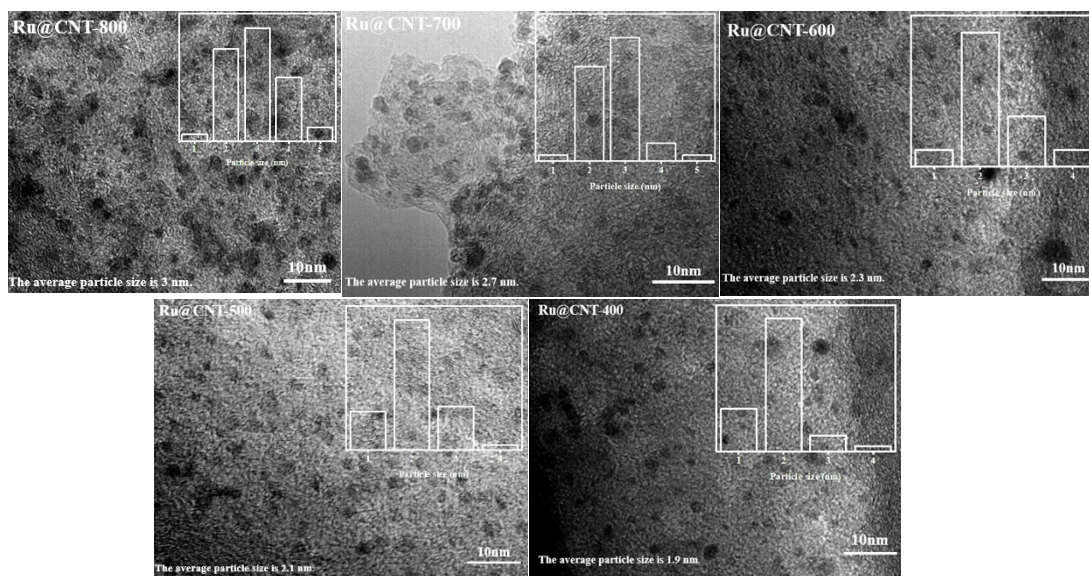
Fig.S1 TEM images of all Ru@CNT samples.
