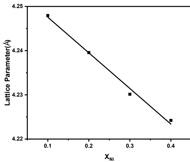
Figure S1 : Variation of the lattice parameter of Ni x Co 1-x O with Ni content
