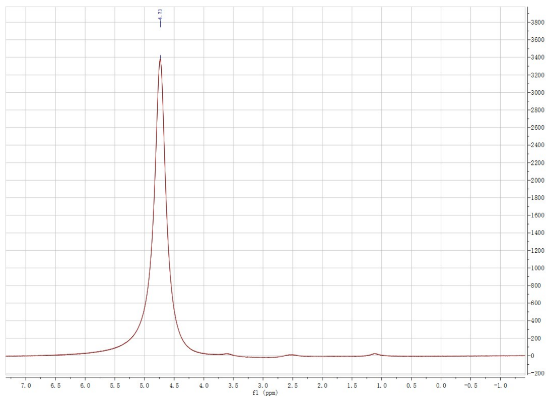
Fig.S3 ^1\text{H} NMR spectra of CP-1-Fe
