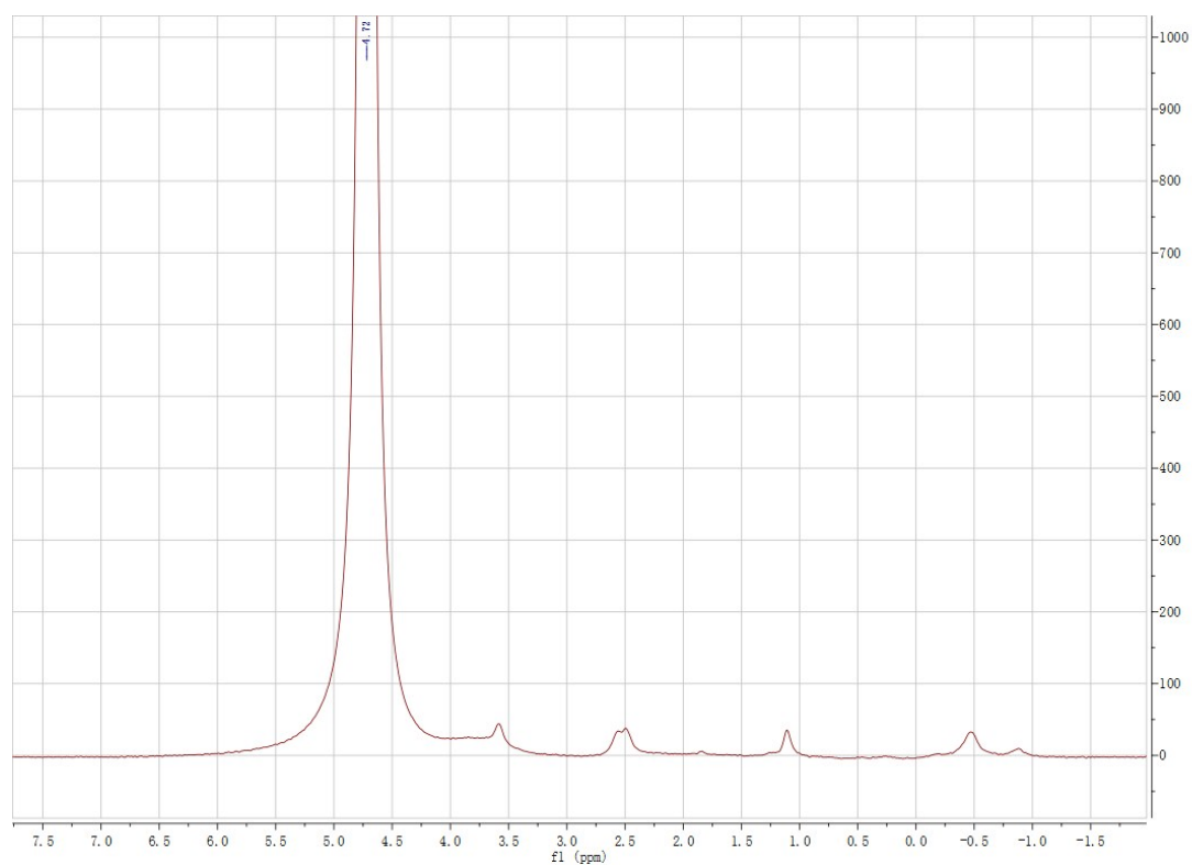
Fig.S4 ^1\text{H} NMR spectra of CP-3-Fe
