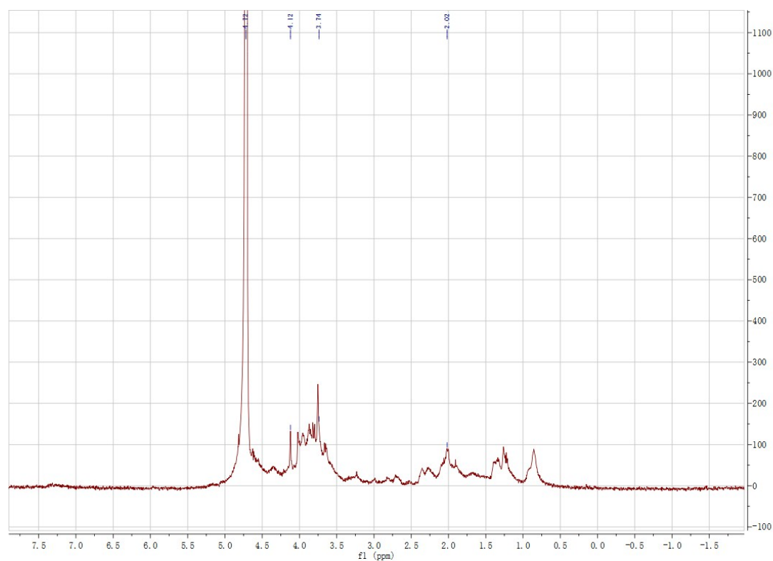
Fig.S2 ^1\text{H} NMR spectra of CP-3
