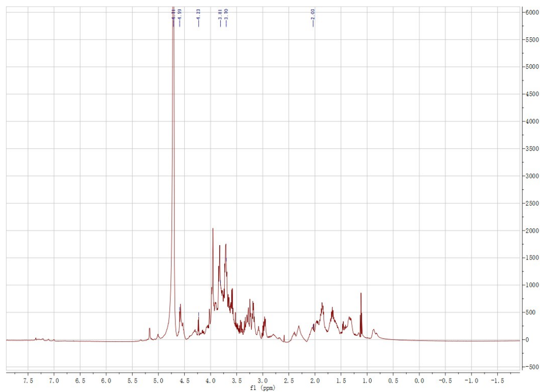
Fig.S1 ^1\text{H} NMR spectra of CP-1
