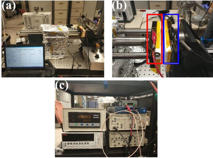
Figure S1. Photograph of (a) our experimental setup, (b) force loading platform, and (c) power supply system.
