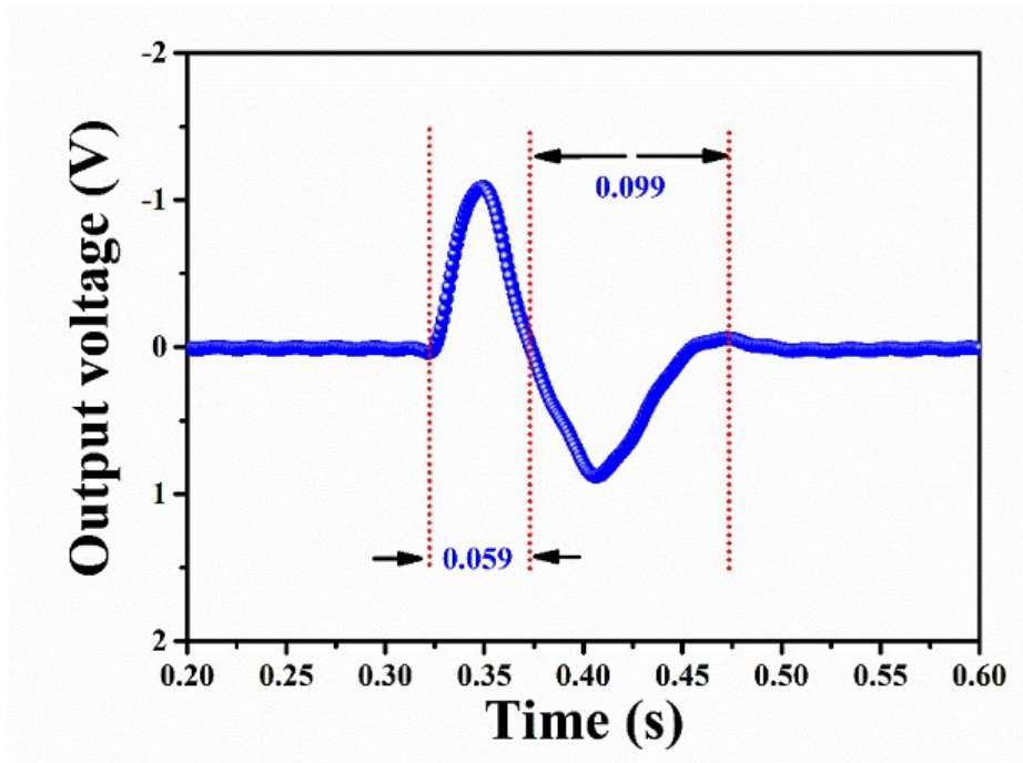
Figure S2. Response time and recovery time of the devices.
