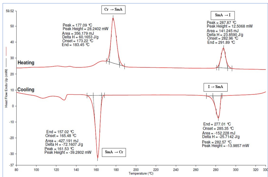
Figure ESI2. DSC thermogram of compound 5b
