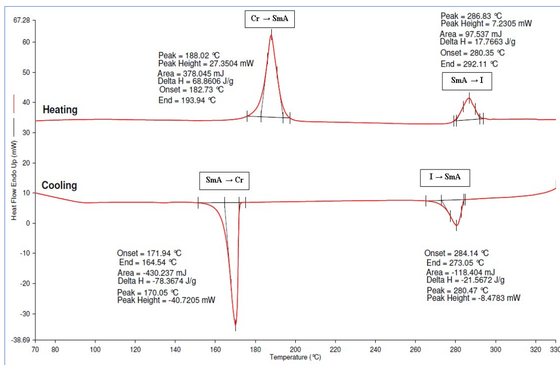
Figure ESI1. DSC thermogram of compound 5a
