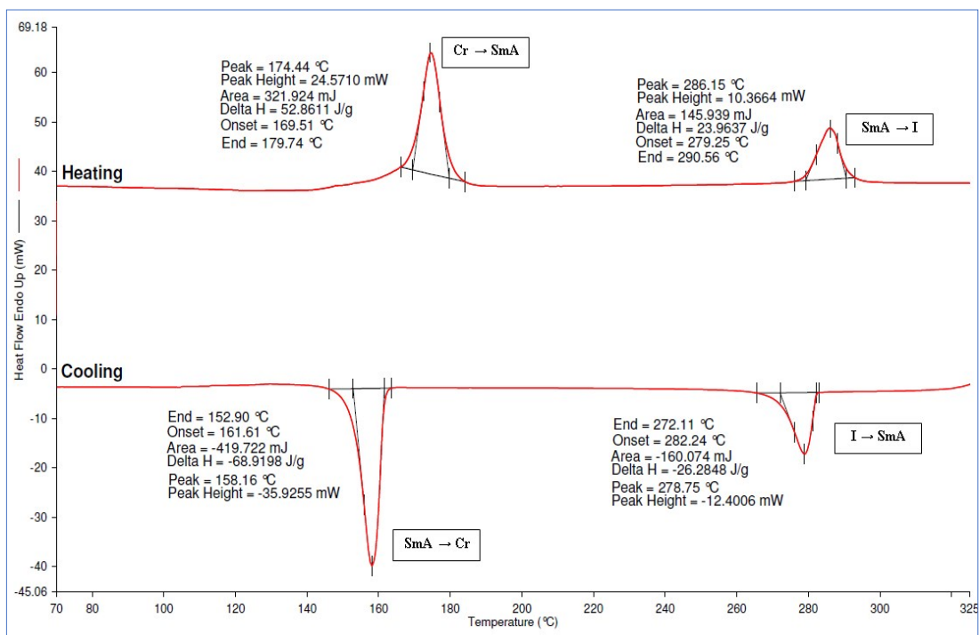
Figure ESI3. DSC thermogram of compound 5c
