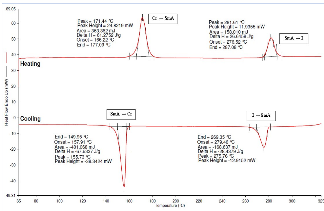
Figure ESI4. DSC thermogram of compound 5d
