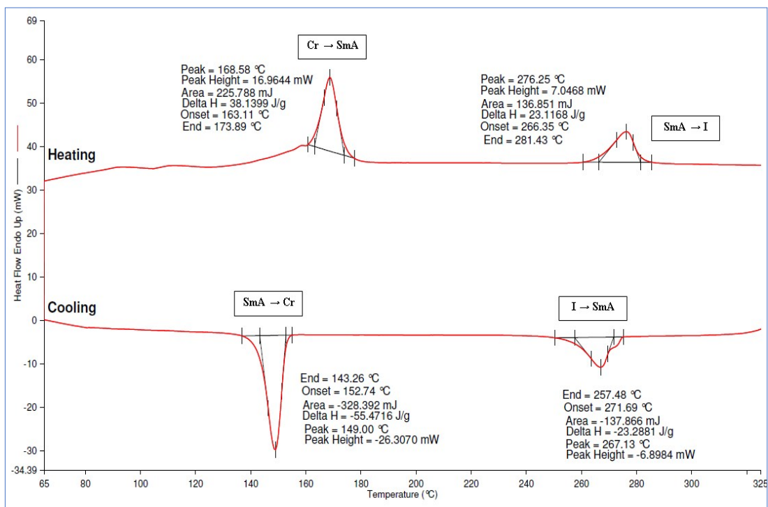
Figure ES15. DSC thermogram of compound 5e
