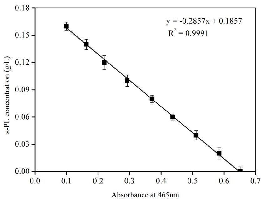
Supplementary Fig. 2 The standard curve of \epsilon -PL using methyl orange method
