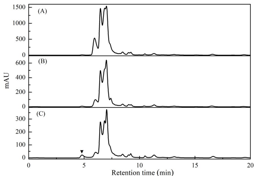
Supplementary Fig. 1 HPLC chromatograms of \epsilon -PL analysis for the bottom phase during the ethanol/ammonium sulfate ATPS extraction. (a) first APTS extraction, (b) second APTS extraction, (c) third APTS extraction. Triangle indicates the \epsilon -PL.
