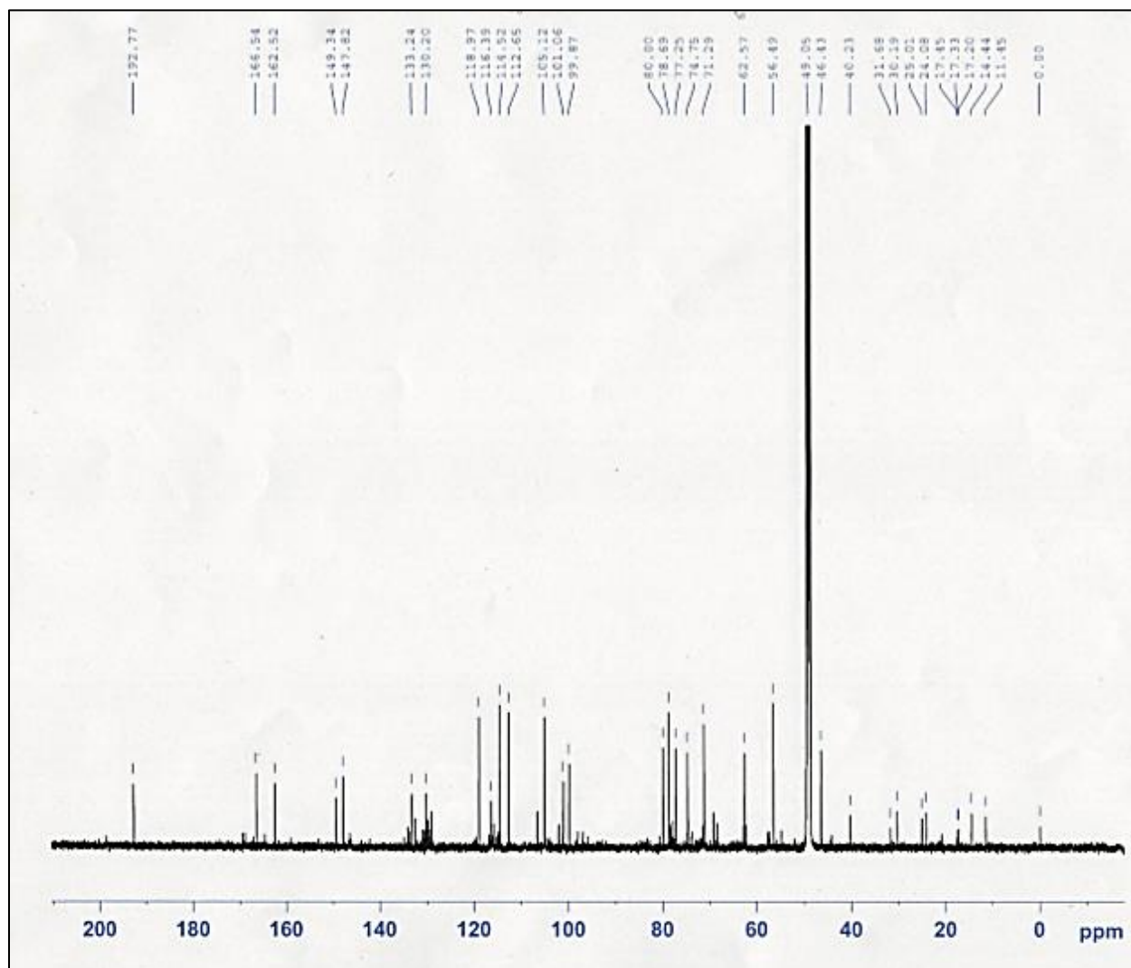
Figure 2S: ^{13}\text{C} -NMR spectrum of compound 1 ( \text{CD}_3\text{OD} , 150 MHz).
