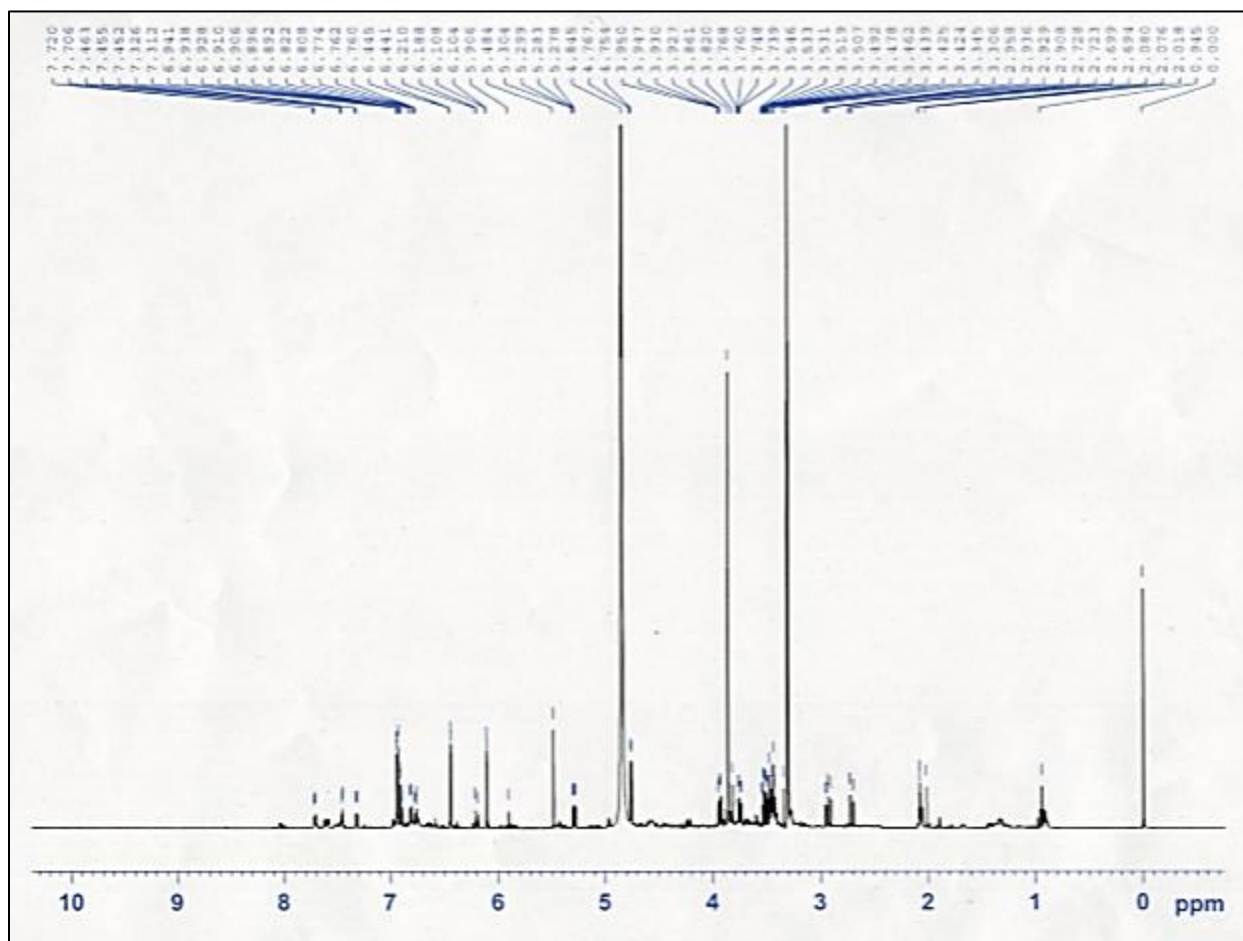
Figure 1S: ^1\text{H} -NMR spectrum of compound 1 ( \text{CD}_3\text{OD} , 600 MHz).
