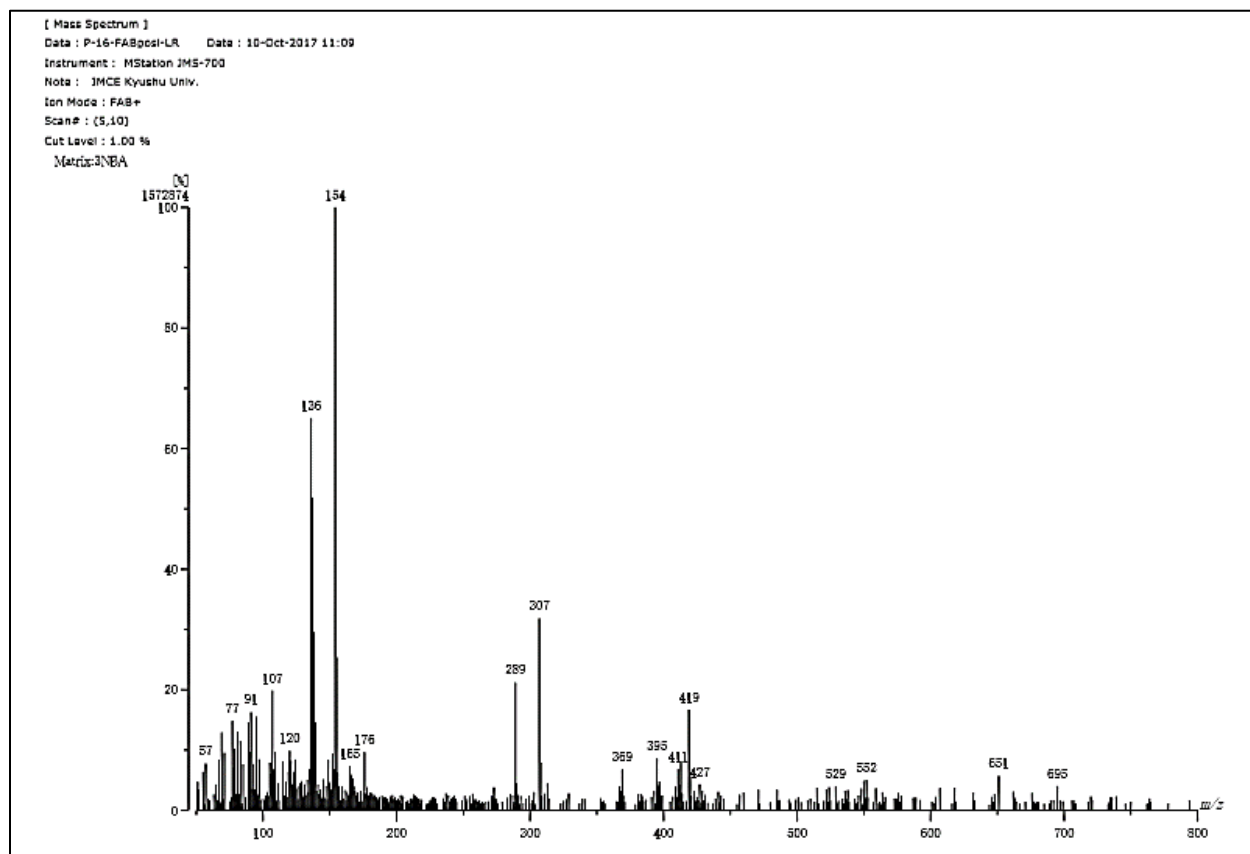
Figure 4S: Positive FAB-MS spectrum of compound 1 .
