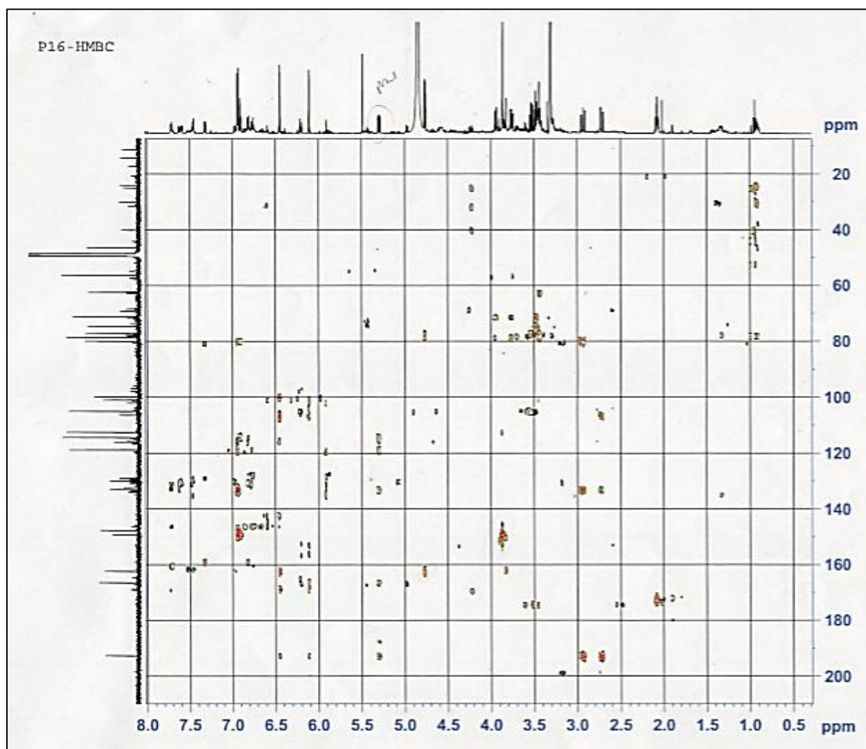
Figure 3S: HMBC spectrum of compound 1 (CD 3 OD).
